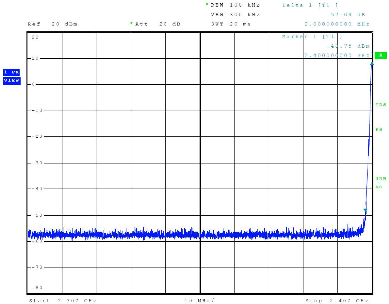
Figure 5 Plot of Transmitter Emissions Low Band Edge Mode 2 BLE
