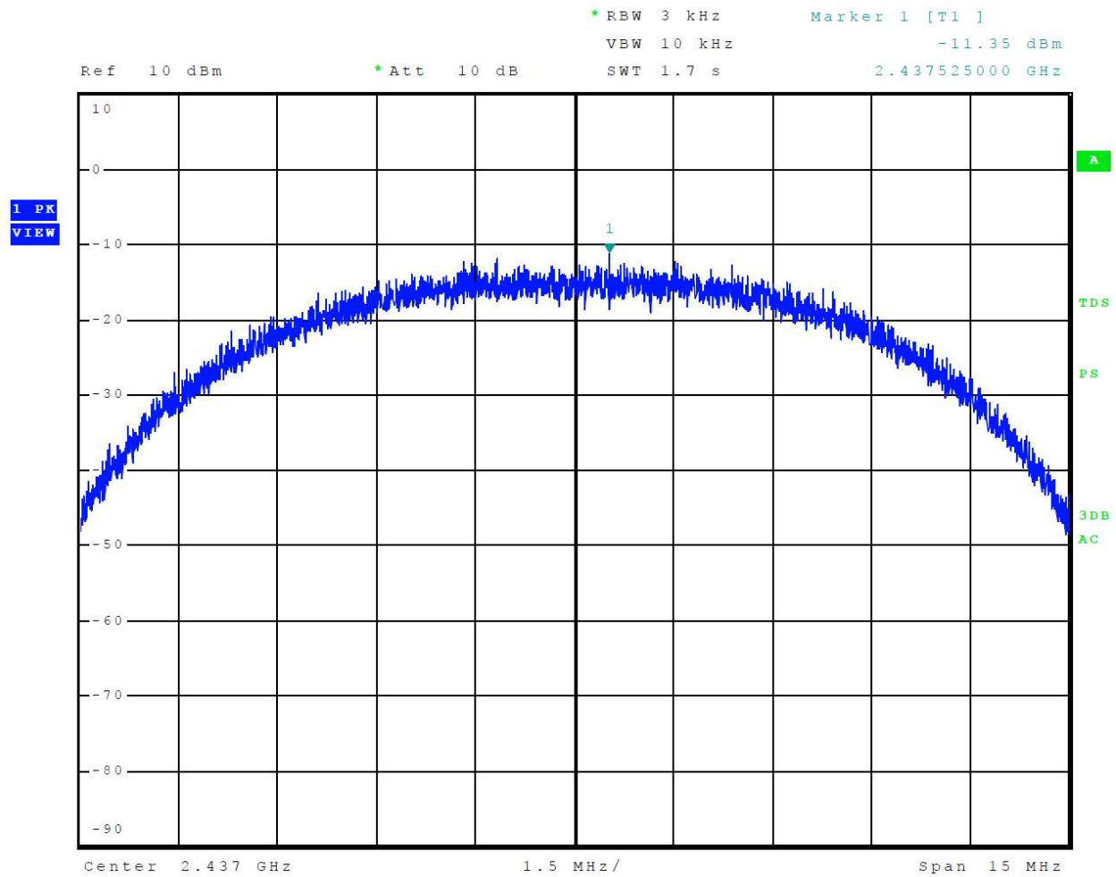
Figure 22 Plot of Transmitter Power Spectral Density Mode 3 802.11b
