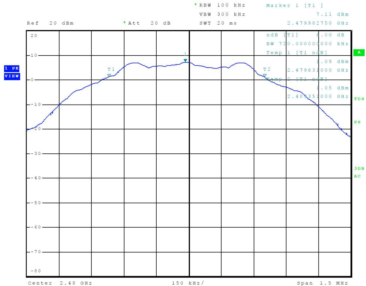
Figure 13 Plot of 6-dB Occupied Bandwidth Mode 2 BLE
