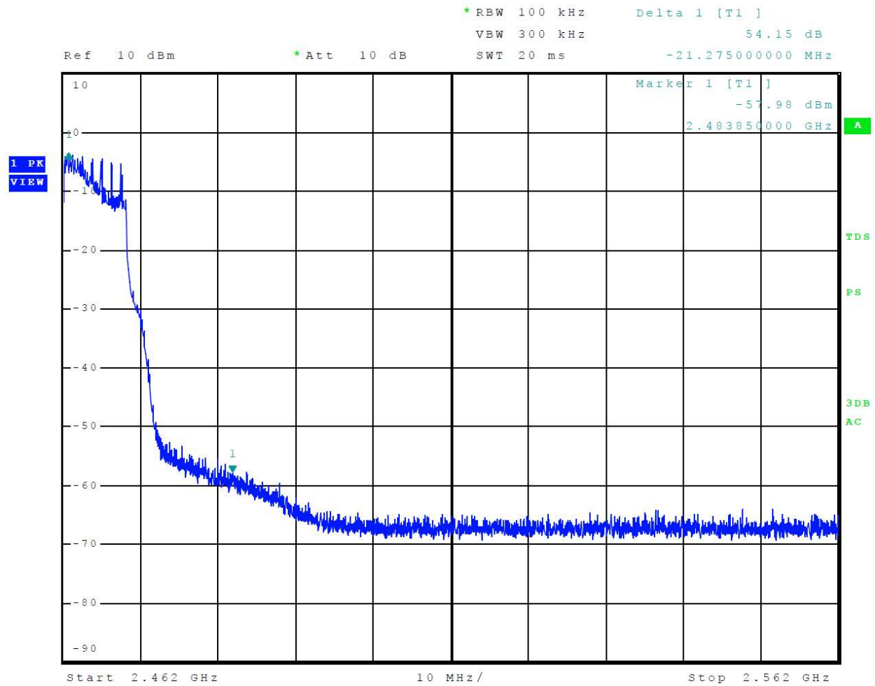
Figure 11 Plot of Transmitter Emissions High Band Edge Mode 4 802.11g
