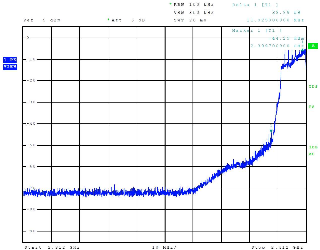
Figure 8 Plot of Transmitter Emissions Low Band Edge Mode 5 802.11n
