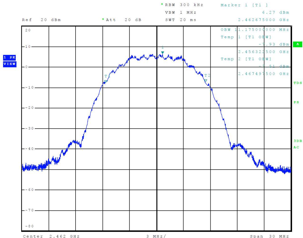
Figure 16 Plot of 99% Occupied Bandwidth Mode 3 802.11b
