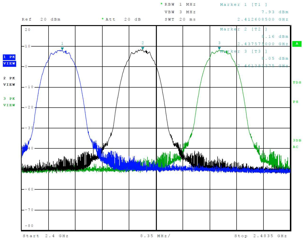
Figure 2 Plot of Transmitter Operation in 2412-2462 MHz Mode 3 802.11b
