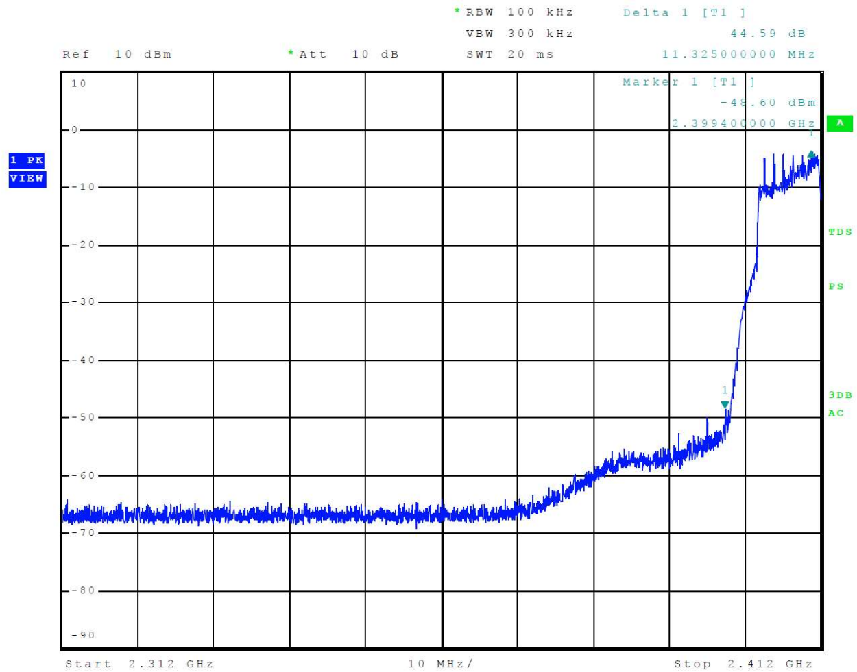
Figure 7 Plot of Transmitter Emissions Low Band Edge Mode 4 802.11g
