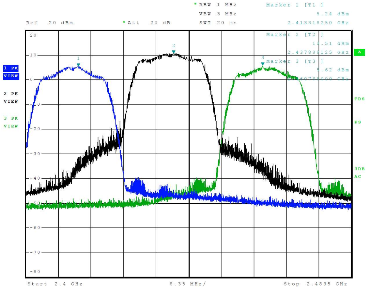
Figure 4 Plot of Transmitter Operation in 2412-2462 MHz Mode 5 802.11n
