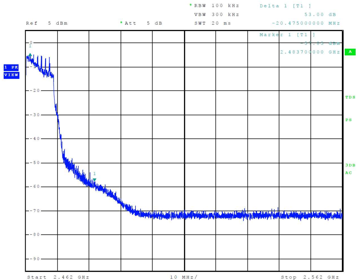
Figure12 Plot of Transmitter Emissions High Band Edge Mode 5 802.11n
