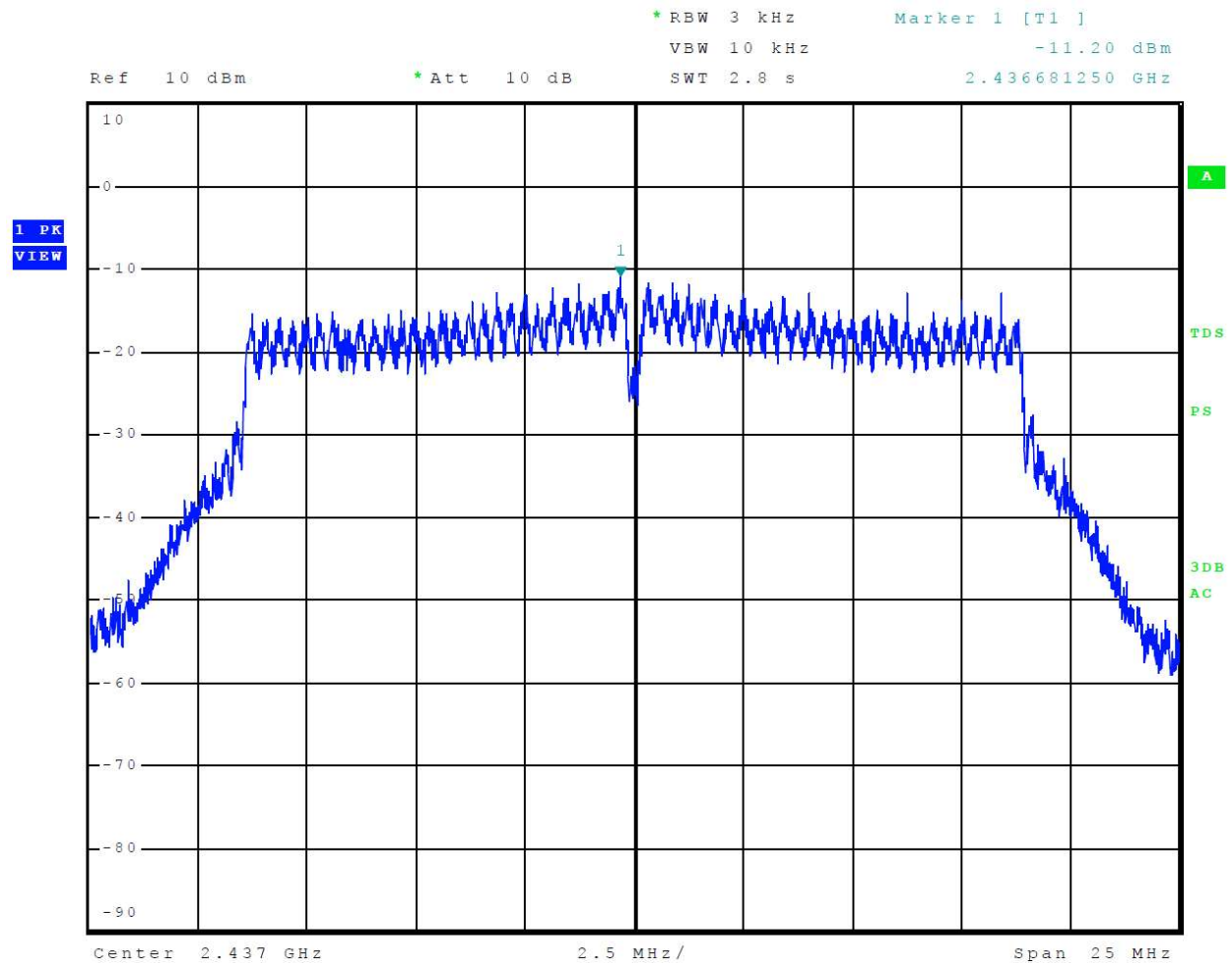
Figure 24 Plot of Transmitter Power Spectral Density Mode 5 802.11n
