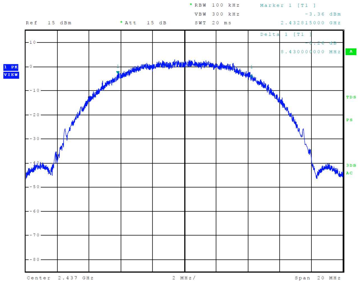
Figure 15 Plot of 6-dB Occupied Bandwidth Mode 3 802.11b
