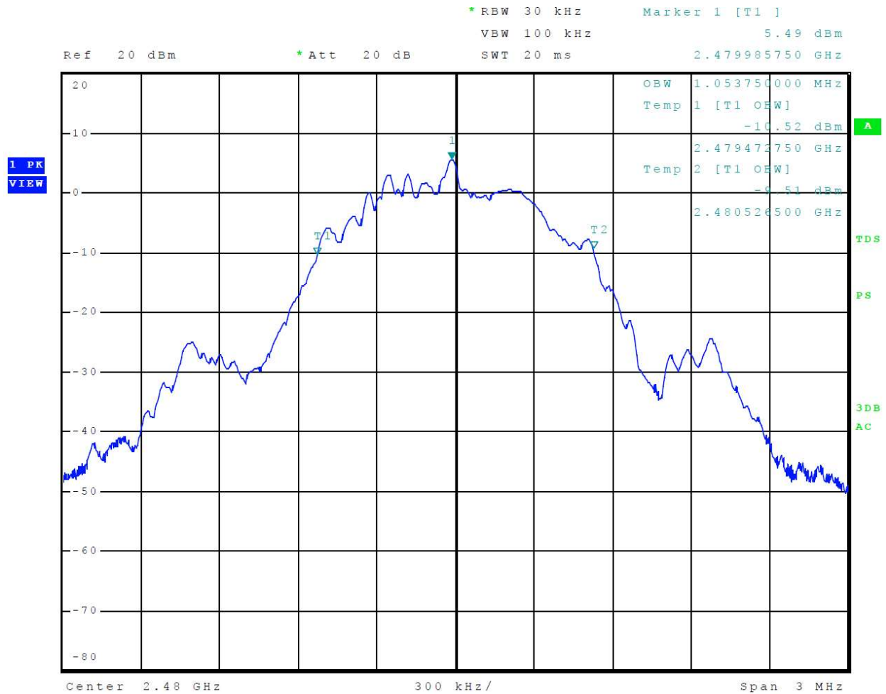
Figure 14 Plot of 99% Occupied Bandwidth Mode 2 BLE
