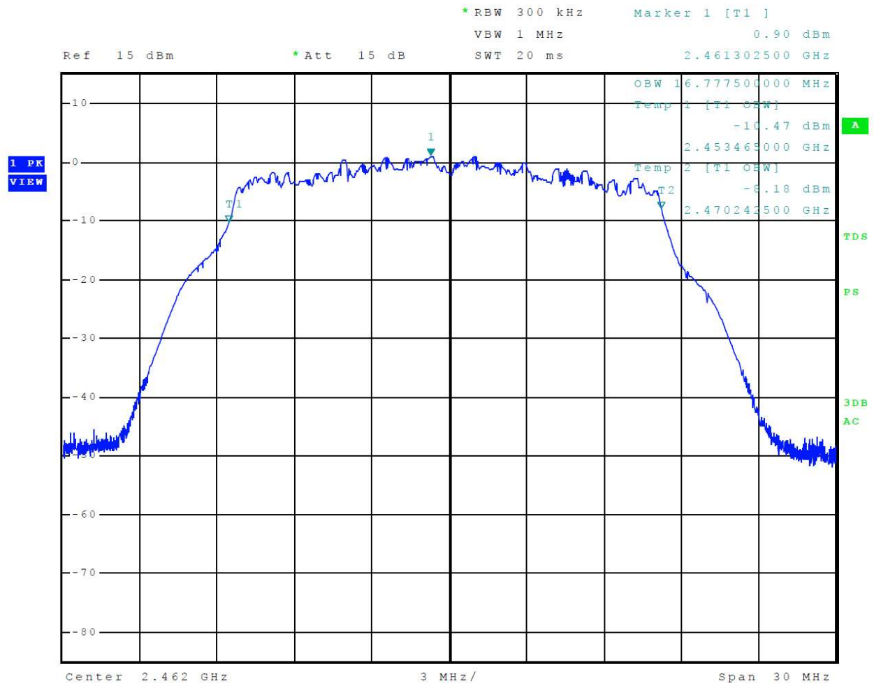
Figure 18 Plot of 99% Occupied Bandwidth Mode 4 802.11g
