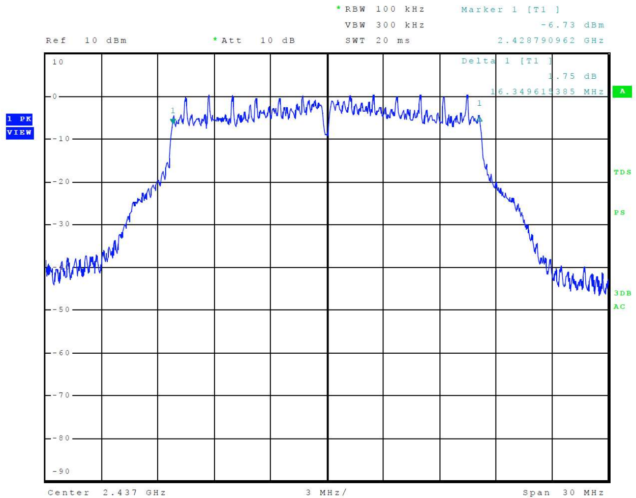
Figure 17 Plot of 6-dB Occupied Bandwidth Mode 4 802.11g
