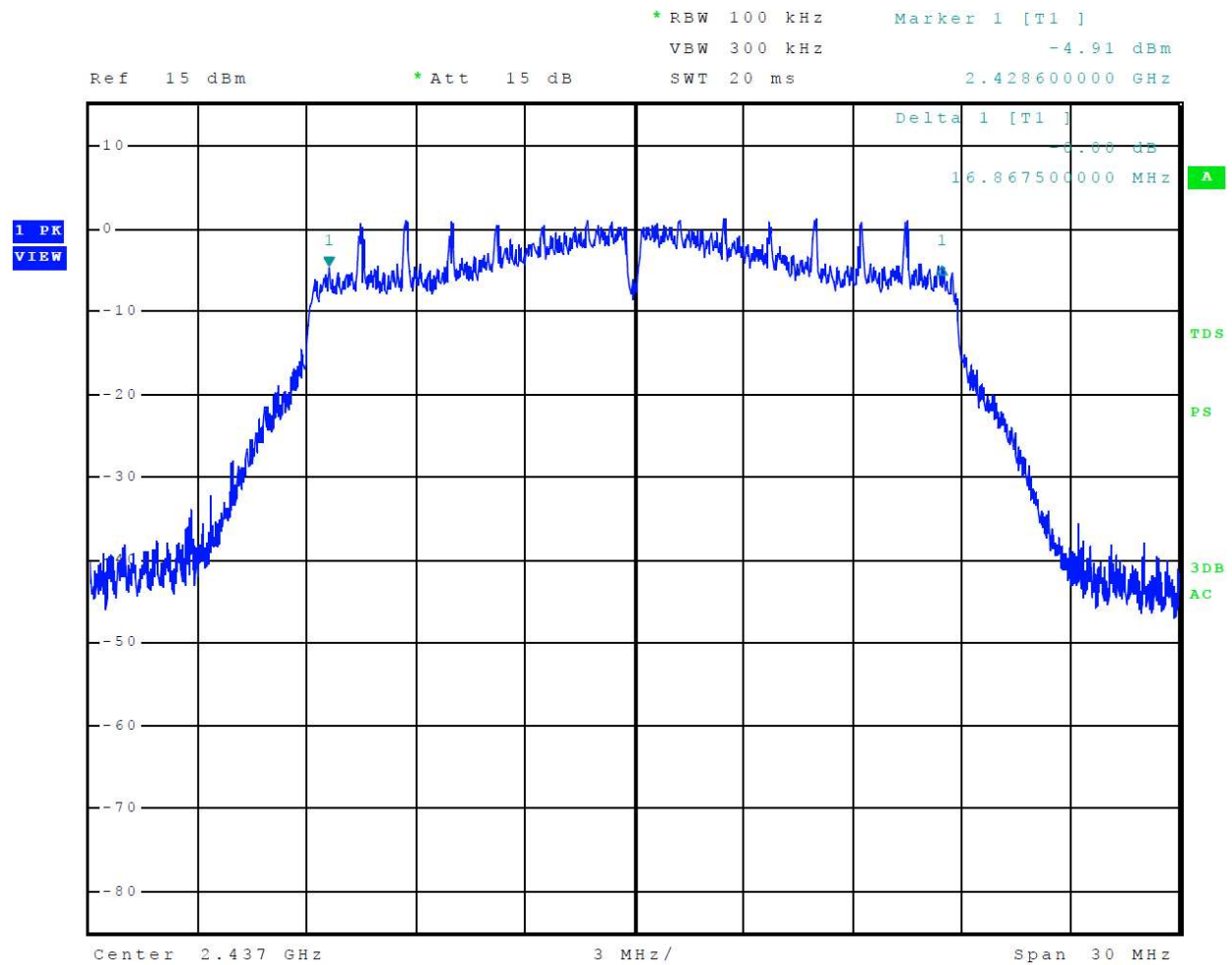
Figure 19 Plot of 6-dB Occupied Bandwidth Mode 5 802.11n
