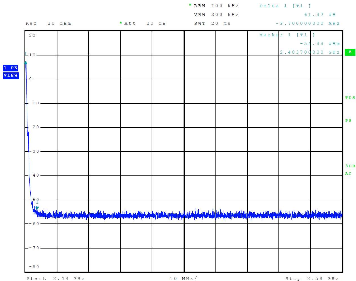
Figure 9 Plot of Transmitter Emissions High Band Edge Mode 2 BLE
