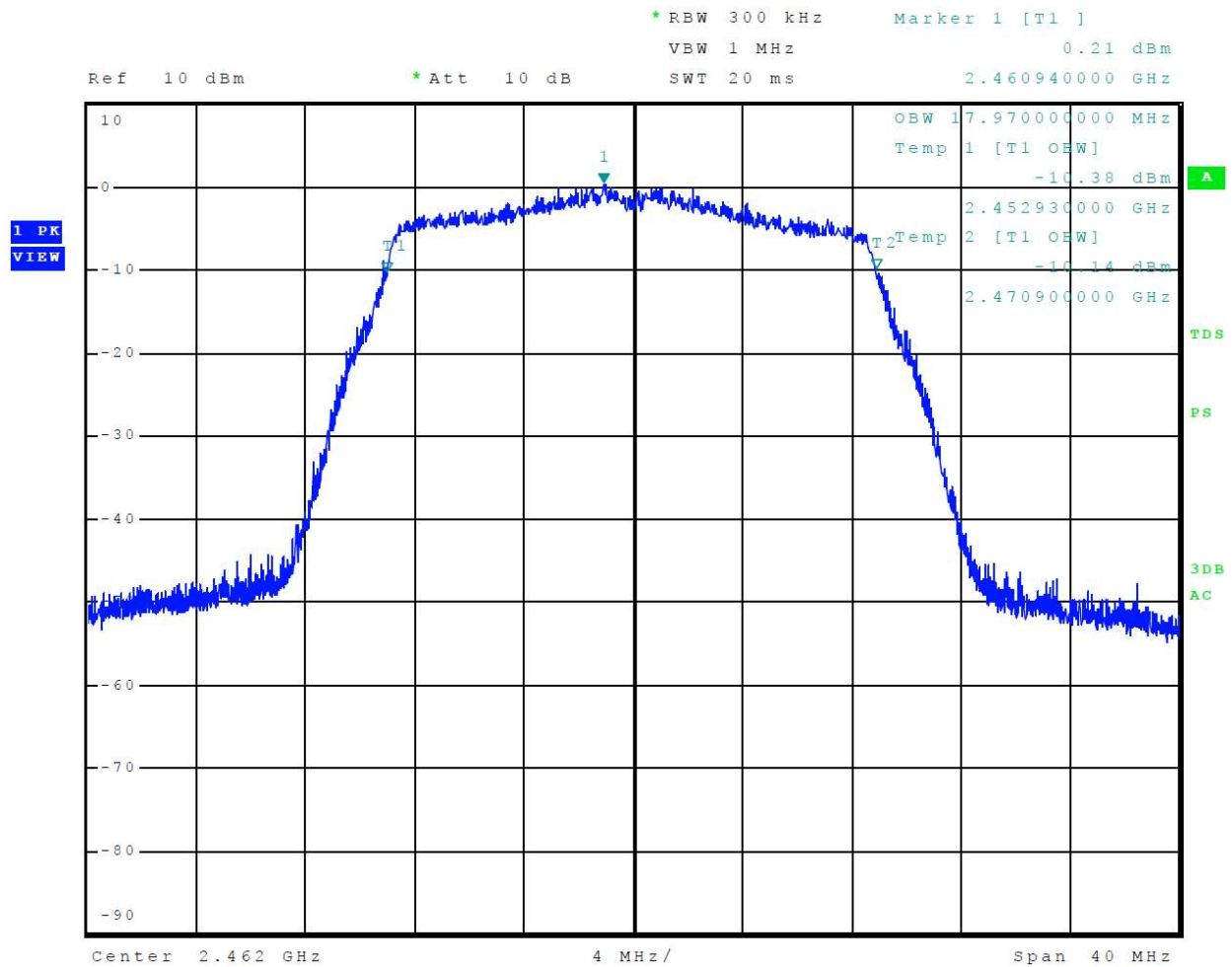
Figure 20 Plot of 99% Occupied Bandwidth Mode 5 802.11n
