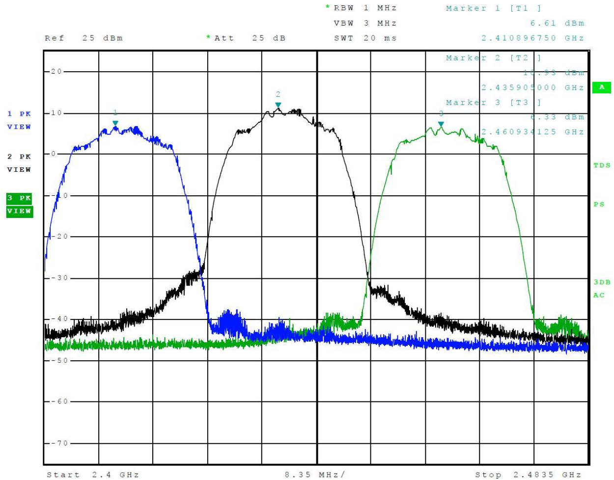
Figure 3 Plot of Transmitter Operation in 2412-2462 MHz Mode 4 802.11g
