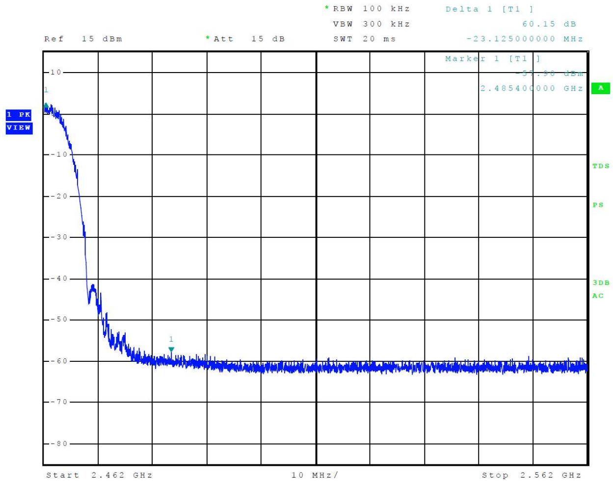
Figure 10 Plot of Transmitter Emissions High Band Edge Mode 3 802.11b
