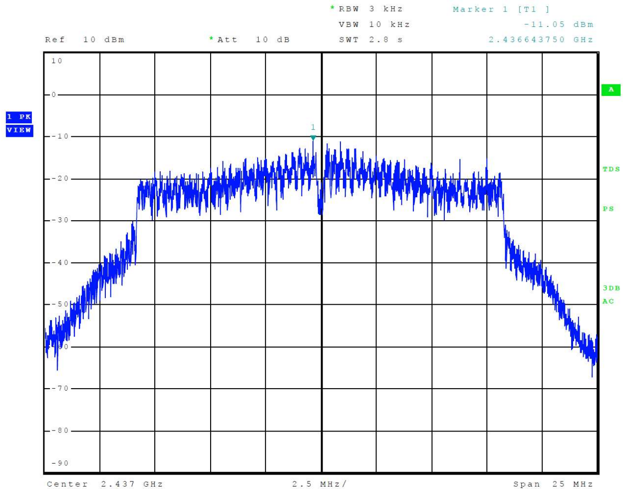
Figure 23 Plot of Transmitter Power Spectral Density Mode 4 802.11g
