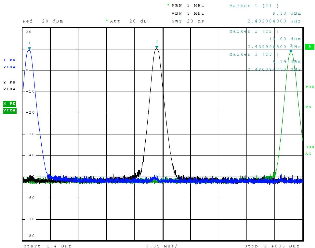
Figure 1 Plot of Transmitter Operation in 2402-2480 MHz Mode 2 BLE
