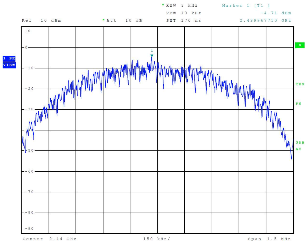
Figure 21 Plot of Transmitter Power Spectral Density Mode 2 BLE
