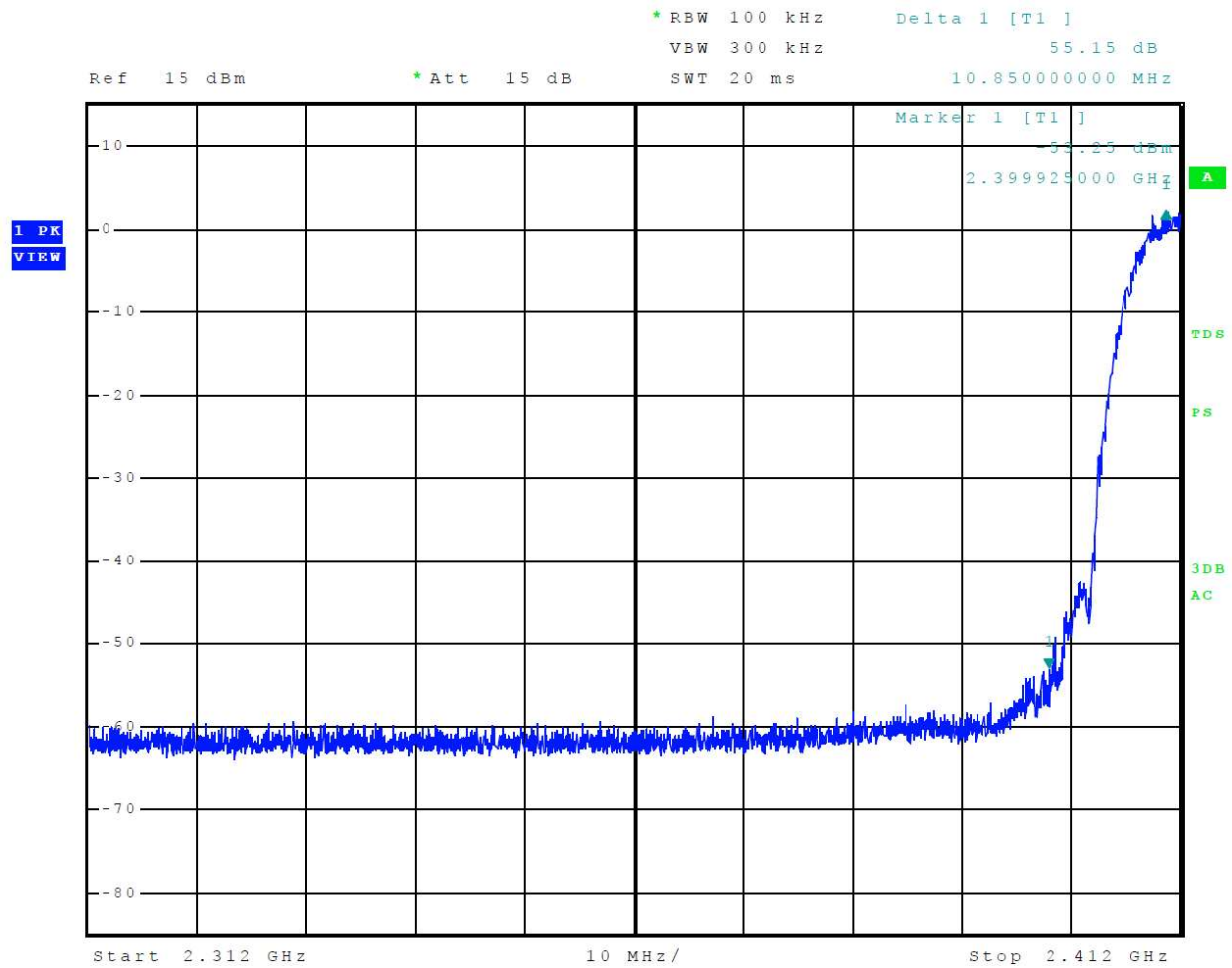
Figure 6 Plot of Transmitter Emissions Low Band Edge Mode 3 802.11b
