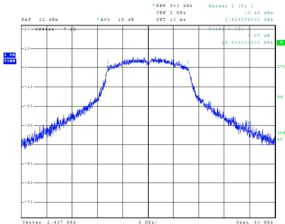
Figure 11 Plot of Transmitter 6-dB Occupied Bandwidth (802.11 g-mode)
