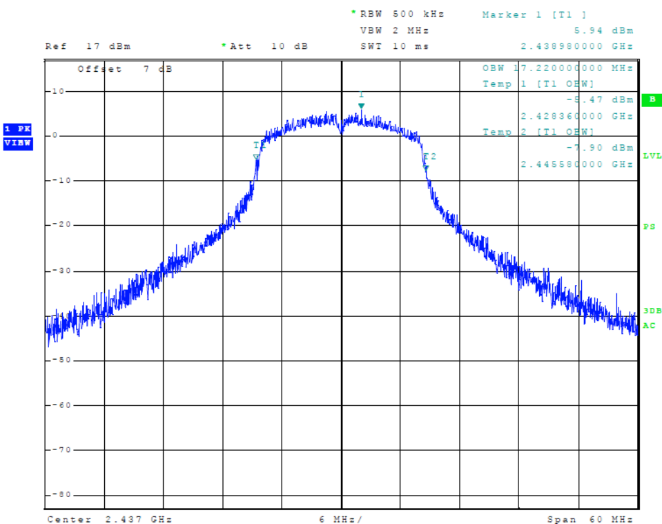
Figure 14 Plot of Transmitter 99% Occupied Bandwidth (802.11 g-mode)
