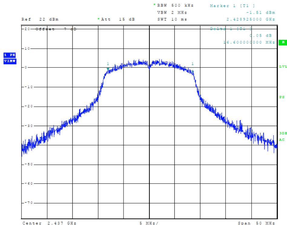
Figure 12 Plot of Transmitter 6-dB Occupied Bandwidth (802.11 n-mode)
