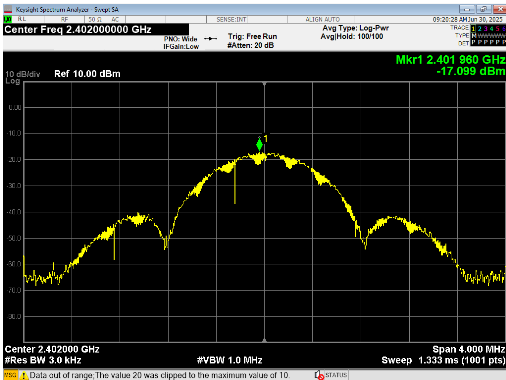
11 PSD, ANT GFSK, 2402MHz
