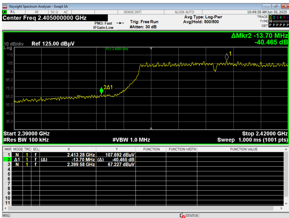
46 LBE Unrestricted, WiFi G 54MB, 2412MHz
