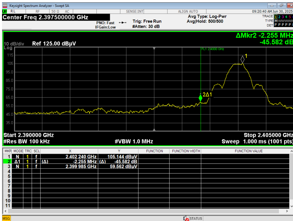
07 LBE Unrestricted, ANT GFSK, 2402MHz
