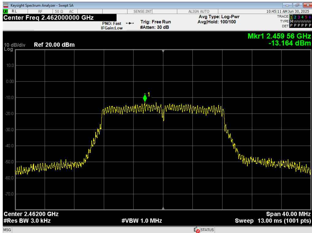
39 PSD, WiFi G 6MB, 2462MHz
