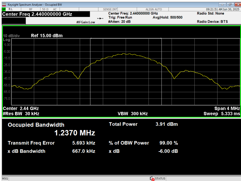
09 Occupied BW, ANT GFSK, 2440MHz
