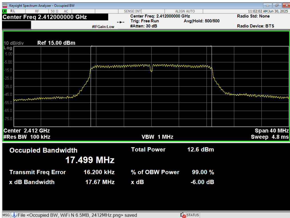
53 6dB BW, WiFi N 6.5MB, 2412MHz
