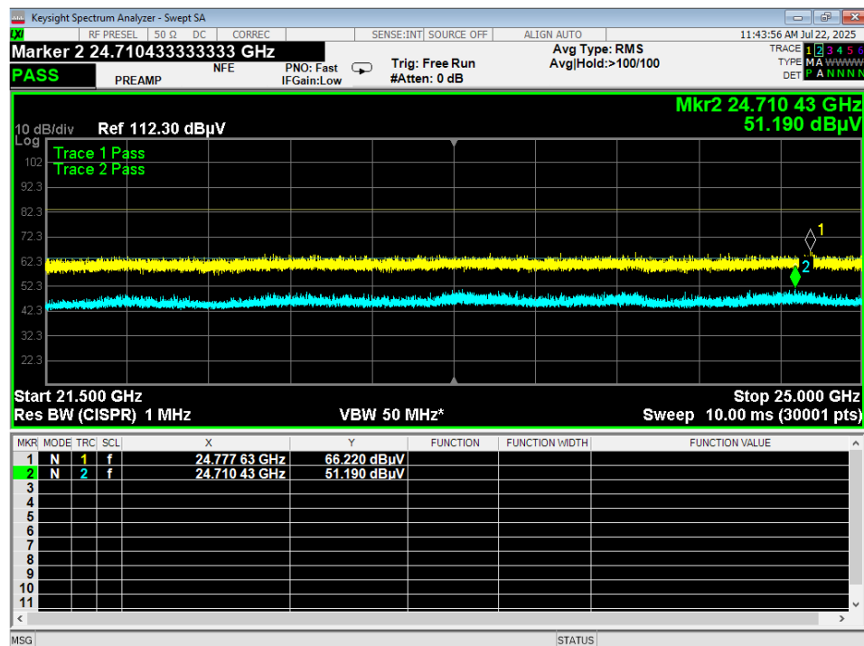
Figure 11 - Radiated Emissions Plot, 21.5-25GHz, BLE 2MB Mid, 1m test distance No emissions were found above lab noise floor, tabular data not provided
