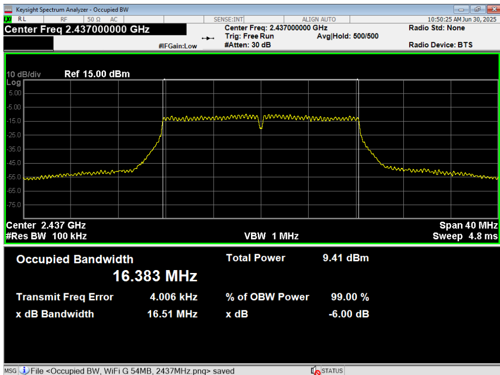
41 6dB BW, WiFi G 54MB, 2437MHz
