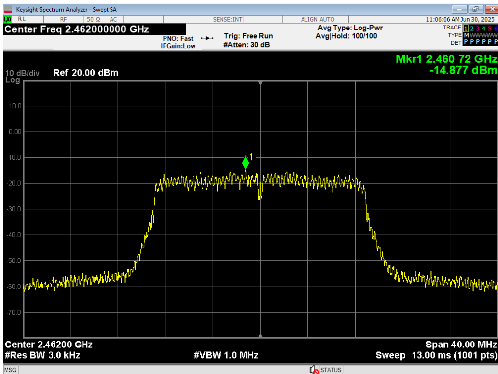
65 PSD, WiFi N 6.5MB, 2462MHz
