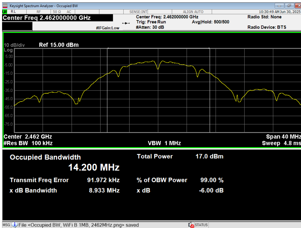
03 6dB BW, WiFi B 1MB, 2462MHz
