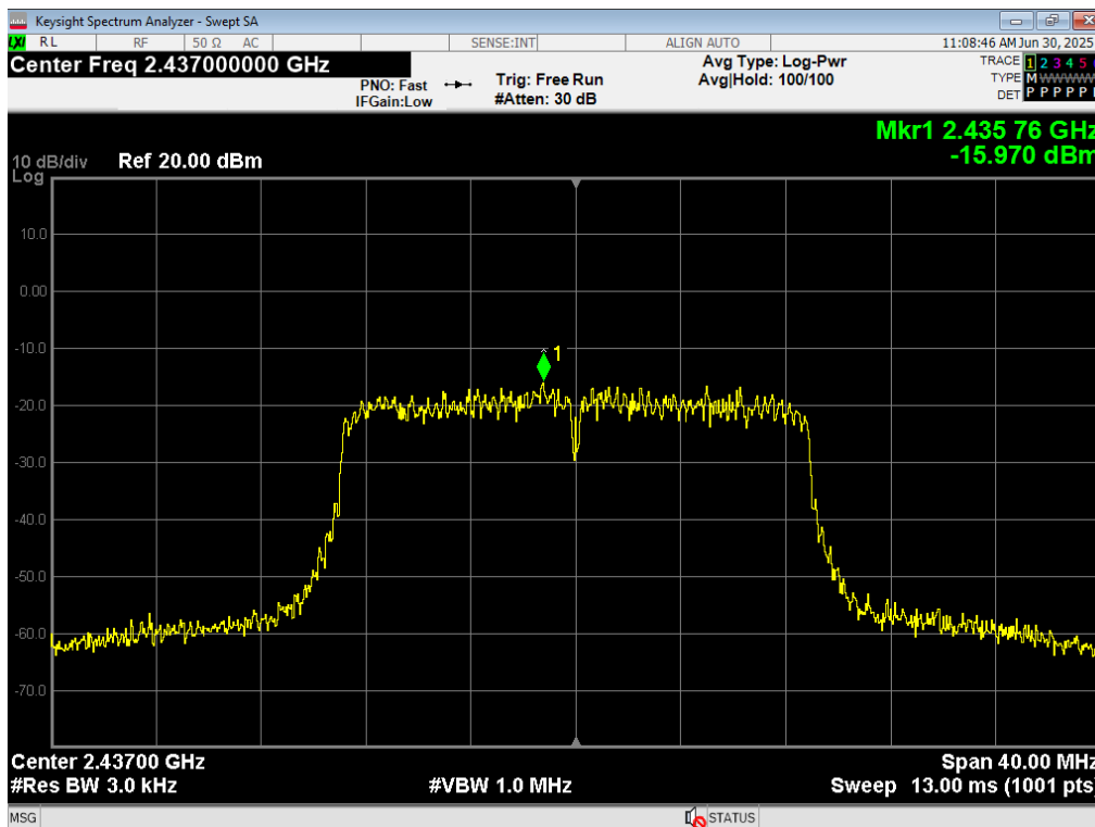
77 PSD, WiFi N 72.2MB, 2437MHz
