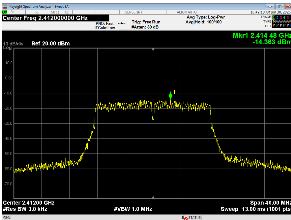
50 PSD, WiFi G 54MB, 2412MHz
