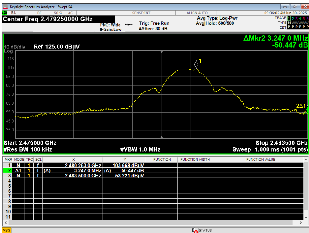
18 HBE Unrestricted, BLE 1MB, 2480MHz
