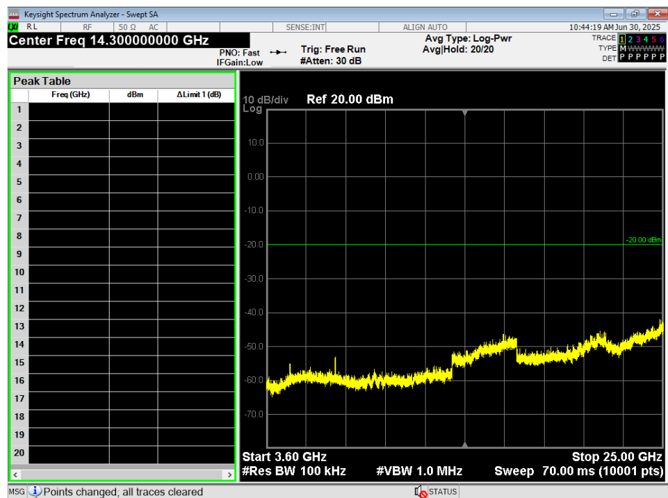
Figure 26 - Conducted Spurious Plot, WIFI 802.11g, 3.6G – 25G, Mid
