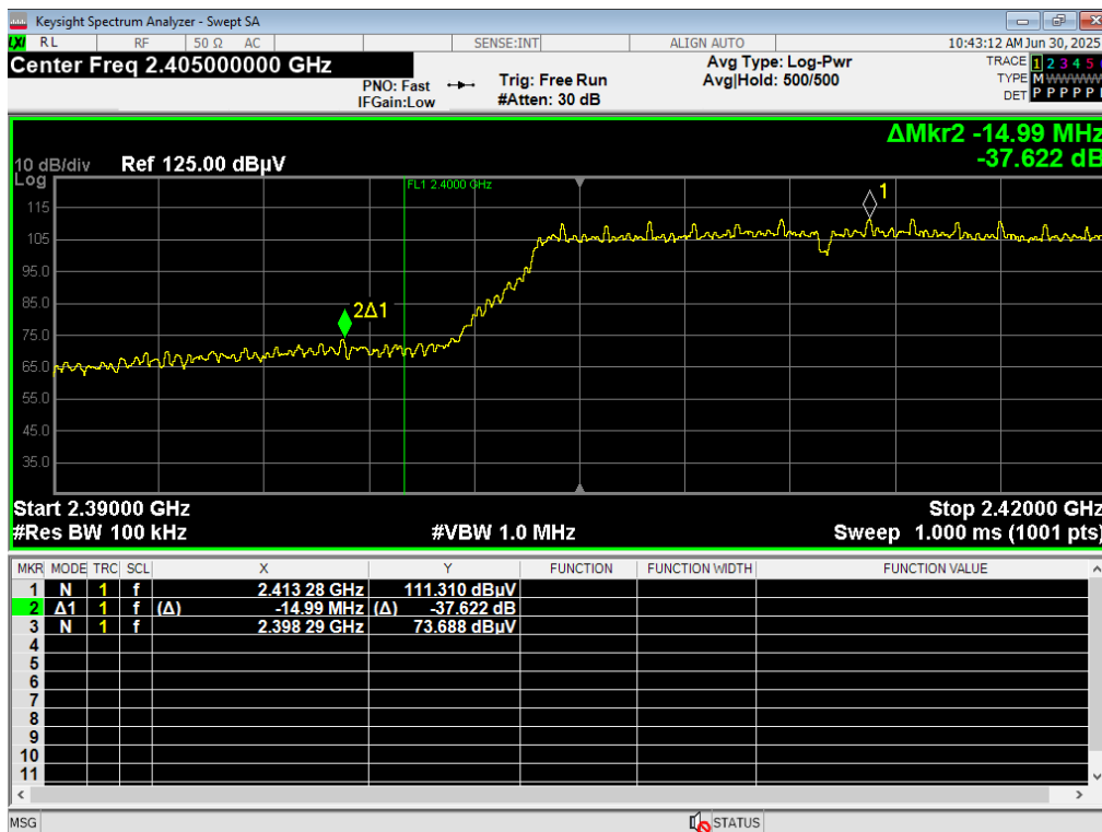
33 LBE Unrestricted, WiFi G 6MB, 2412MHz
