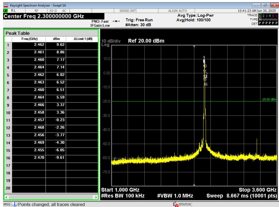
Figure 22 - Conducted Spurious Plot, WIFI 802.11b, 1G – 3.6G, High
