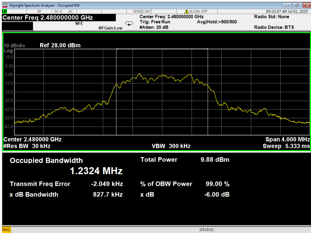
23 Occupied BW, 3EDR, 2480MHz
