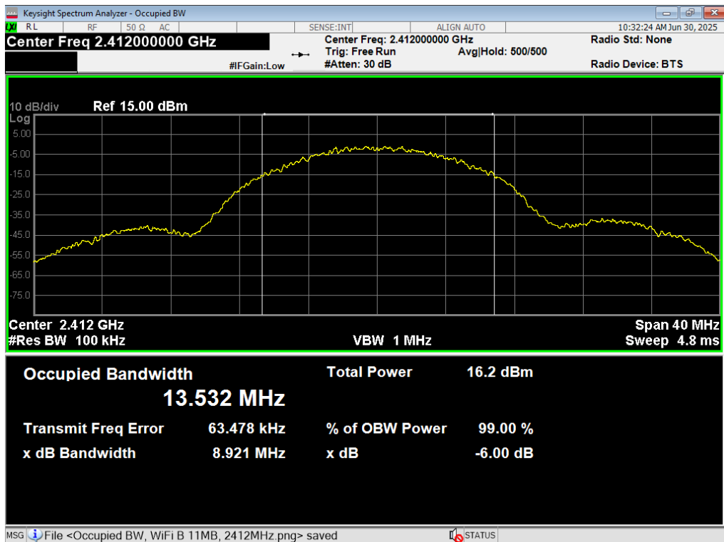
14 6dB BW, WiFi B 11MB, 2412MHz
