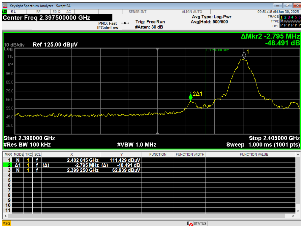
07 LBE Unrestricted, BTBR, 2402MHz
