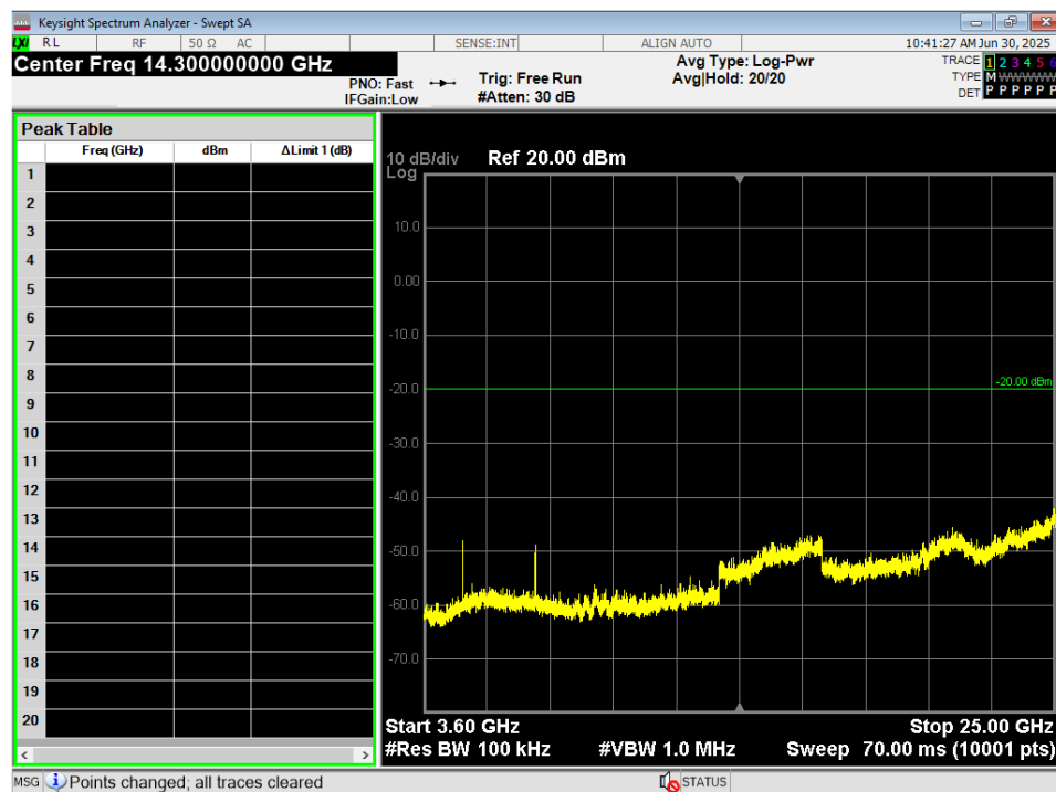
Figure 23 - Conducted Spurious Plot, WIFI 802.11b, 3.6G – 25G, High
