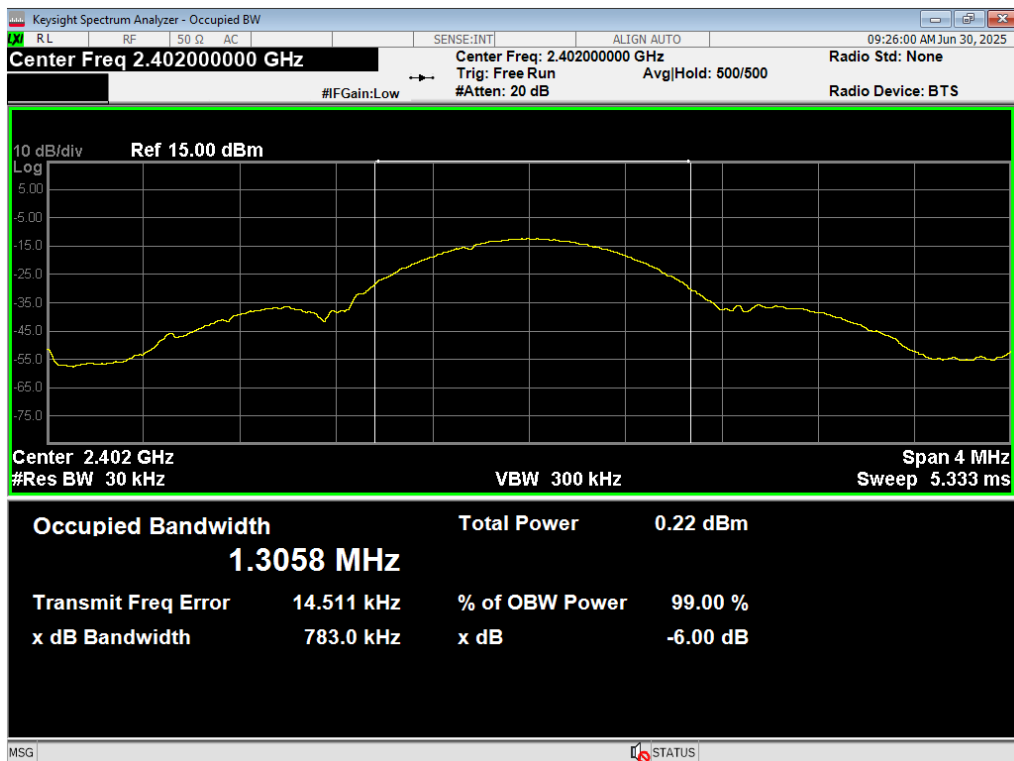
21 Occupied BW, BLE 1MB, 2402MHz
