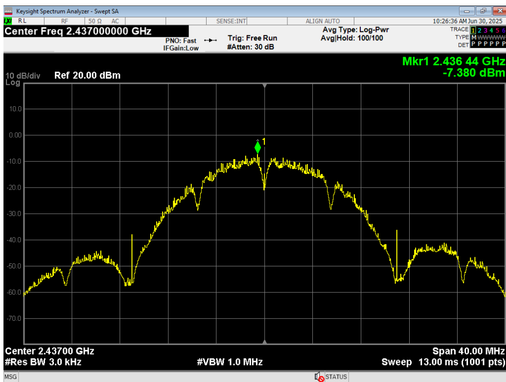
12 PSD, WiFi B 1MB, 2437MHz
