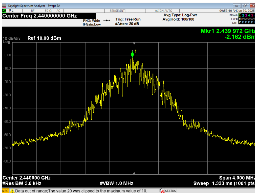
12 PSD, BTBR, 2440MHz
