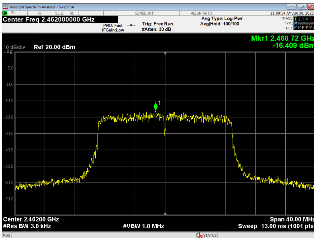
78 PSD, WiFi N 72.2MB, 2462MHz
