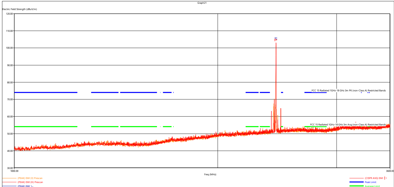
Figure 7 - Radiated Emissions Plot, 1-3.6GHz, BTBR Mid
