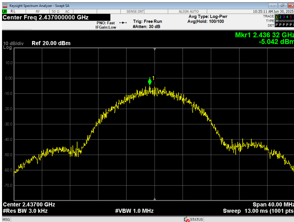
25 PSD, WiFi B 11MB, 2437MHz
