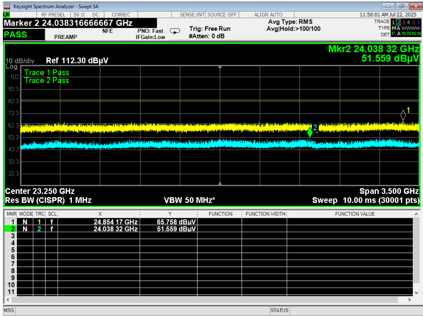
Figure 10 - Radiated Emissions Plot, 21.5-25GHz, 3EDR Mid, 1m test distance
