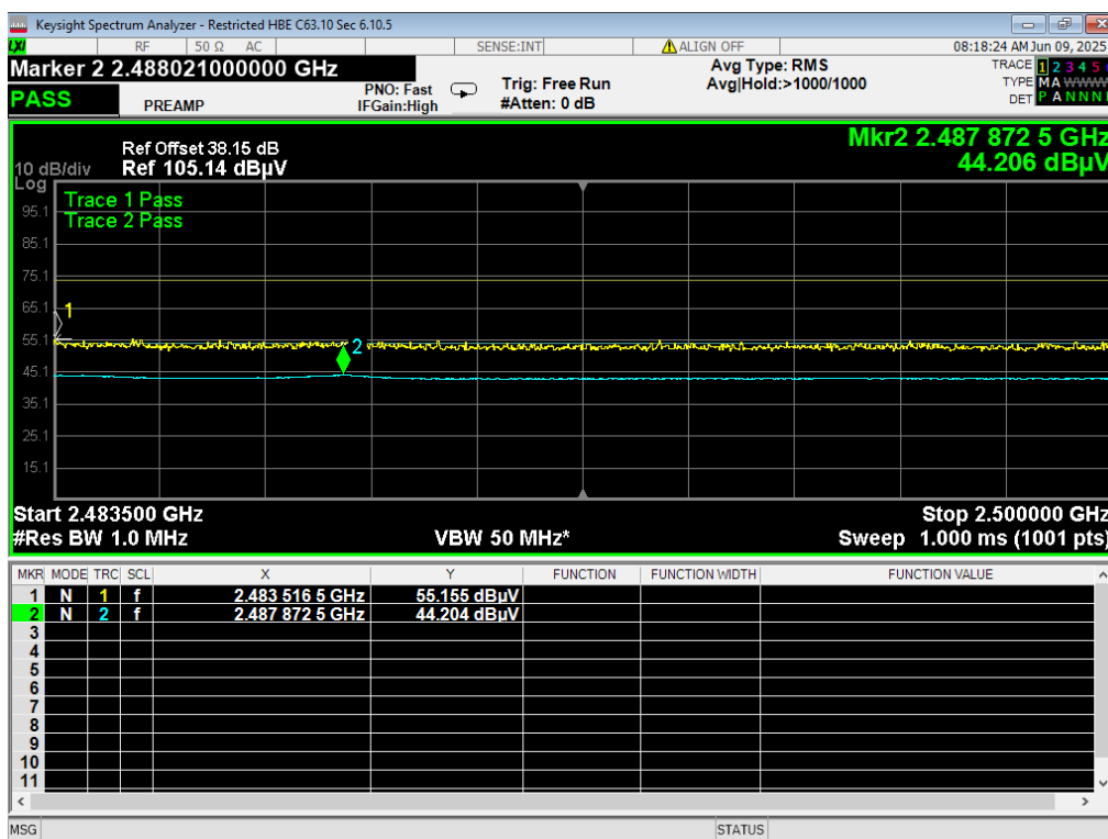
30 HBE Restricted, ANT GFSK, 2480MHz
