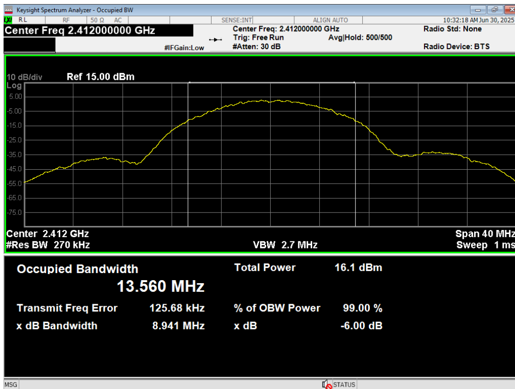
21 Occupied BW, WiFi B 11MB, 2412MHz
