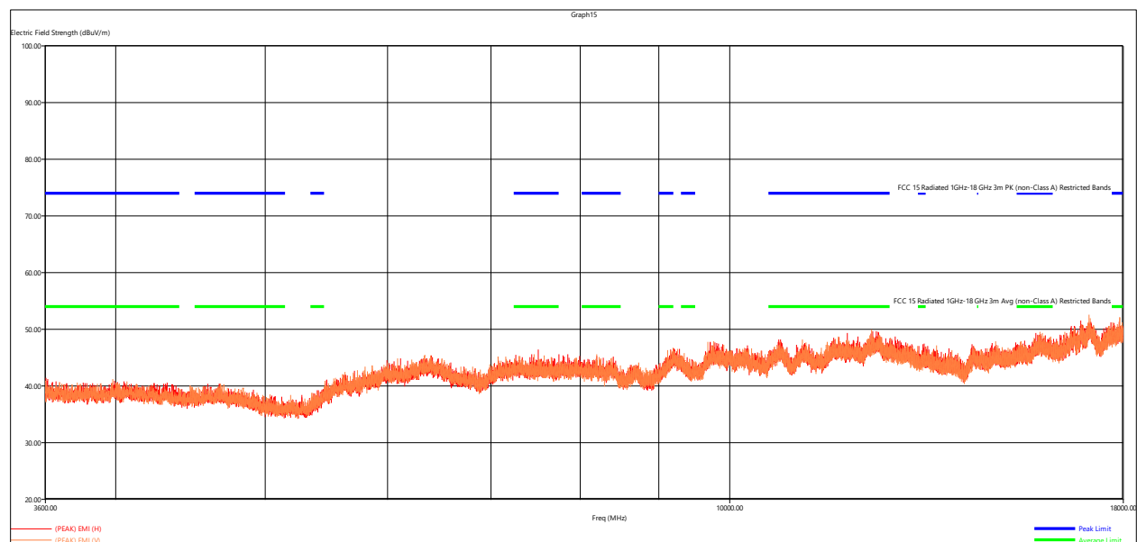
Figure 9 - Radiated Emissions Plot, 3.6-18GHz, BLE 2MB Low
