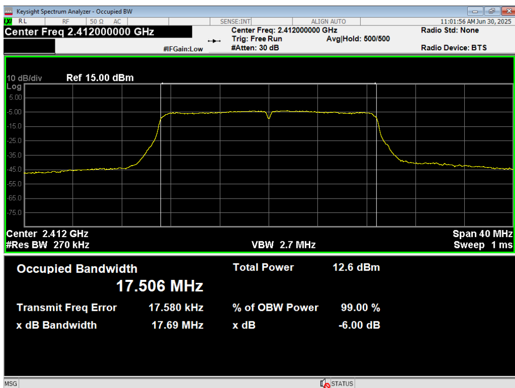
60 Occupied BW, WiFi N 6.5MB, 2412MHz
