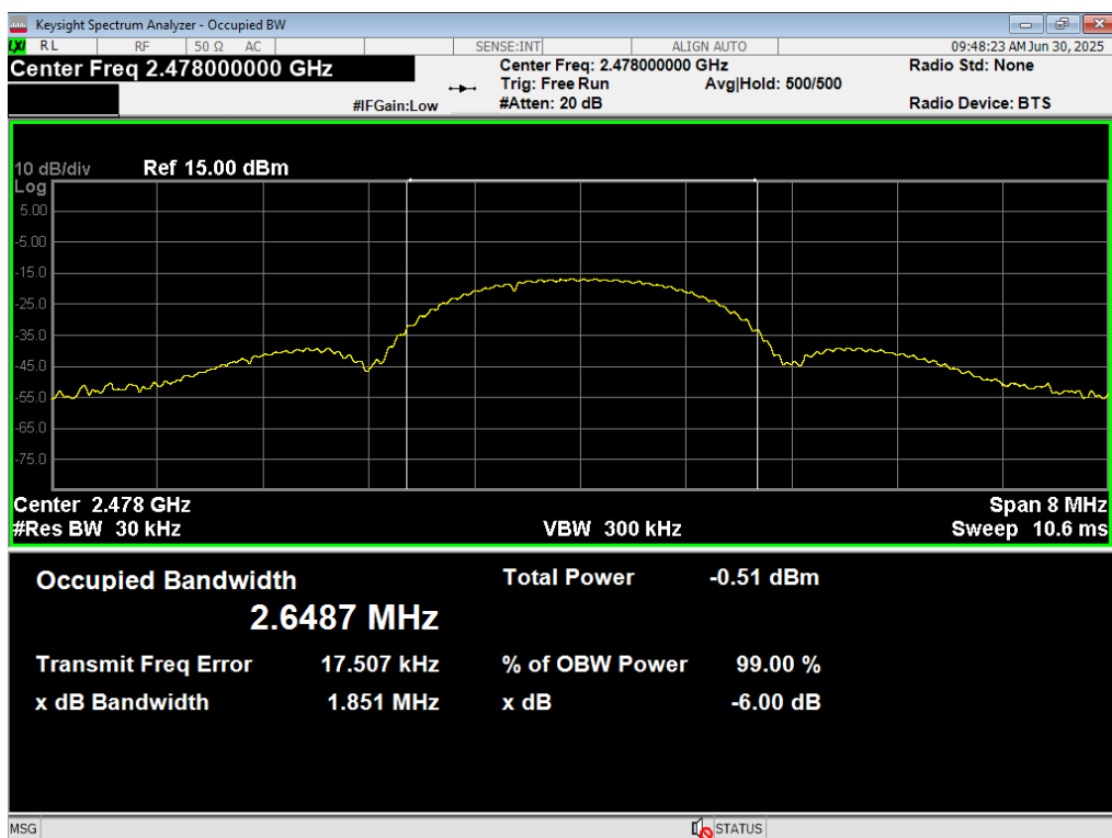
36 Occupied BW, BLE 2MB, 2478MHz
