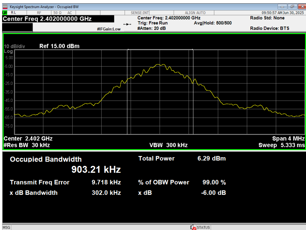
08 Occupied BW, BTBR, 2402MHz
