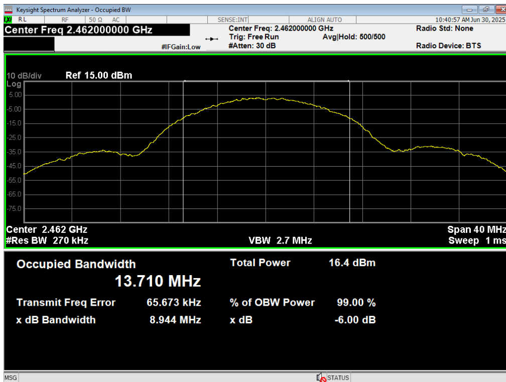
23 Occupied BW, WiFi B 11MB, 2462MHz
