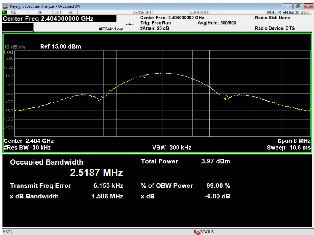
34 Occupied BW, BLE 2MB, 2404MHz
