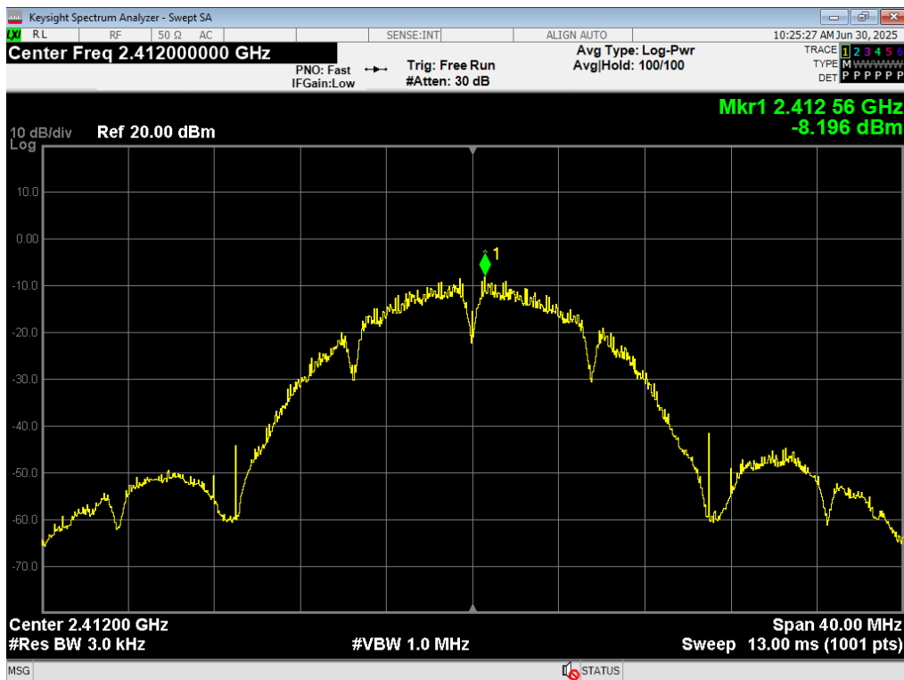
11 PSD, WiFi B 1MB, 2412MHz
