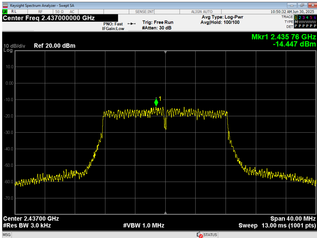
51 PSD, WiFi G 54MB, 2437MHz
