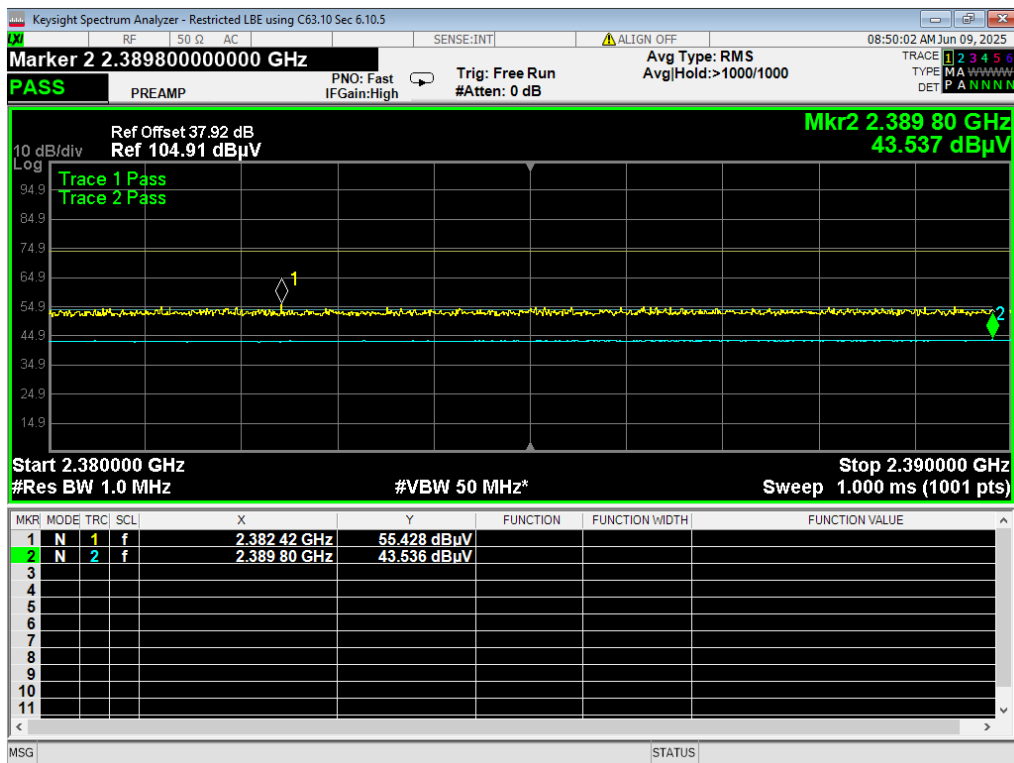
19 LBE Restricted, 3EDR, 2402MHz
