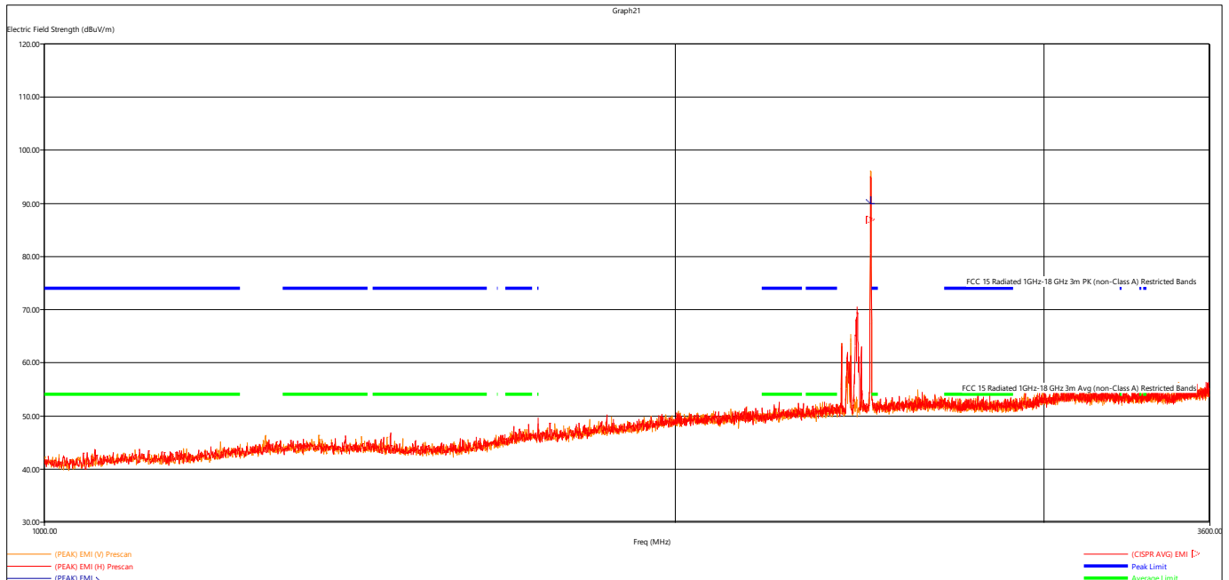
Figure 8 - Radiated Emissions Plot, 1-3.6GHz, BLE 2MB High
