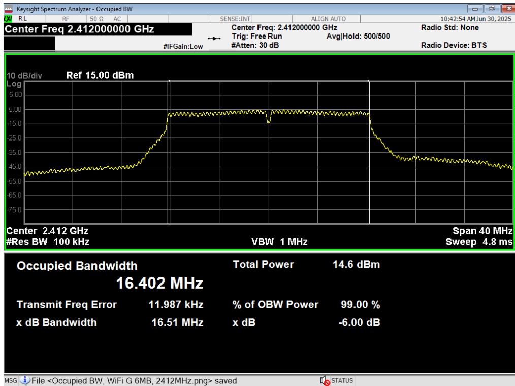
27 6dB BW, WiFi G 6MB, 2412MHz
