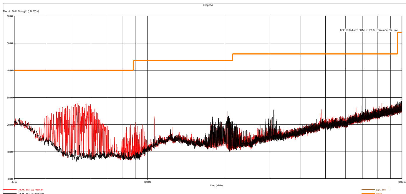
Figure 5 - Radiated Emissions Plot, 2EDR
