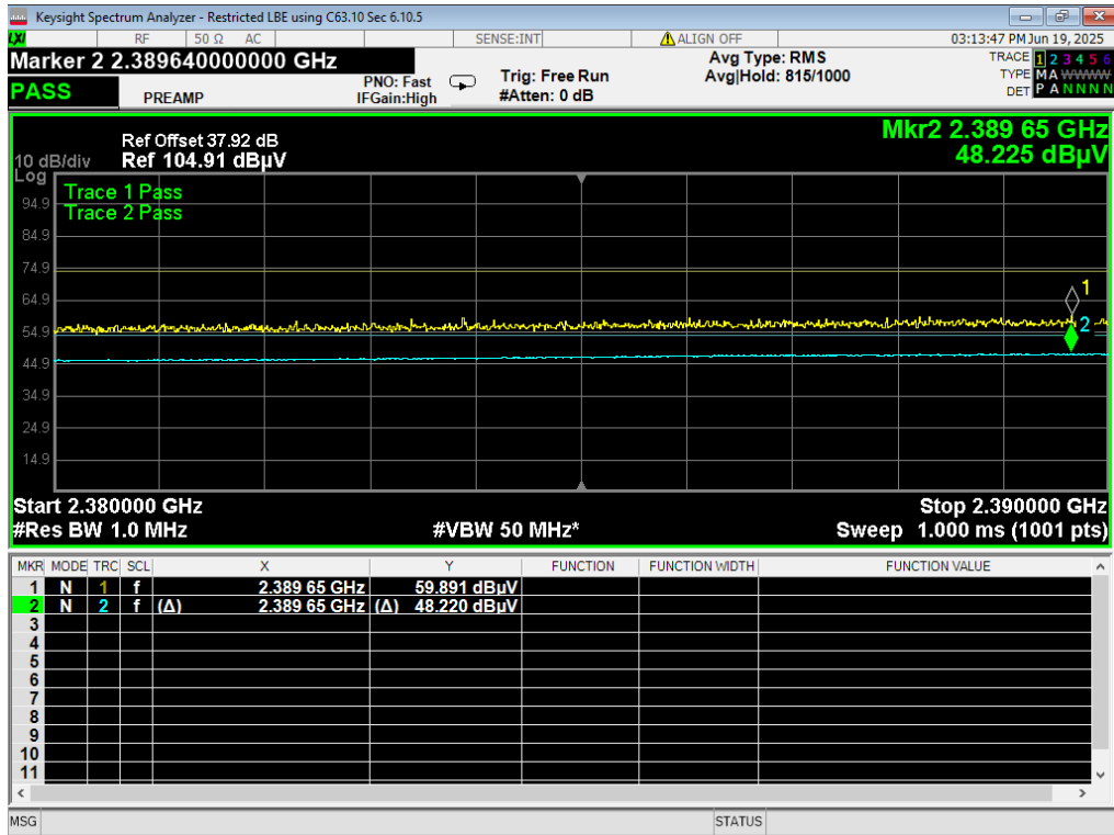
19 LBE Restricted, WiFi B 11MB, ch1 2412MHz, pwr42
