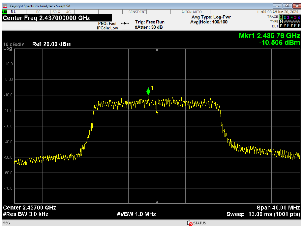
64 PSD, WiFi N 6.5MB, 2437MHz
