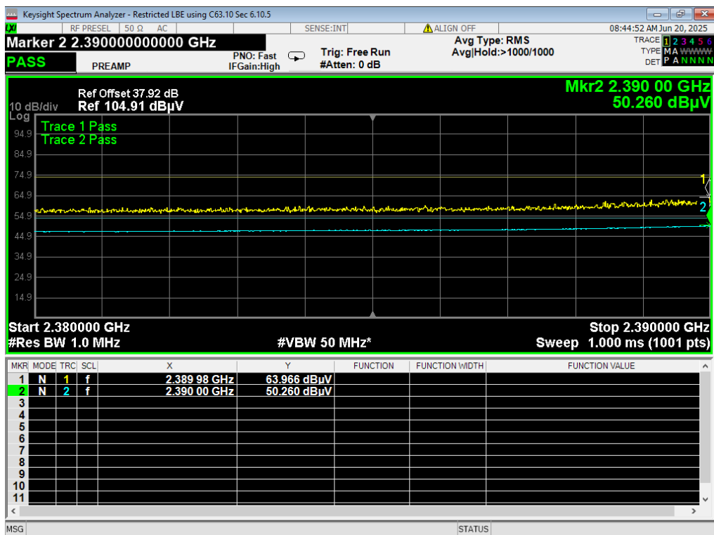
58 LBE Restricted, WiFi N 6.5MB, 2412MHz
