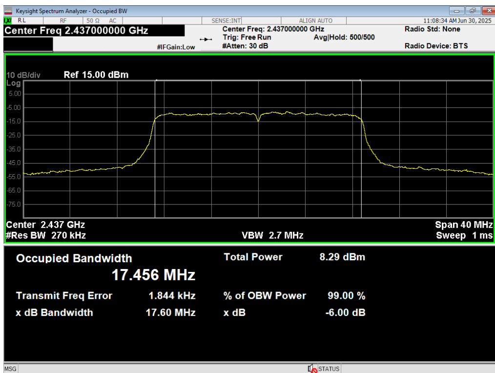
74 Occupied BW, WiFi N 72.2MB, 2437MHz
