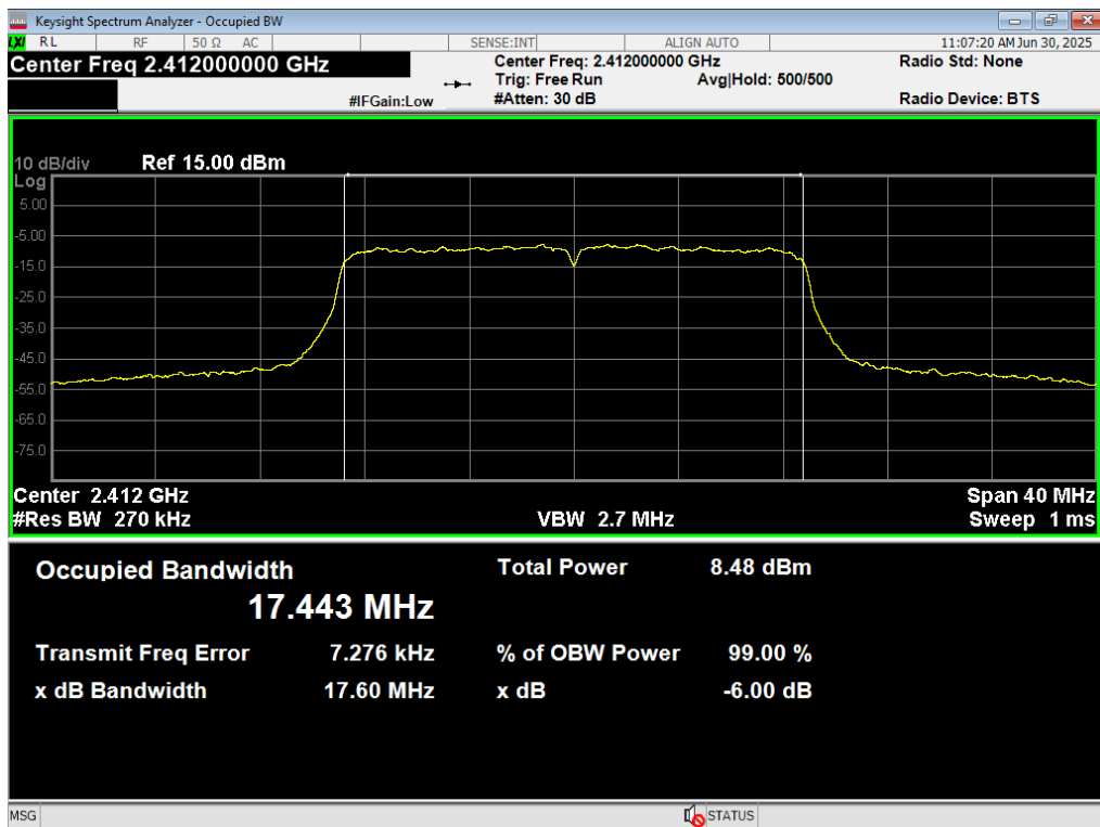
73 Occupied BW, WiFi N 72.2MB, 2412MHz
