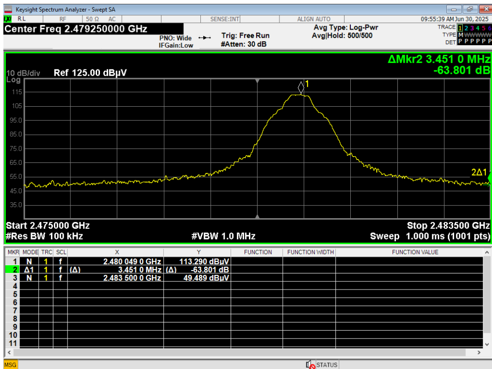
05 HBE Unrestricted, BTBR, 2480MHz
