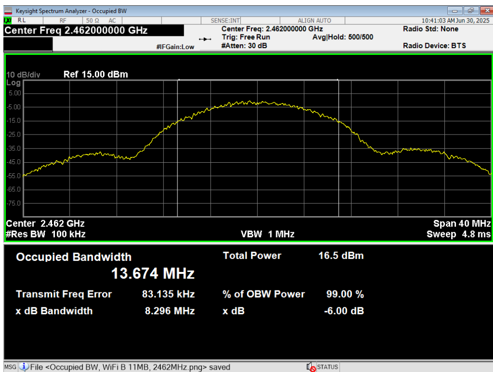
16 6dB BW, WiFi B 11MB, 2462MHz
