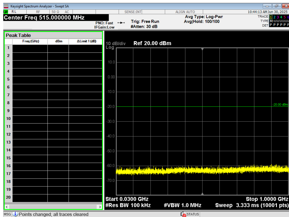
Figure 24 - Conducted Spurious Plot, WIFI 802.11g, 30M – 1G, Mid
