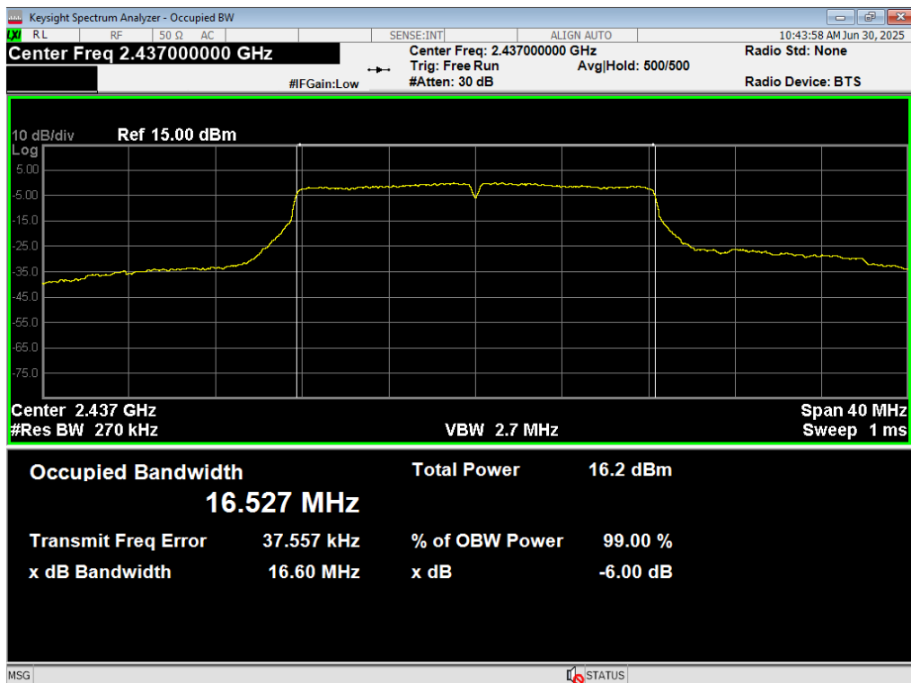
35 Occupied BW, WiFi G 6MB, 2437MHz
