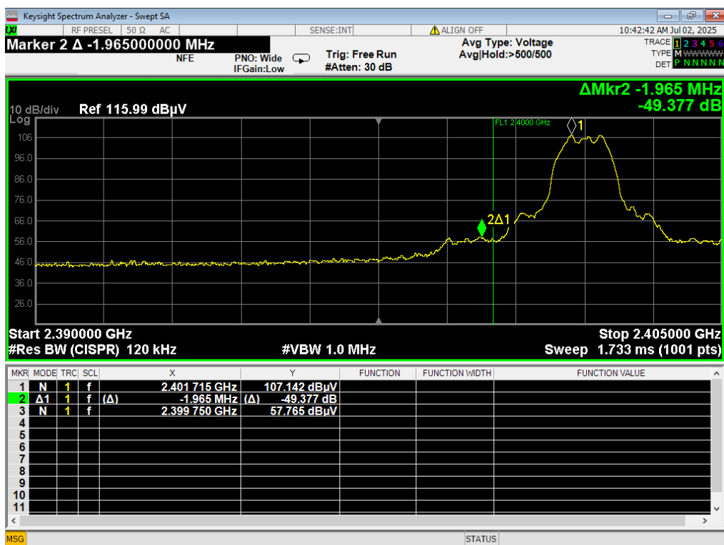
20 LBE Unrestricted, 3EDR
