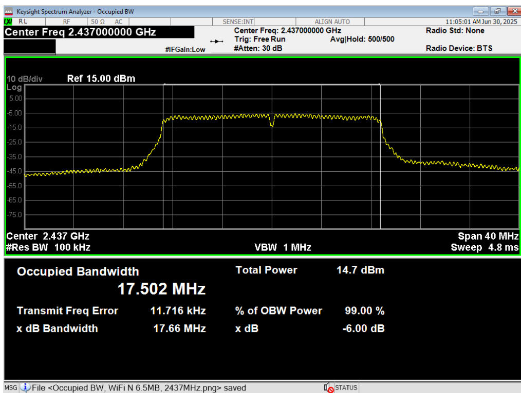
54 6dB BW, WiFi N 6.5MB, 2437MHz
