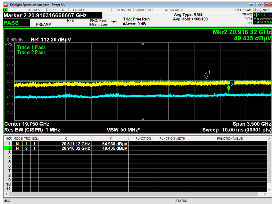
Figure 10 - Radiated Emissions Plot, 18-21.5GHz, BLE 2MB Mid, 1m test distance No emissions were found above lab noise floor, tabular data not provided
