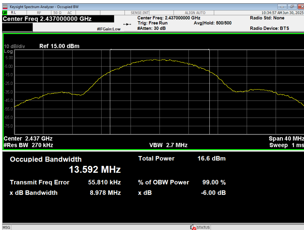
22 Occupied BW, WiFi B 11MB, 2437MHz
