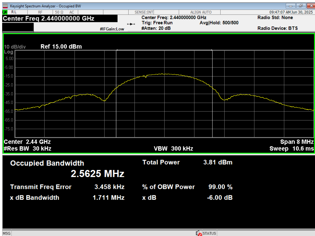
35 Occupied BW, BLE 2MB, 2440MHz
