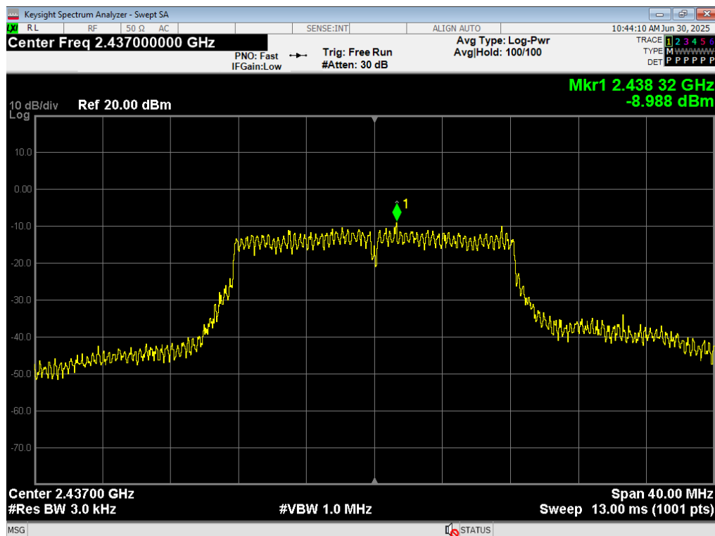
38 PSD, WiFi G 6MB, 2437MHz
