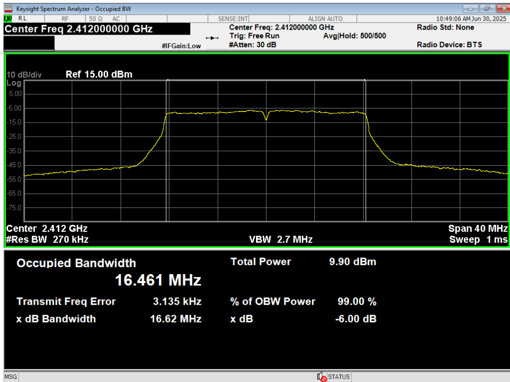
47 Occupied BW, WiFi G 54MB, 2412MHz
