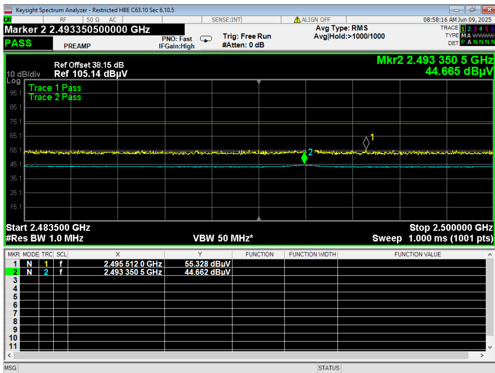
04 HBE Restricted, BTBR, 2480MHz
