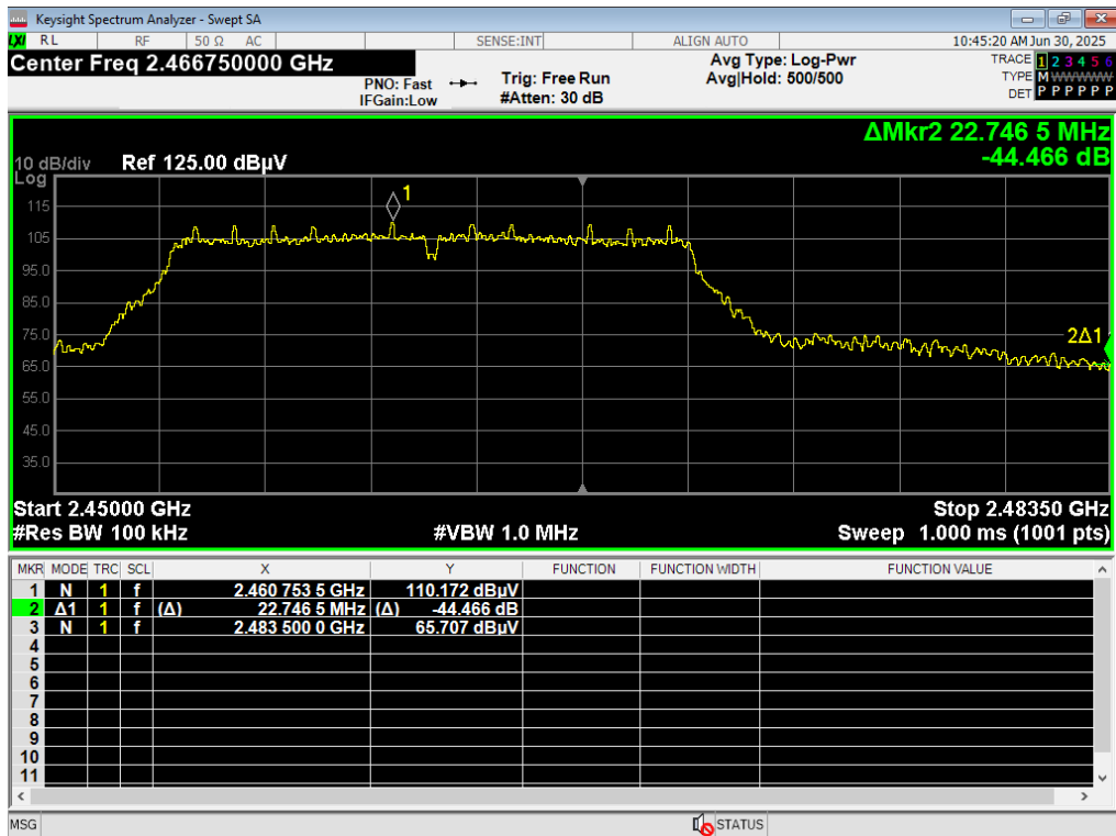
31 HBE Unrestricted, WiFi G 6MB, 2462MHz
