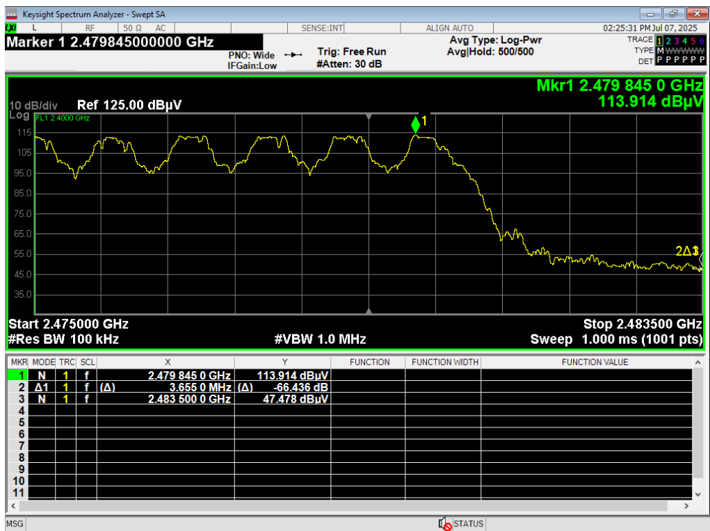
14 HBE Unrestricted, BTBR Hopping
