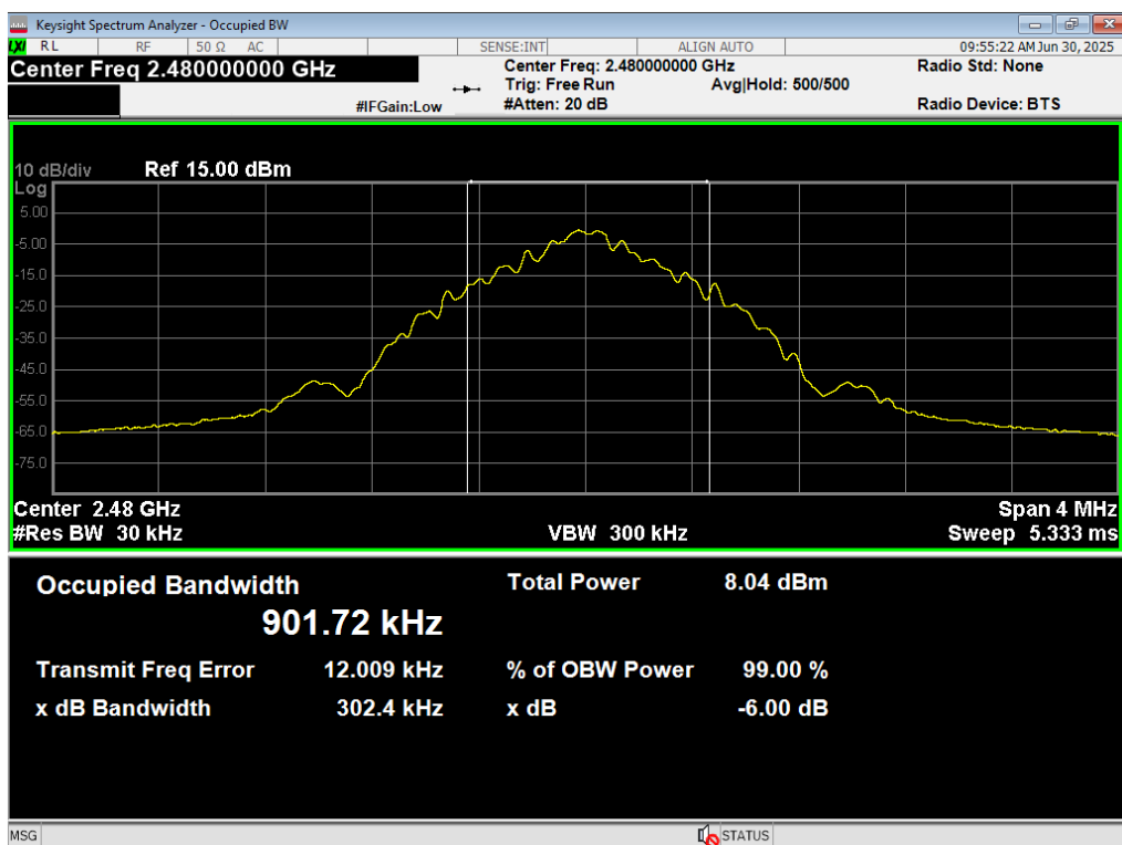
10 Occupied BW, BTBR, 2480MHz
