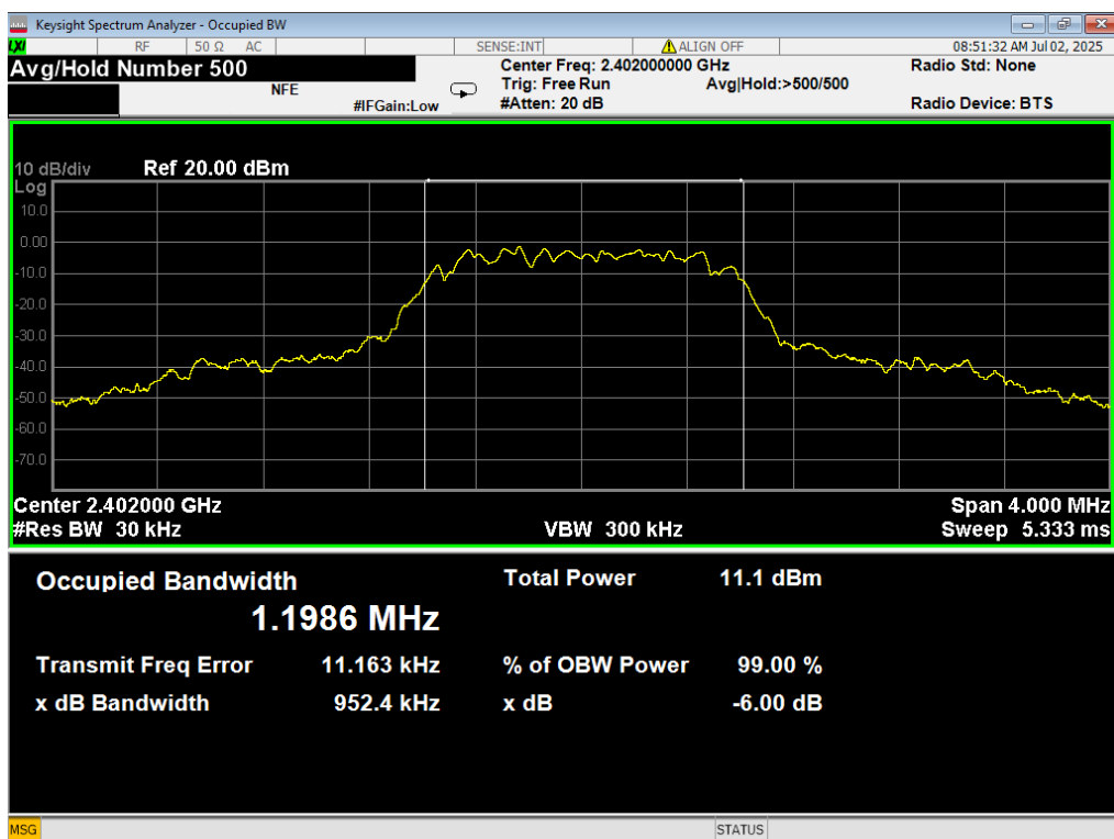
08 Occupied BW, 2EDR, 2402MHz
