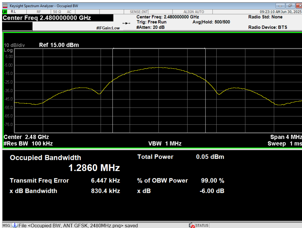
03 6dB BW, ANT GFSK, 2480MHz
