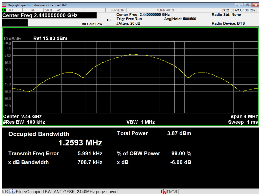
02 6dB BW, ANT GFSK, 2440MHz
