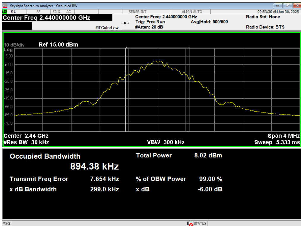
09 Occupied BW, BTBR, 2440MHz
