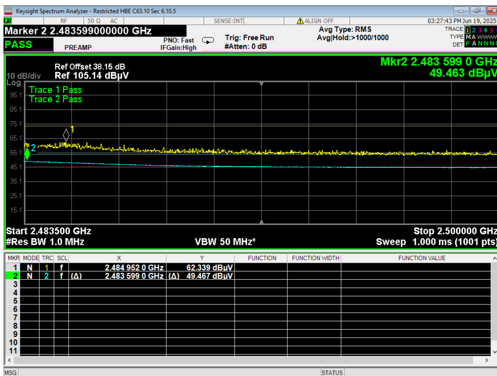
56 HBE Restricted, WiFi N 6.5MB, 2462MHz
