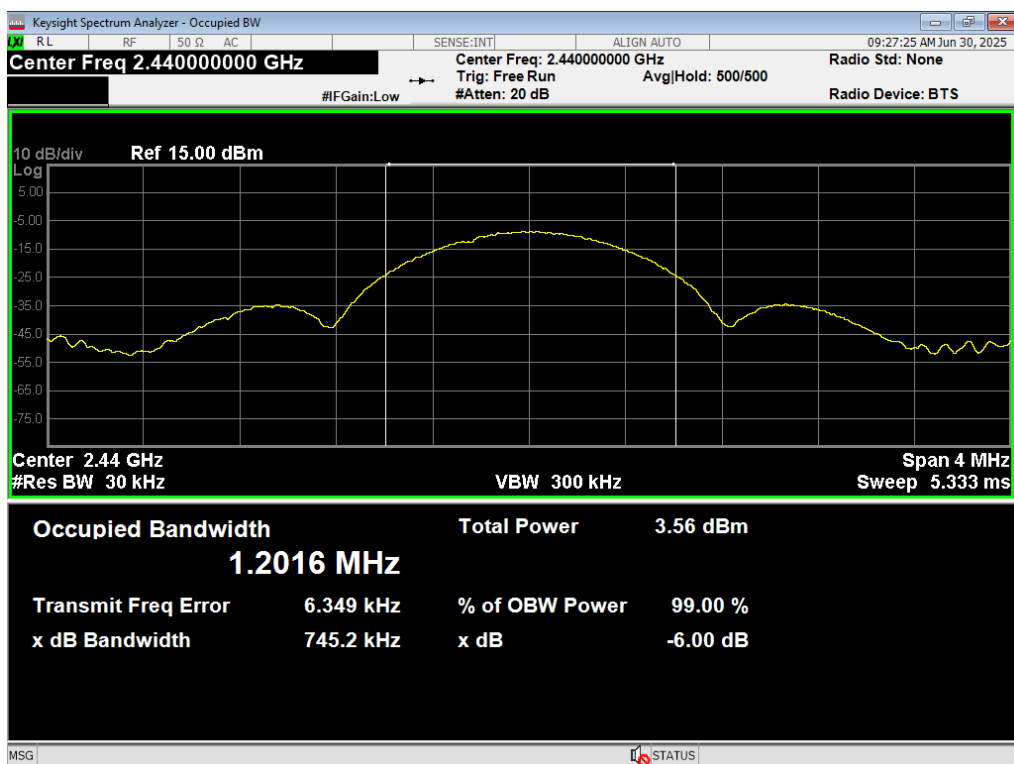
22 Occupied BW, BLE 1MB, 2440MHz
