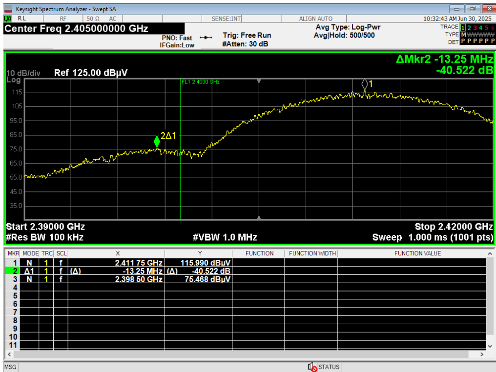
20 LBE Unrestricted, WiFi B 11MB, 2412MHz
