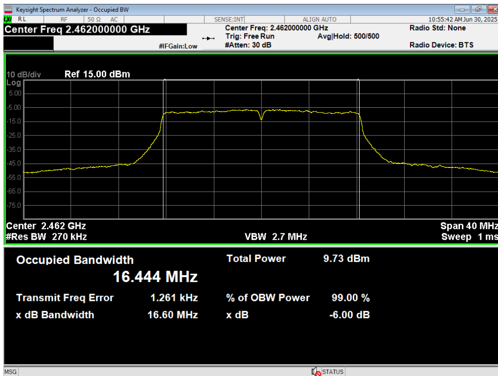
49 Occupied BW, WiFi G 54MB, 2462MHz
