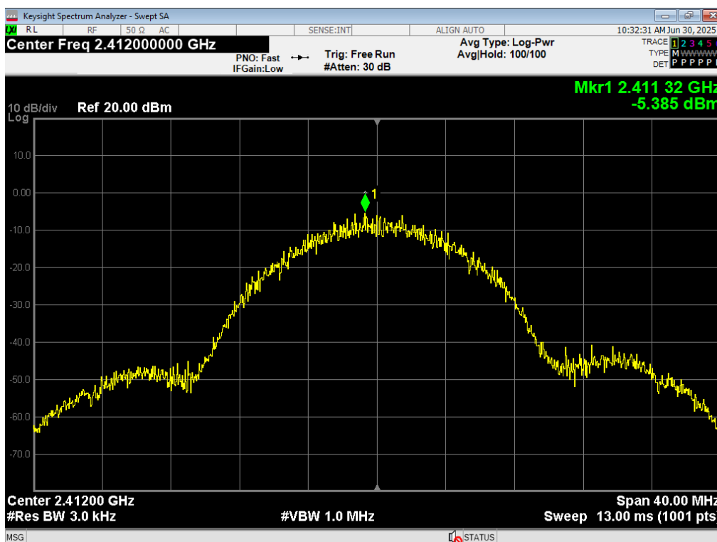
24 PSD, WiFi B 11MB, 2412MHz
