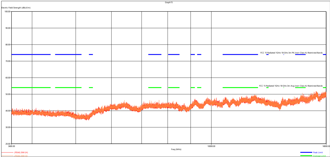
Figure 8 - Radiated Emissions Plot, 3.6-18GHz, 3EDR Low
