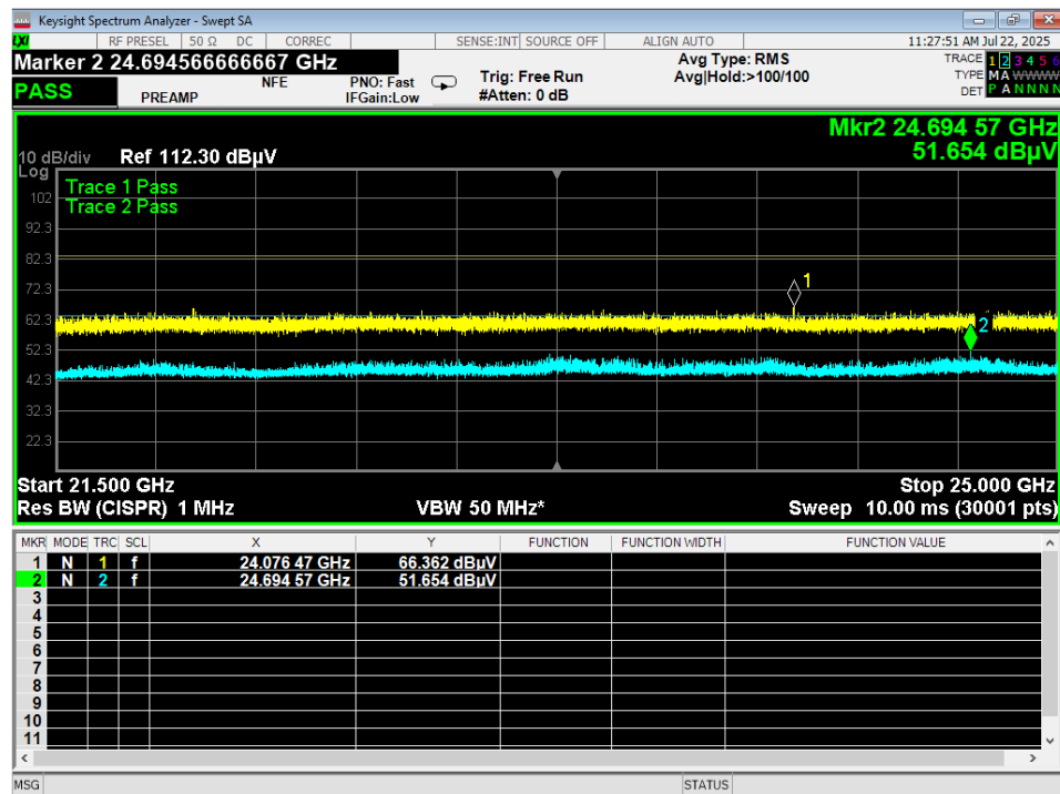
Figure 20 - Radiated Emissions Plot, 21.5-25GHz, 802.11b 1MB Mid, 1m test distance No emissions were found above lab noise floor, tabular data not provided
