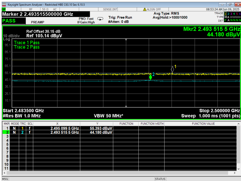
17 HBE Restricted, 3EDR, 2480MHz
