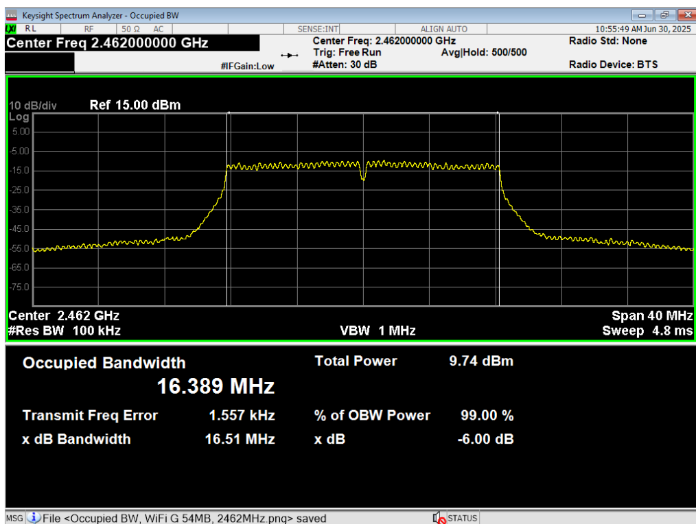
42 6dB BW, WiFi G 54MB, 2462MHz
