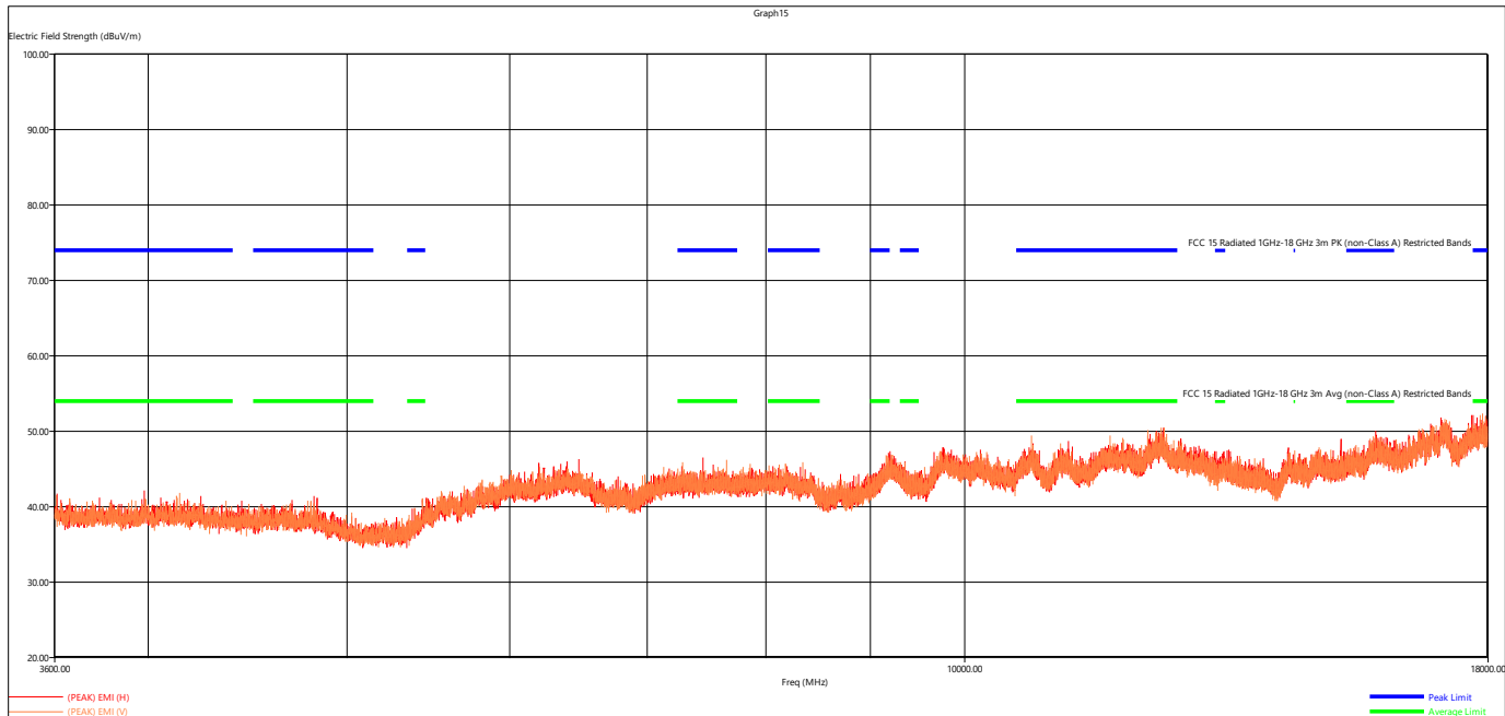
Figure 8 - Radiated Emissions Plot, 3.6-18GHz, BTBR Mid
