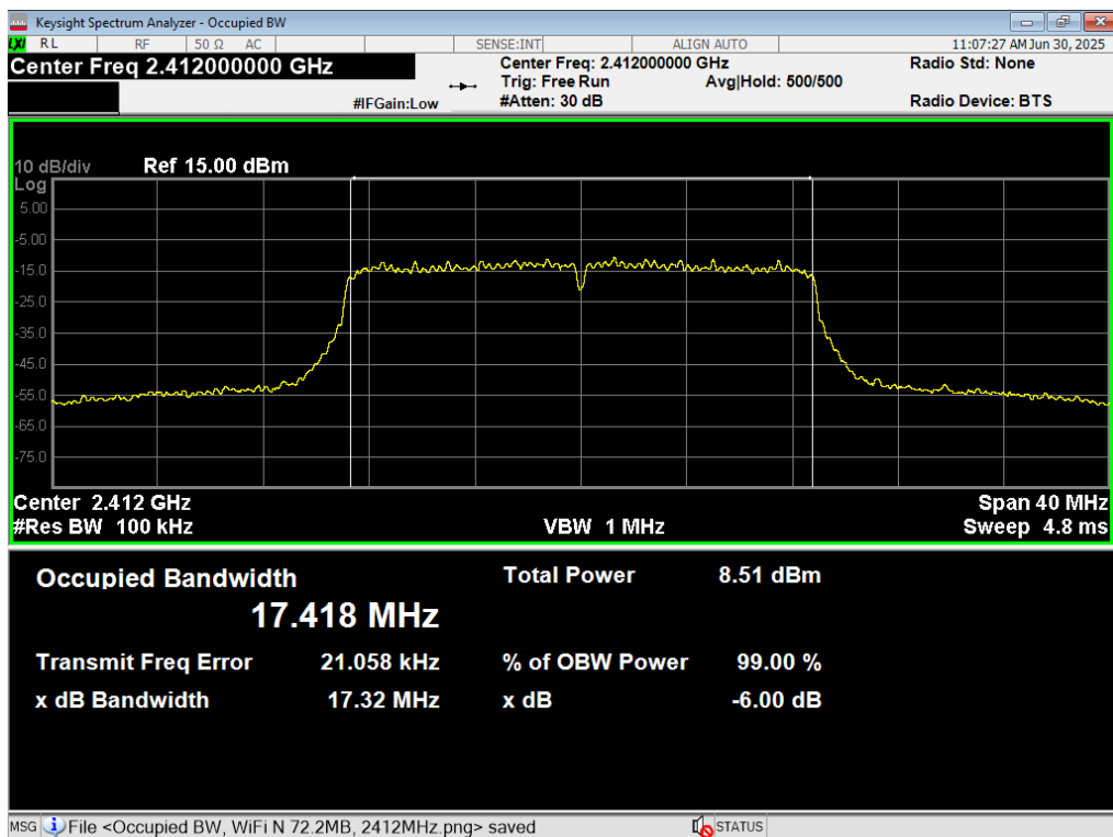
66 6dB BW, WiFi N 72.2MB, 2412MHz
