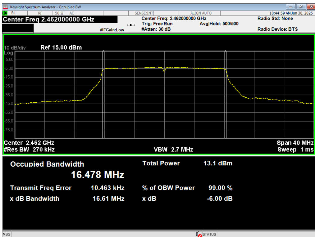
36 Occupied BW, WiFi G 6MB, 2462MHz
