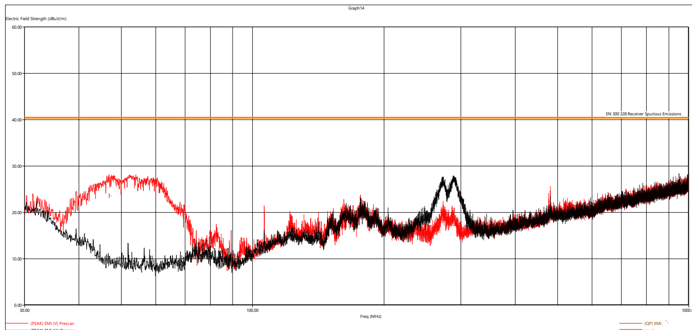
Figure 16 - Radiated Emissions Plot, 802.11n 72.2MB
