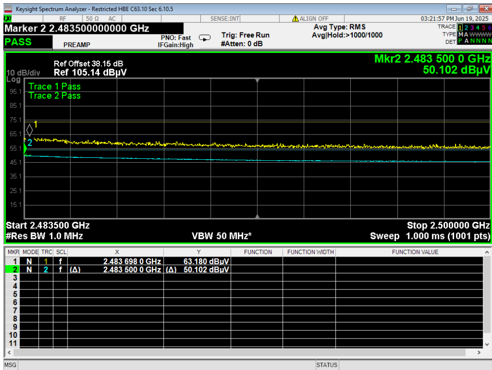
30 HBE Restricted, WiFi G 6MB, ch11, 2462MHz
