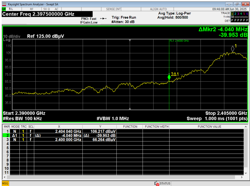
33 LBE Unrestricted, BLE 2MB, 2404MHz
