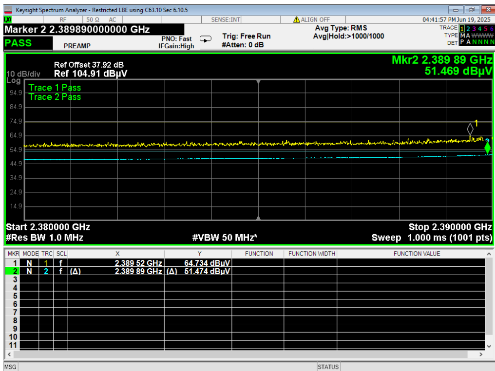
32 LBE Restricted, WiFi G 6MB, ch1 2412MHz
