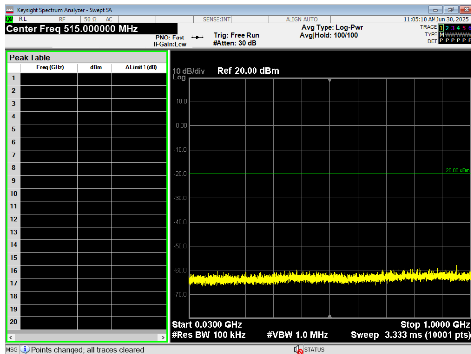
Figure 27 - Conducted Spurious Plot, WIFI 802.11n, 30M – 1G, Mid
