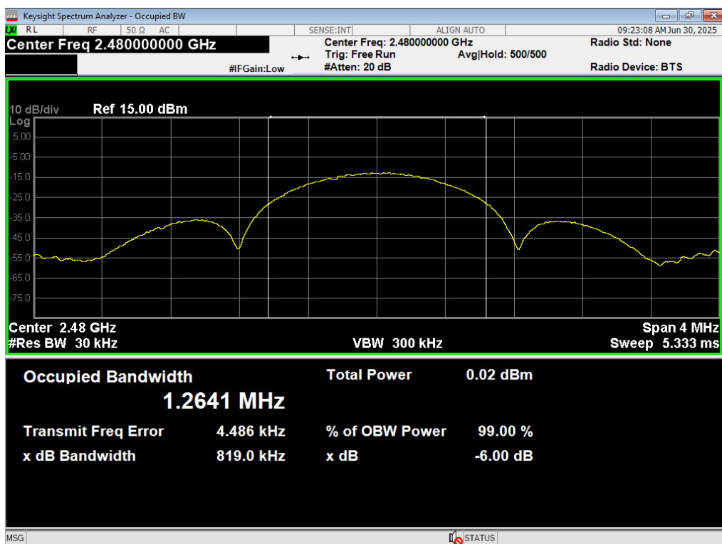
10 Occupied BW, ANT GFSK, 2480MHz
