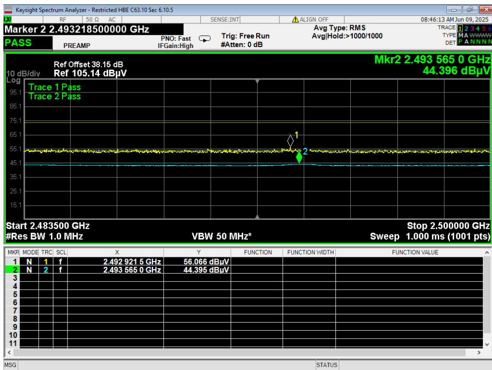
04 HBE Restricted, 2EDR, 2480MHz
