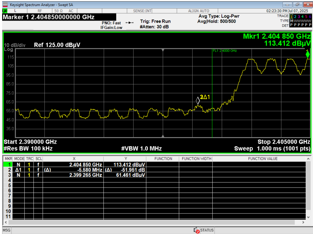
15 LBE Unrestricted, BTBR Hopping
