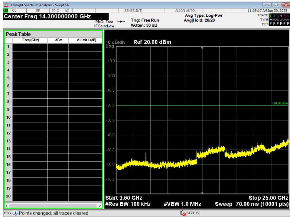
Figure 29 - Conducted Spurious Plot, WIFI 802.11n, 3.6G – 25G, Mid
