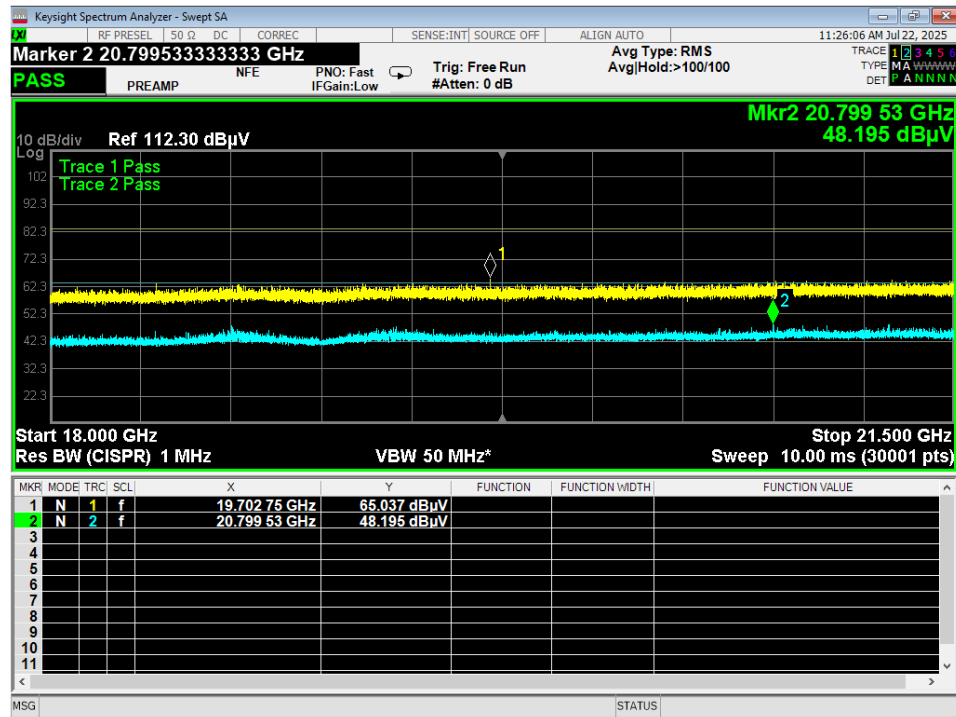
Figure 19 - Radiated Emissions Plot, 18-21.5GHz, 802.11b 1MB Mid, 1m test distance No emissions were found above lab noise floor, tabular data not provided
