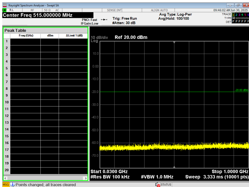
Figure 18 - Conducted Spurious Plot, GMSK 2MB, 30MHz – 1GHz, Low
