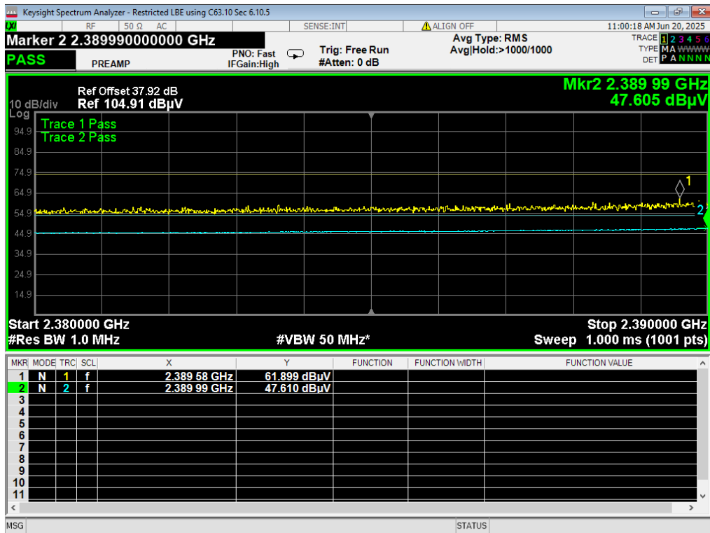
71 LBE Restricted, WiFi N 72.2MB, 2412MHz
