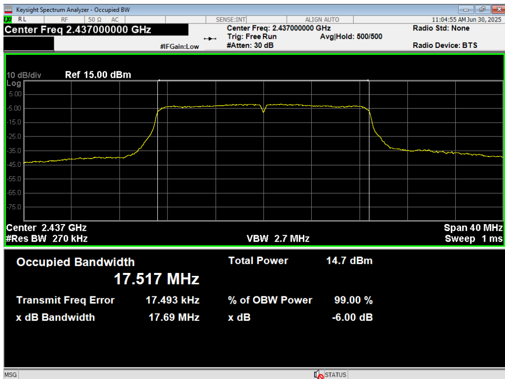
61 Occupied BW, WiFi N 6.5MB, 2437MHz
