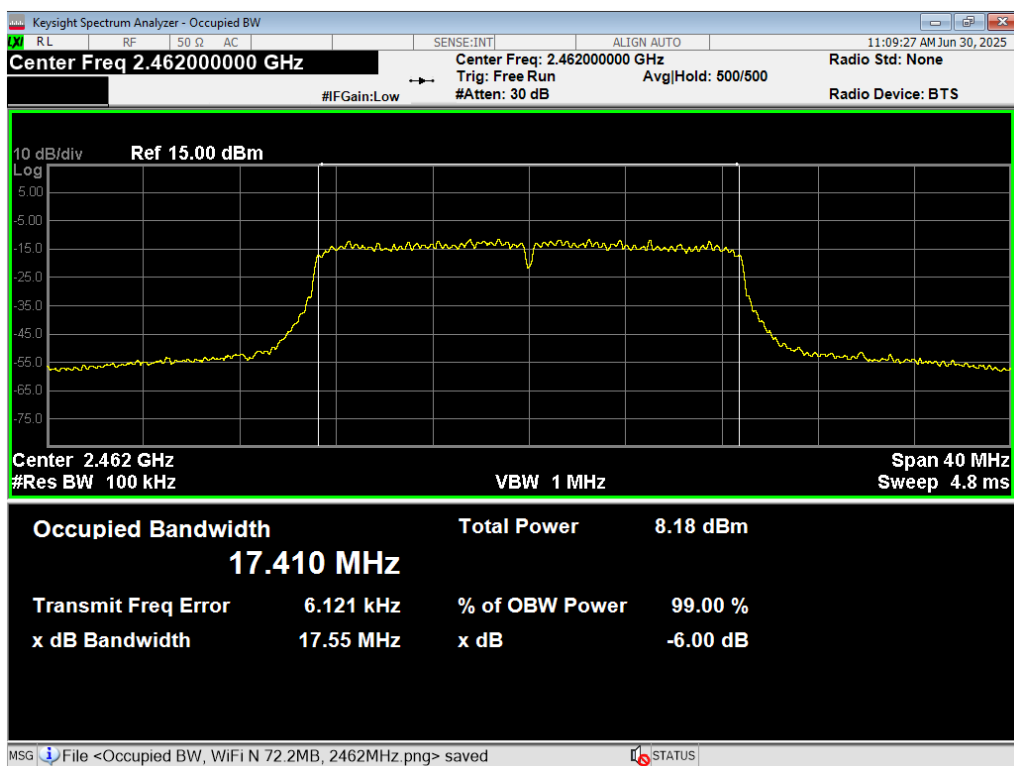
68 6dB BW, WiFi N 72.2MB, 2462MHz
