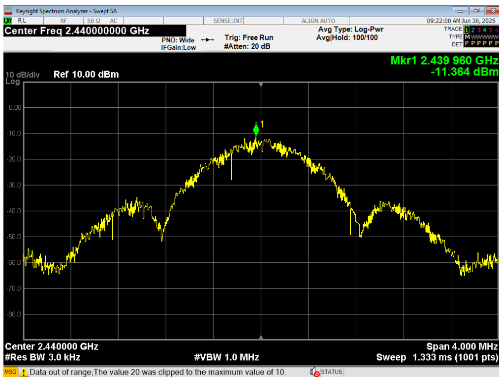
12 PSD, ANT GFSK, 2440MHz
