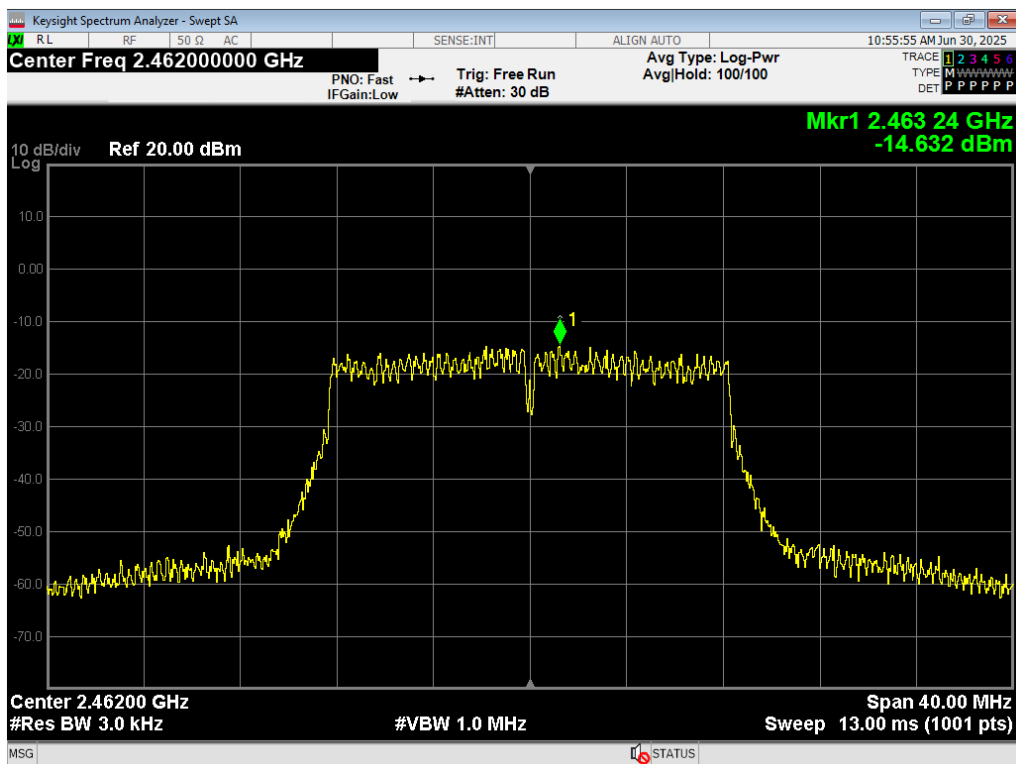
52 PSD, WiFi G 54MB, 2462MHz
