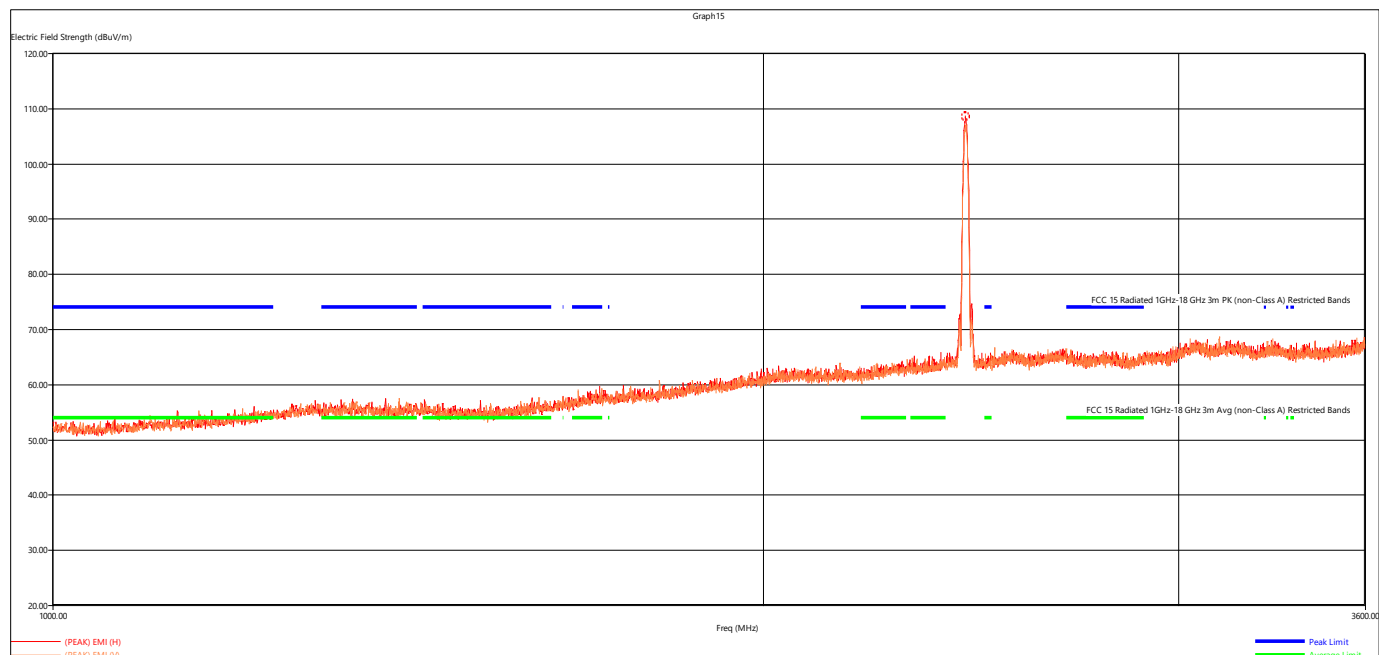
Figure 17 - Radiated Emissions Plot, 1-3.6GHz, 802.11b 1MB Low
