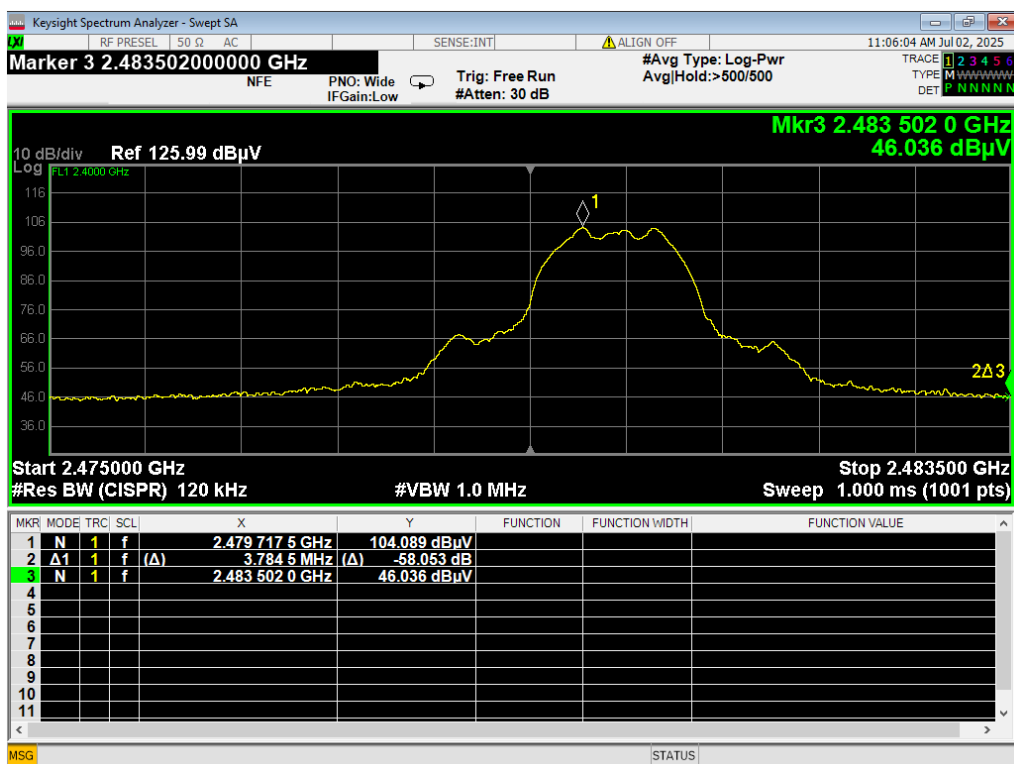
18 HBE Unrestricted, 3EDR
