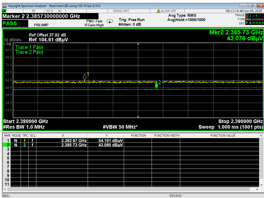
06 LBE Restricted, ANT GFSK, 2402MHz
