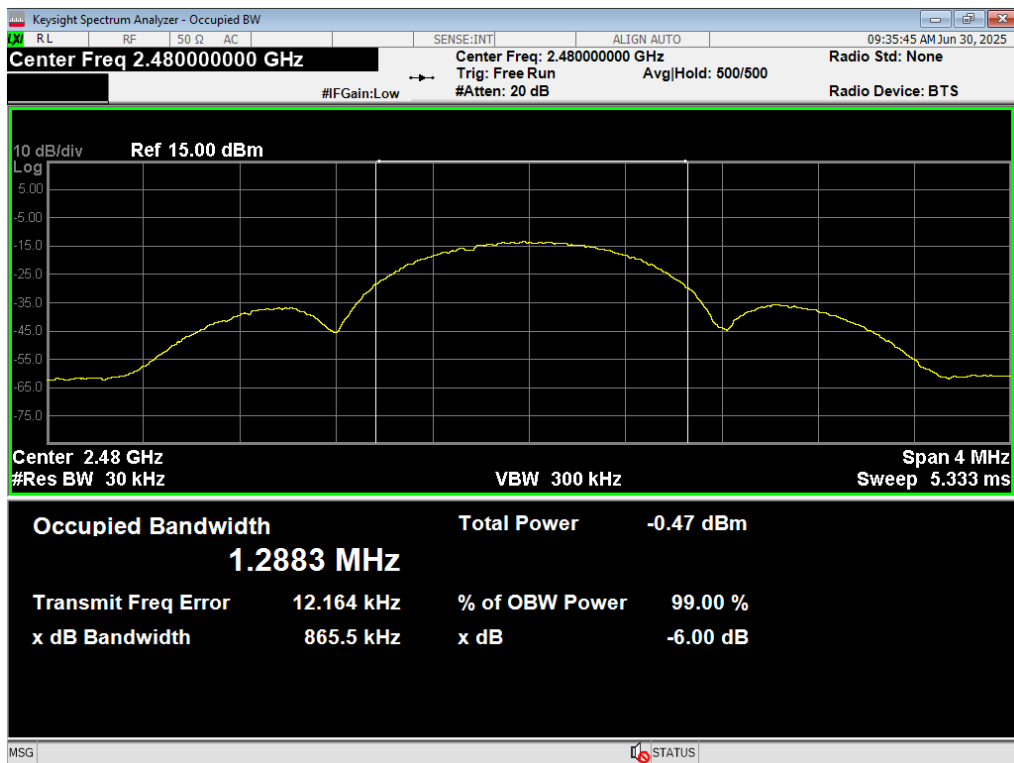
23 Occupied BW, BLE 1MB, 2480MHz
