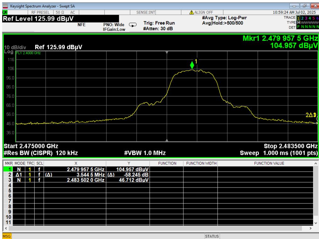
05 HBE Unrestricted, 2EDR
