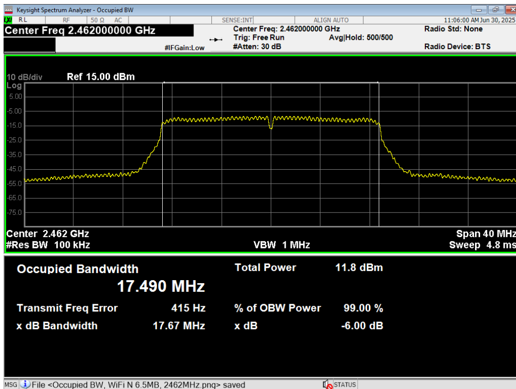
55 6dB BW, WiFi N 6.5MB, 2462MHz
