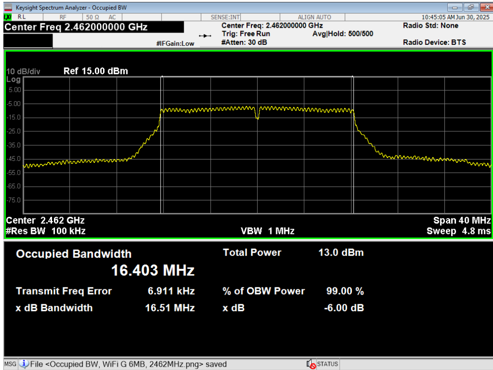
29 6dB BW, WiFi G 6MB, 2462MHz
