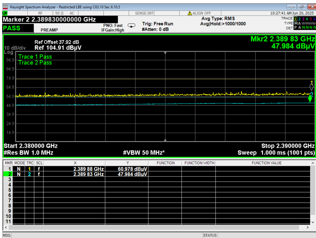
06 LBE Restricted, WiFi B 1MB, ch1 2412MHz, pwr42
