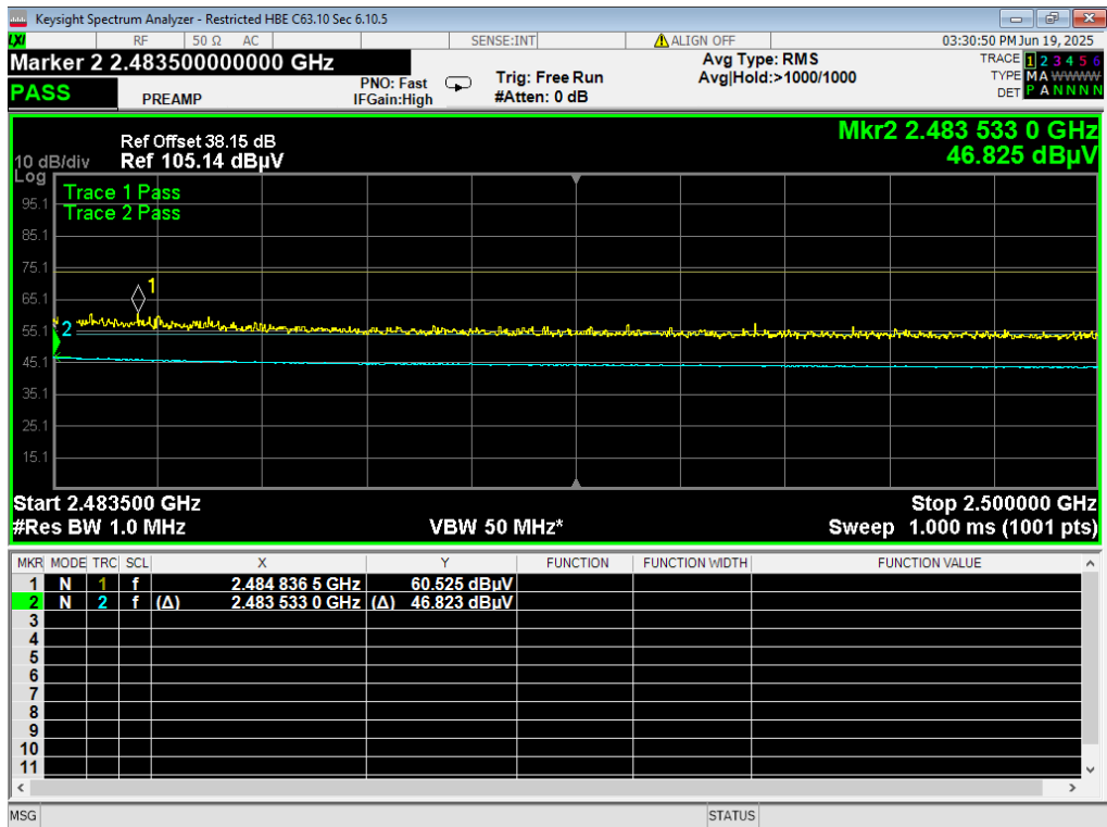
69 HBE Restricted, WiFi N 72.2MB, 2462MHz
