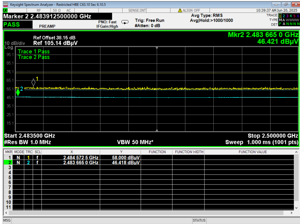
17 HBE Restricted, WiFi B 11MB, ch11 2462MHz, pwr42
