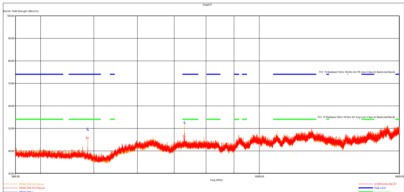
Figure 18 - Radiated Emissions Plot, 3.6-18GHz, 802.11b 1MB Low
