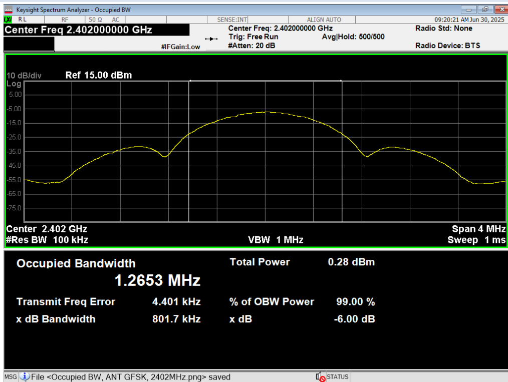
01 6dB BW, ANT GFSK, 2402MHz
