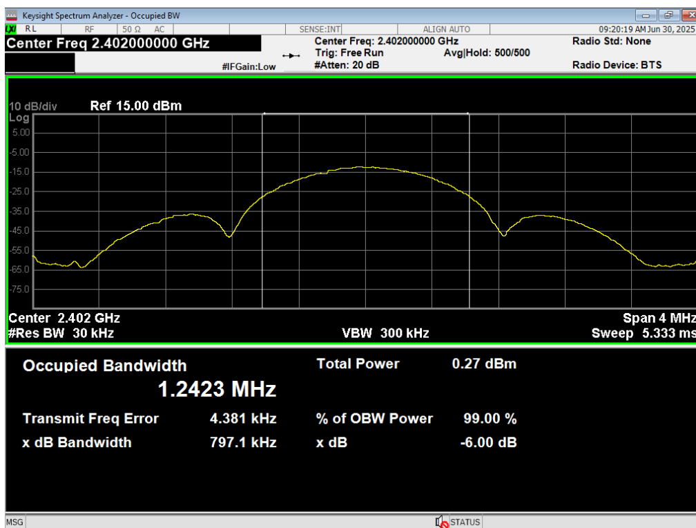
08 Occupied BW, ANT GFSK, 2402MHz
