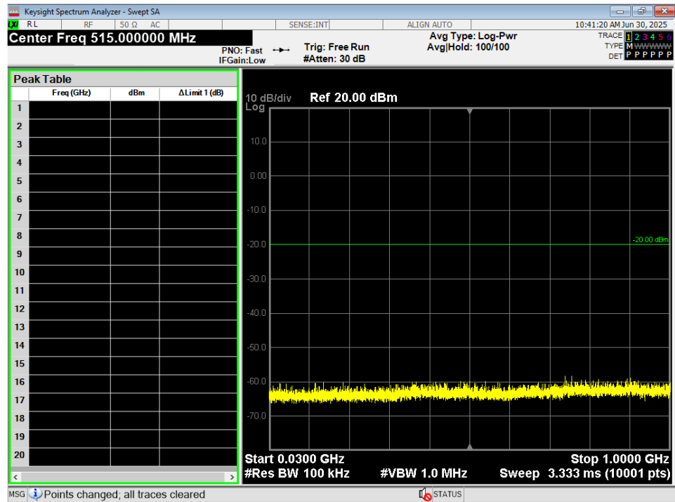
Figure 21 – Conducted Spurious Plot, WIFI 802.11b, 30M – 1G, High
