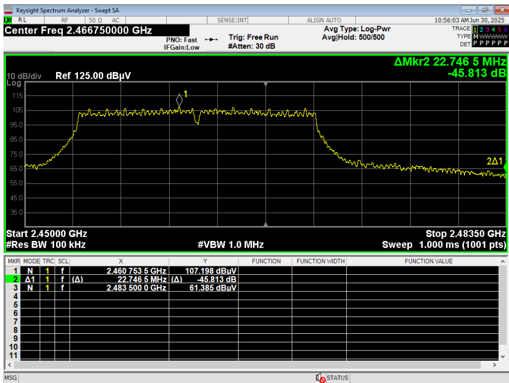
44 HBE Unrestricted, WiFi G 54MB, 2462MHz
