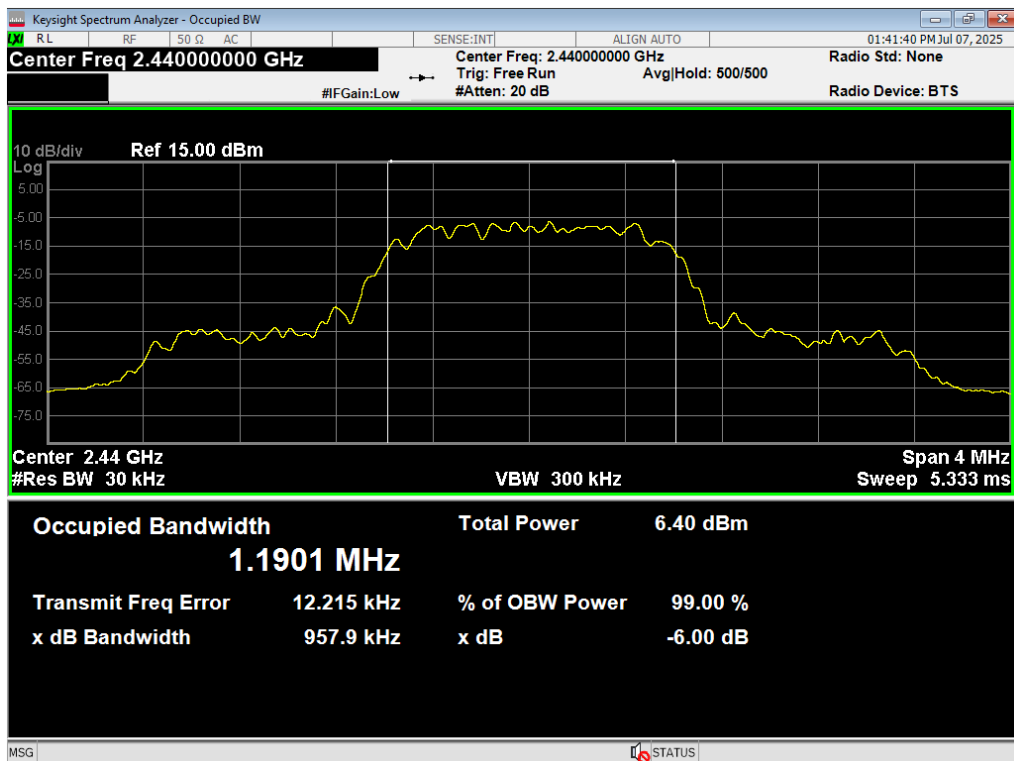
09 Occupied BW, 2EDR, 2440MHz
