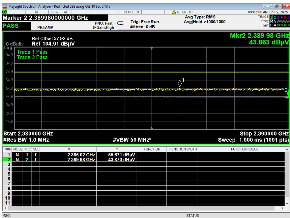
06 LBE Restricted, BTBR, 2402MHz
