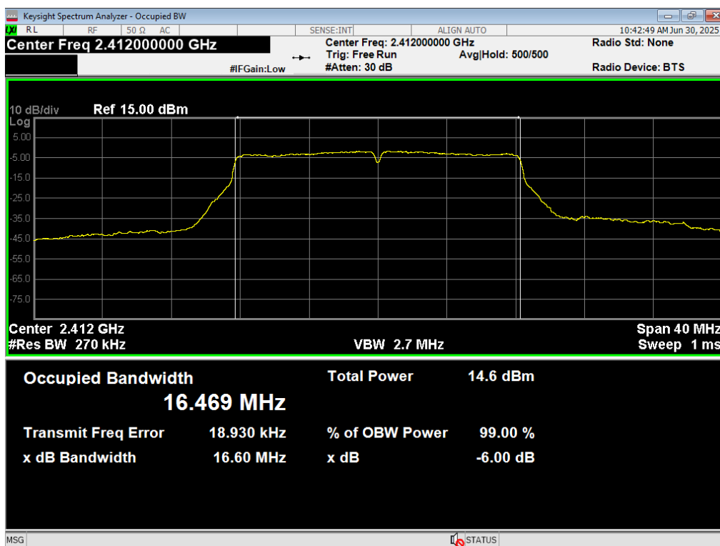
34 Occupied BW, WiFi G 6MB, 2412MHz
