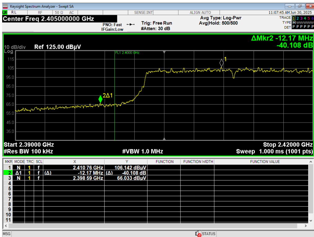
72 LBE Unrestricted, WiFi N 72.2MB, 2412MHz
