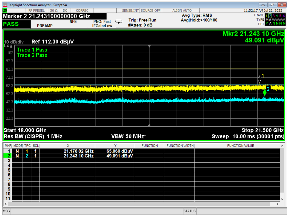
Figure 9 - Radiated Emissions Plot, 18-21.5GHz, BTBR Mid, 1m test distance No emissions were found above lab noise floor, tabular data not provided
