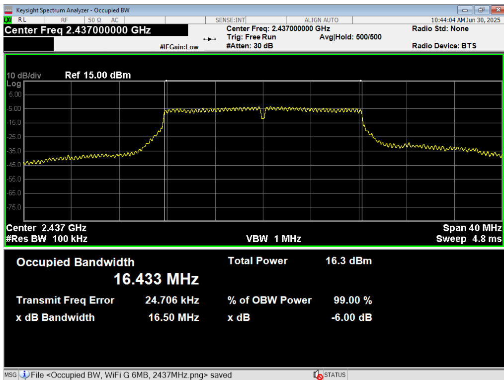
28 6dB BW, WiFi G 6MB, 2437MHz
