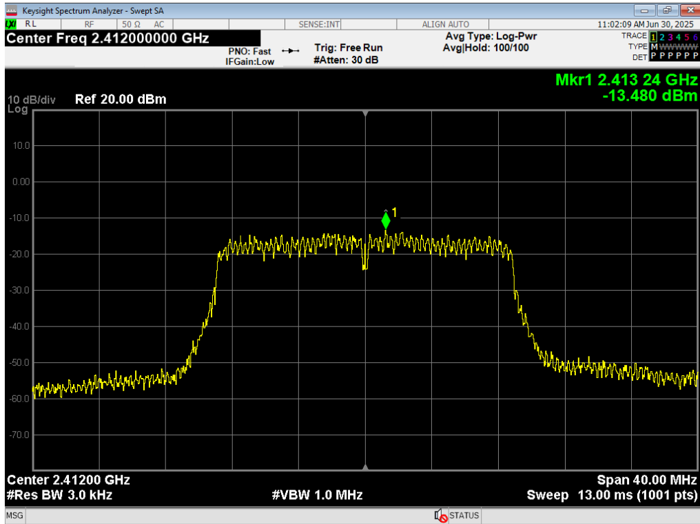
63 PSD, WiFi N 6.5MB, 2412MHz
