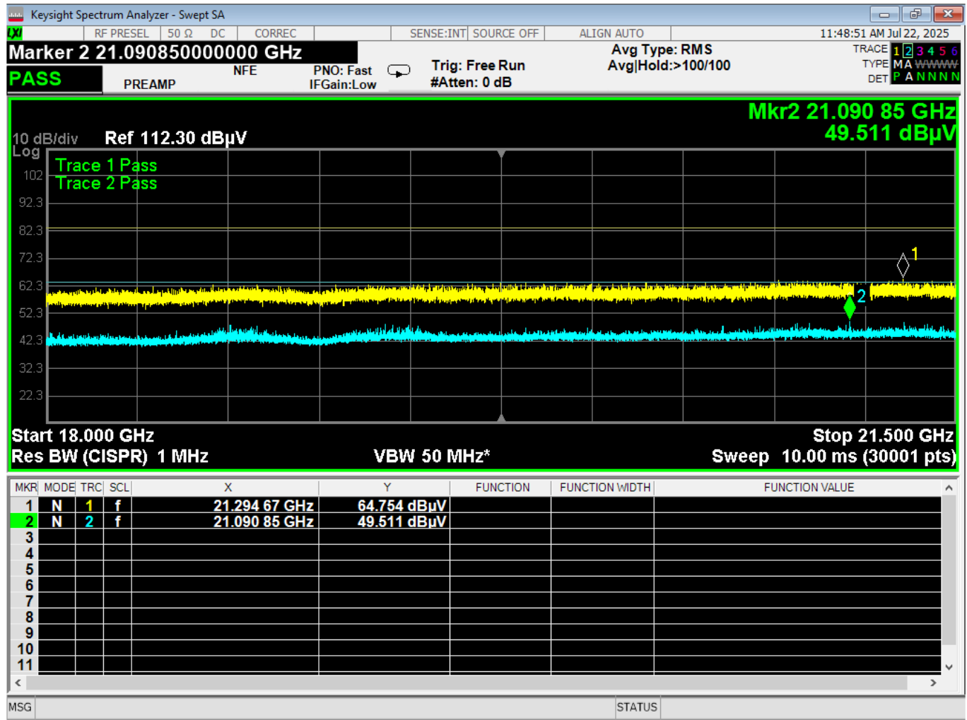
Figure 9 - Radiated Emissions Plot, 18-21.5GHz, 3EDR Mid, 1m test distance No emissions were found above lab noise floor, tabular data not provided
