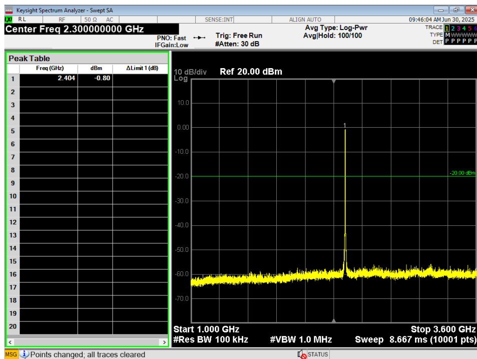
Figure 19 - Conducted Spurious Plot, GMSK 2MB, 1GHz – 3.6GHz, Low
