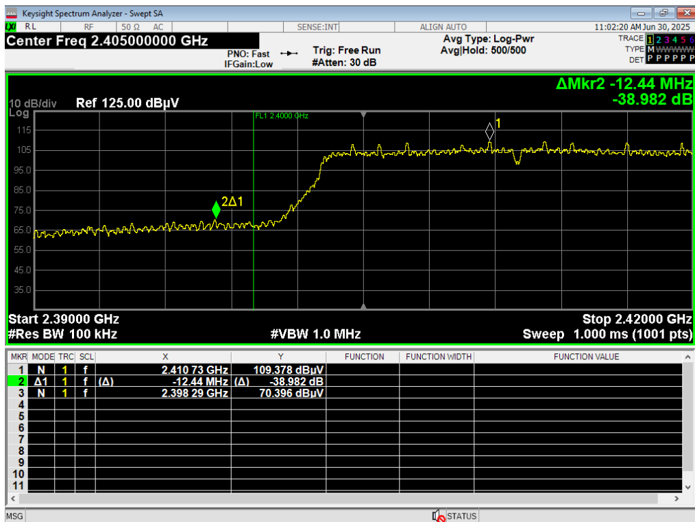
59 LBE Unrestricted, WiFi N 6.5MB, 2412MHz
