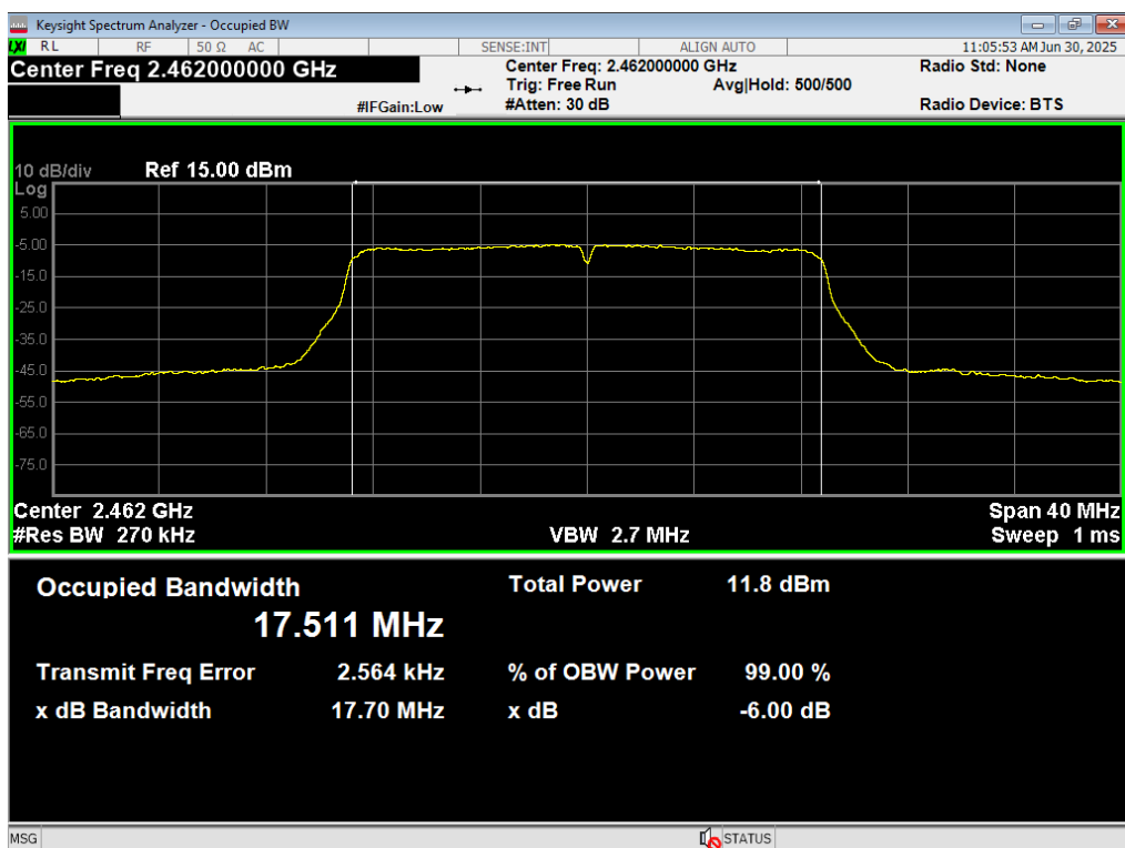
62 Occupied BW, WiFi N 6.5MB, 2462MHz
