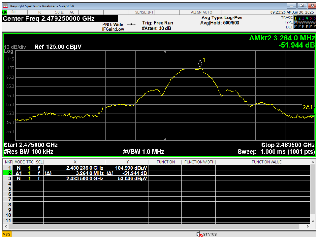
05 HBE Unrestricted, ANT GFSK, 2480MHz
