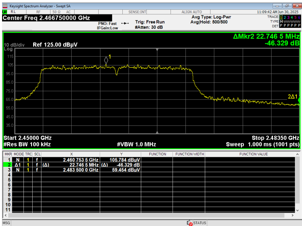
70 HBE Unrestricted, WiFi N 72.2MB, 2462MHz
