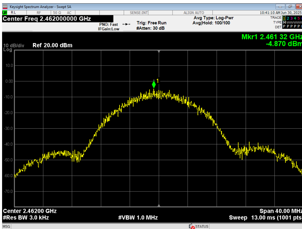
26 PSD, WiFi B 11MB, 2462MHz
