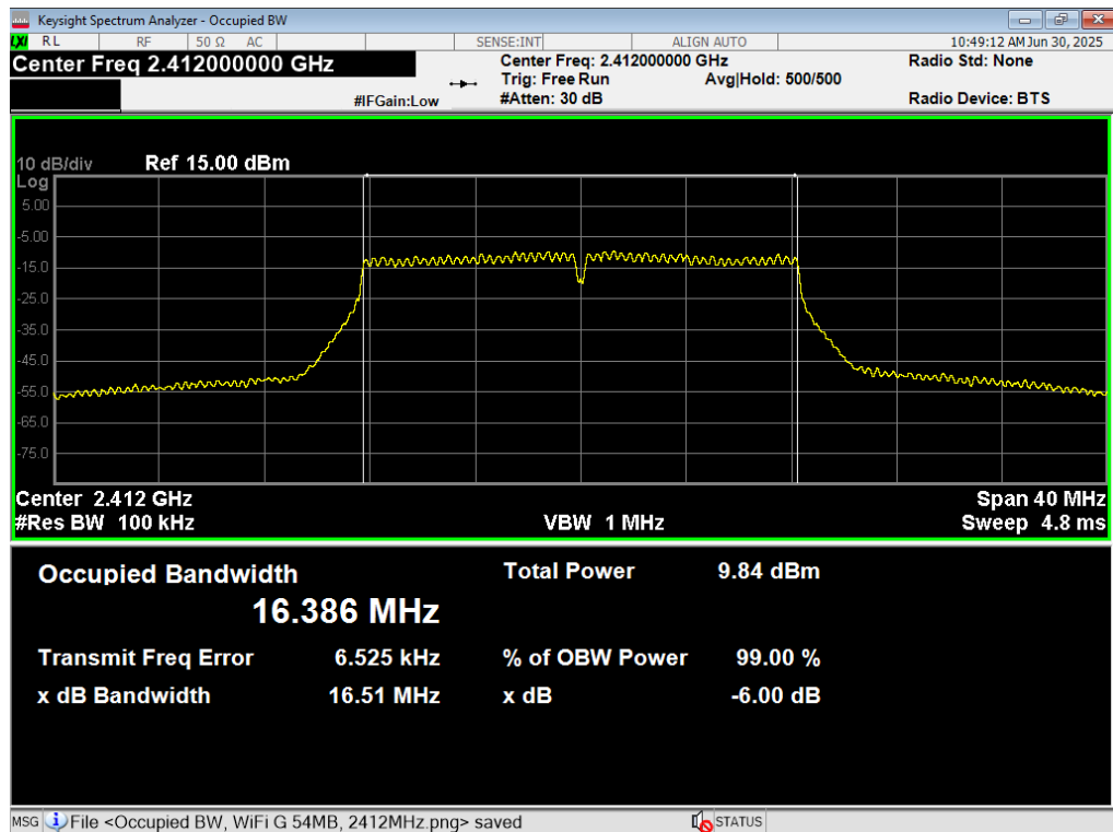
40 6dB BW, WiFi G 54MB, 2412MHz
