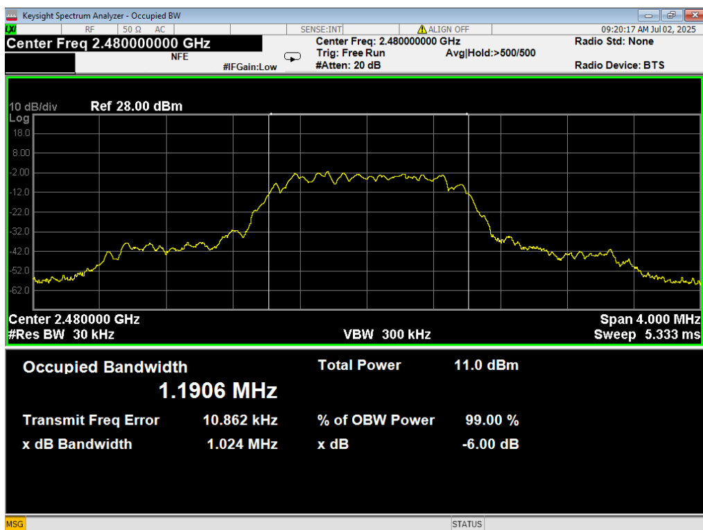
10 Occupied BW, 2EDR, 2480MHz
