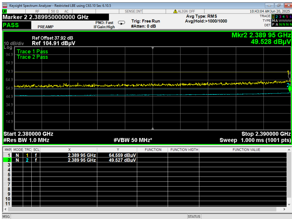
45 LBE Restricted, WiFi G 54MB, ch1 2412MHz
