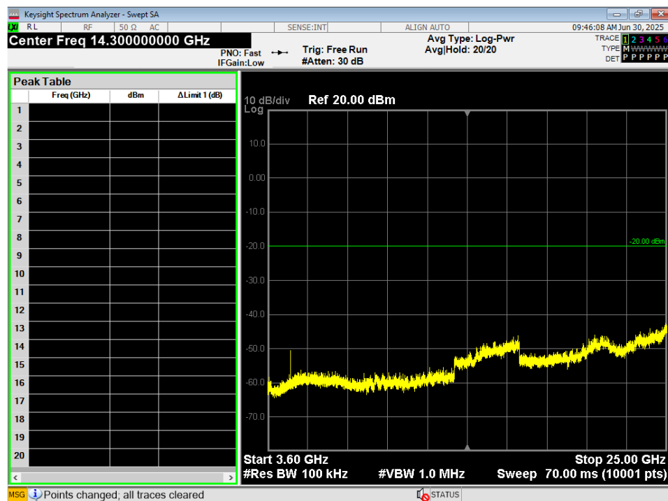
Figure 20 - Conducted Spurious Plot, GMSK 2MB, 3.6GHz – 25GHz, Low
