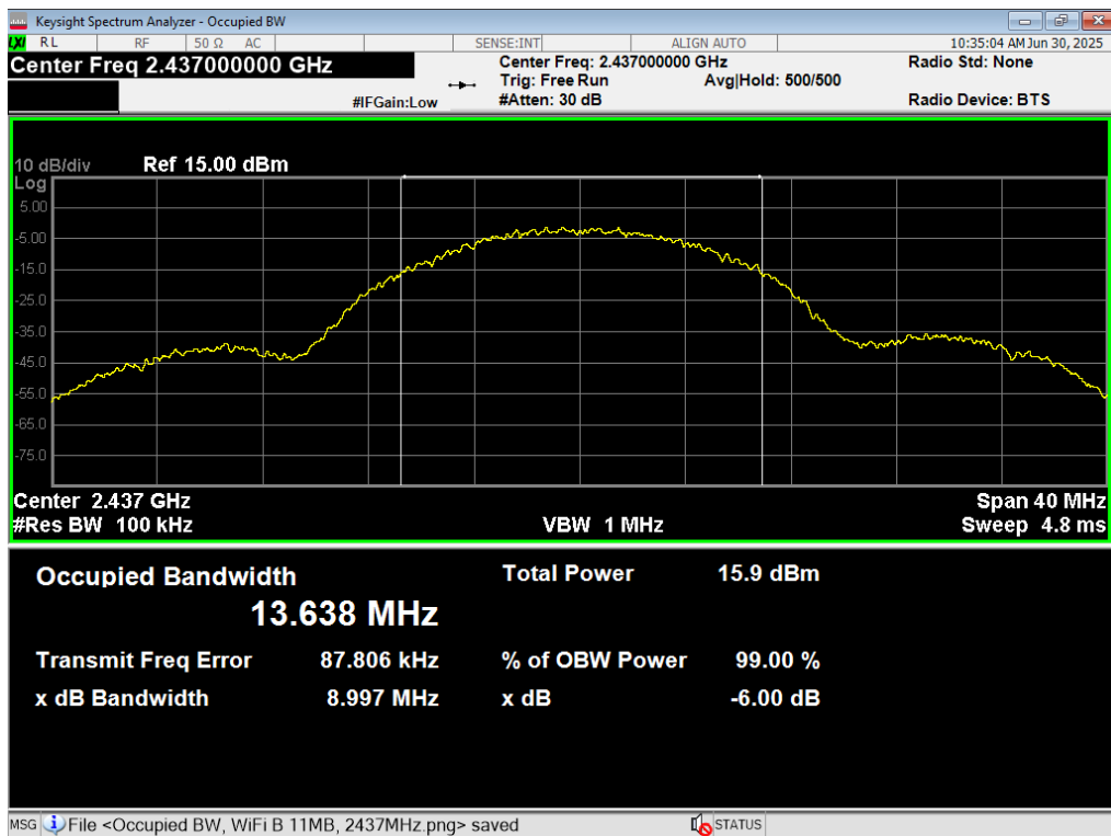
15 6dB BW, WiFi B 11MB, 2437MHz
