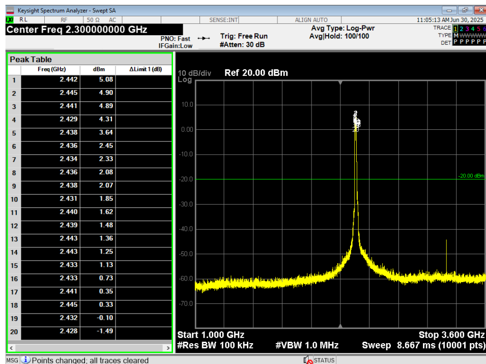
Figure 28 - Conducted Spurious Plot, WIFI 802.11n, 1G – 3.6G, Mid
