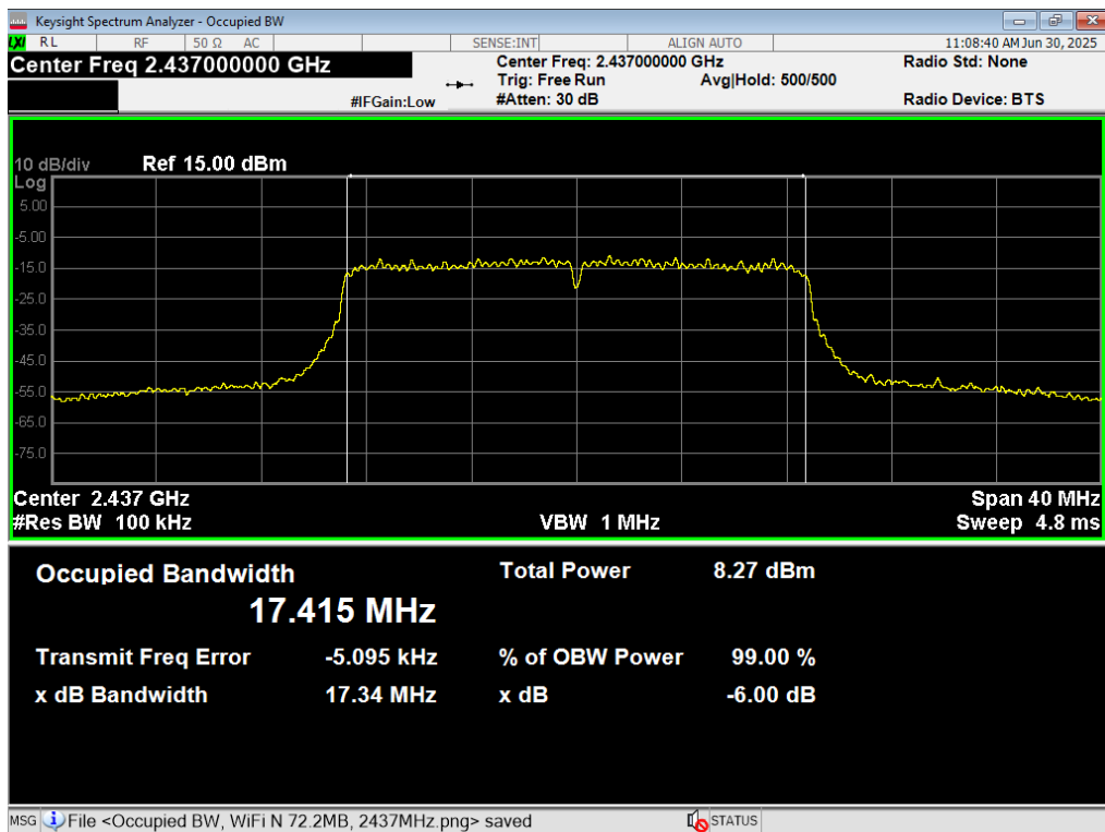
67 6dB BW, WiFi N 72.2MB, 2437MHz
