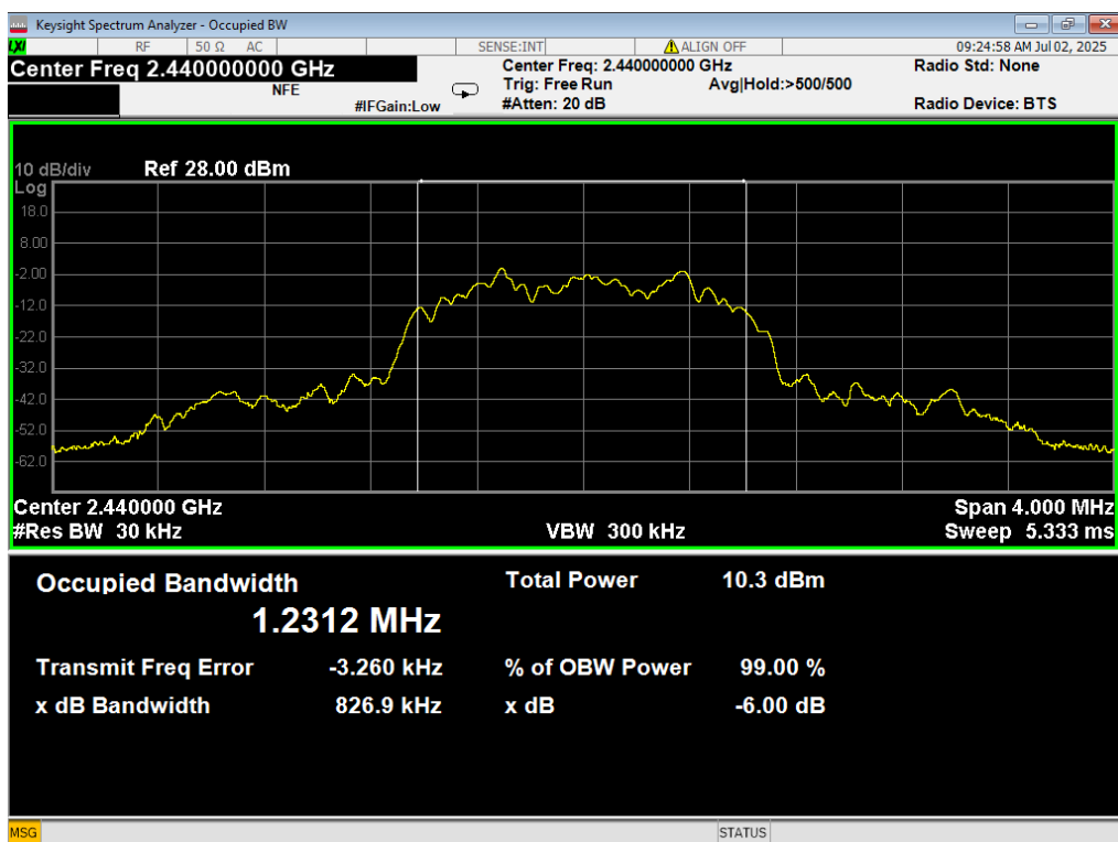
22 Occupied BW, 3EDR, 2440MHz
