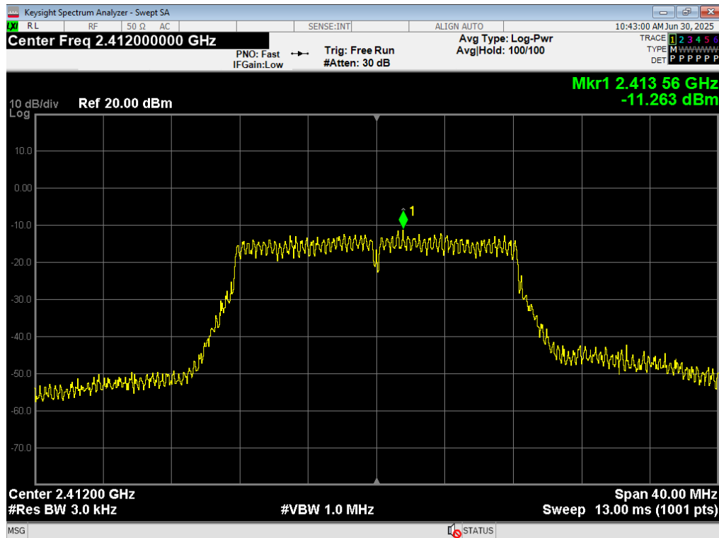
37 PSD, WiFi G 6MB, 2412MHz
