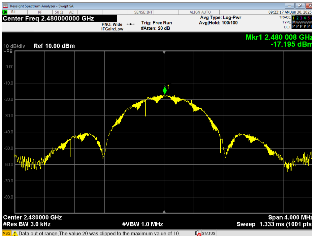
13 PSD, ANT GFSK, 2480MHz
