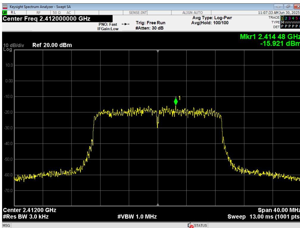
76 PSD, WiFi N 72.2MB, 2412MHz
