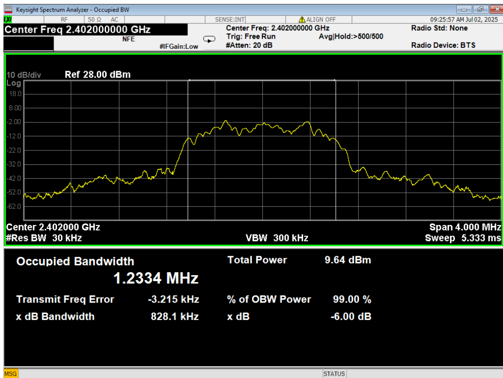
21 Occupied BW, 3EDR, 2402MHz
