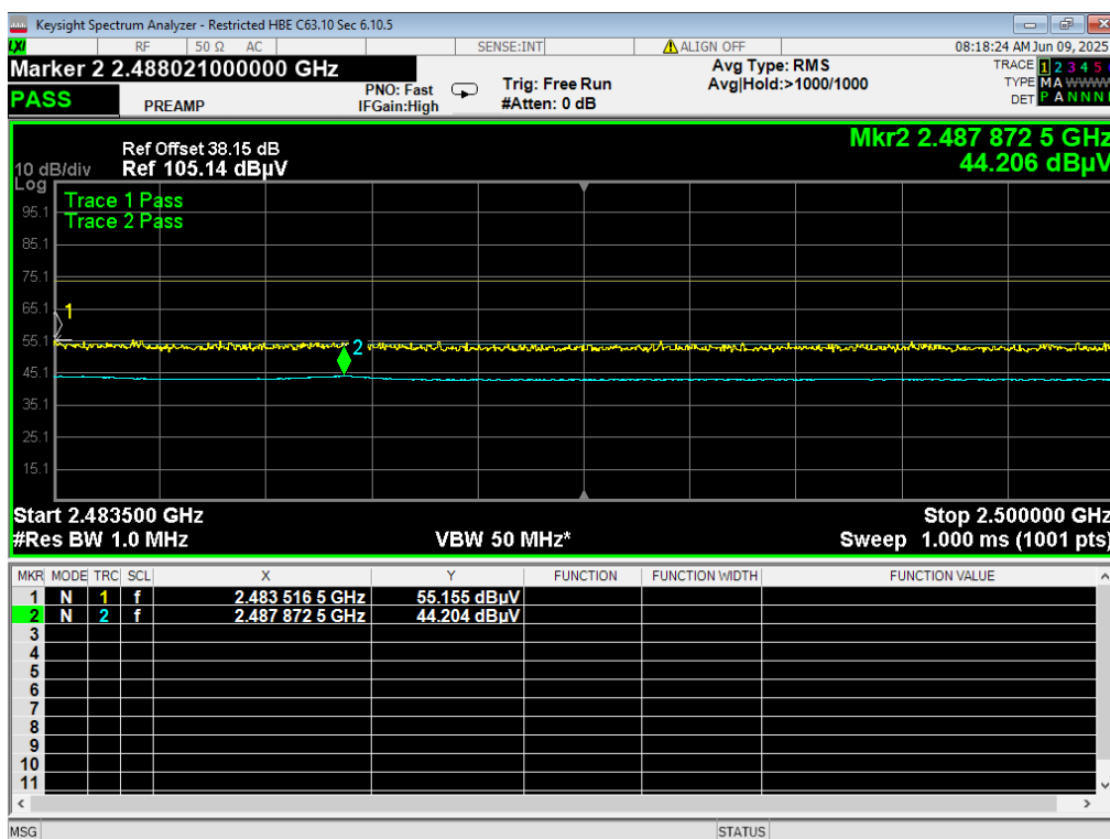
04 HBE Restricted, ANT GFSK, 2480MHz
