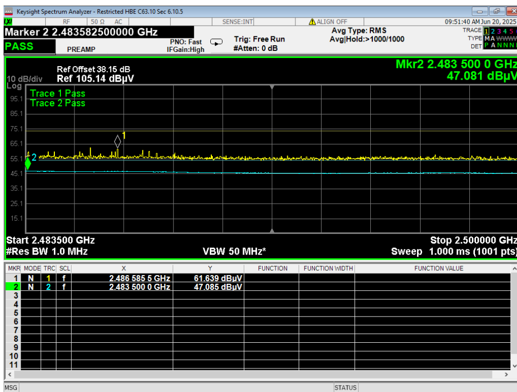
04 HBE Restricted, WiFi B 1MB, ch11 2462MHz, pwr42
