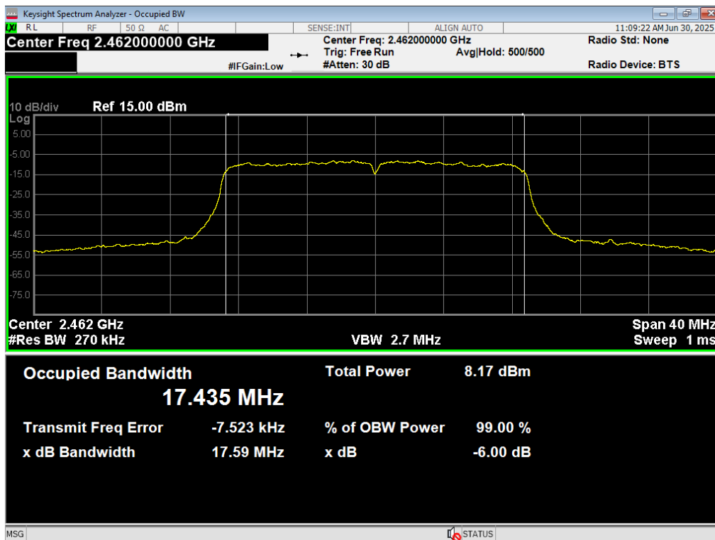
75 Occupied BW, WiFi N 72.2MB, 2462MHz
