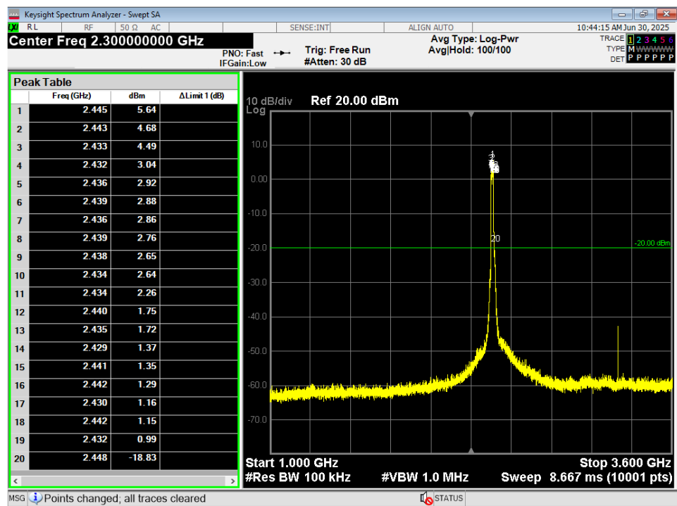
Figure 25 - Conducted Spurious Plot, WIFI 802.11g, 1G – 3.6G, Mid
