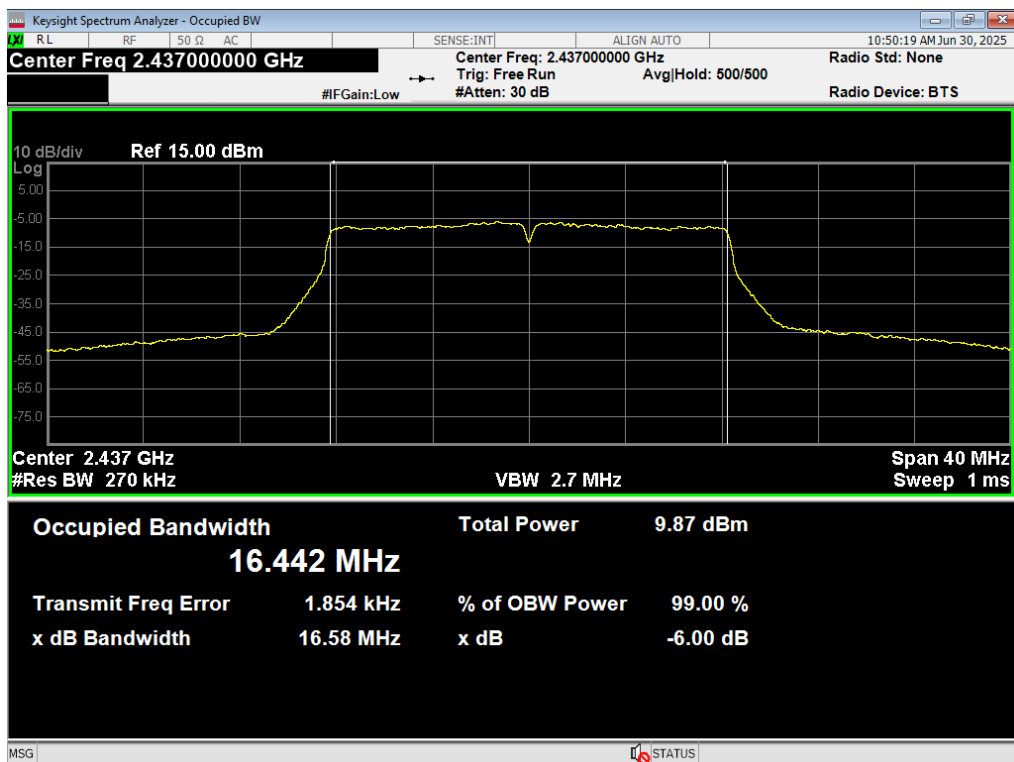
48 Occupied BW, WiFi G 54MB, 2437MHz
