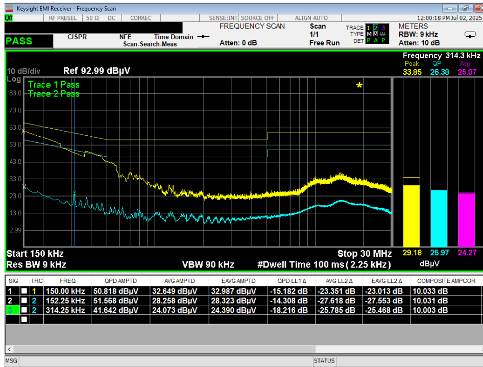
Figure 14 – Conducted Emissions Plot, charging on dock, TX, Line
