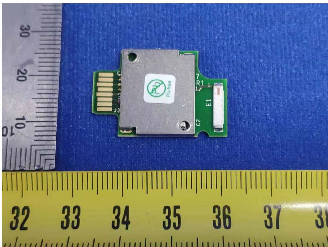
FIGURE 14 BATTERY ANALYZER (M/N: BT521) RF MODULE (SOLDERED SIDE)
