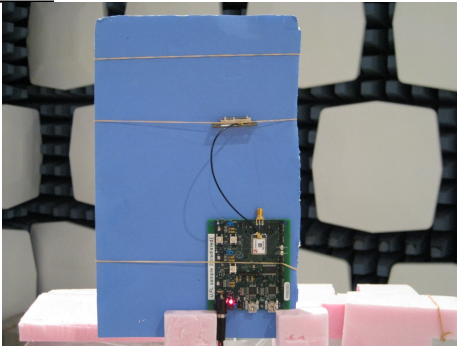
Radio module shown on host board with PIFA antenna
