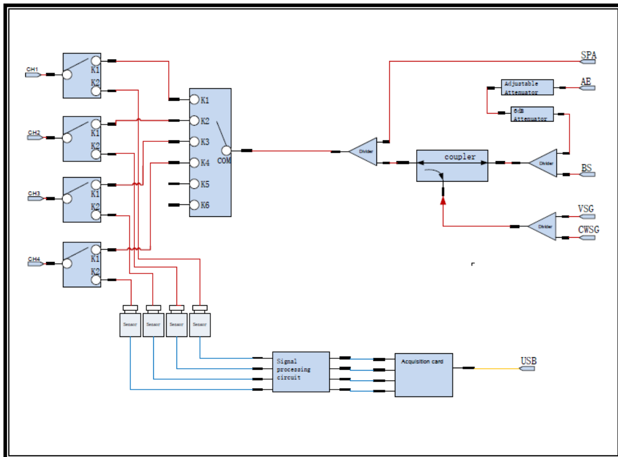
Tonscend SRD Test System
