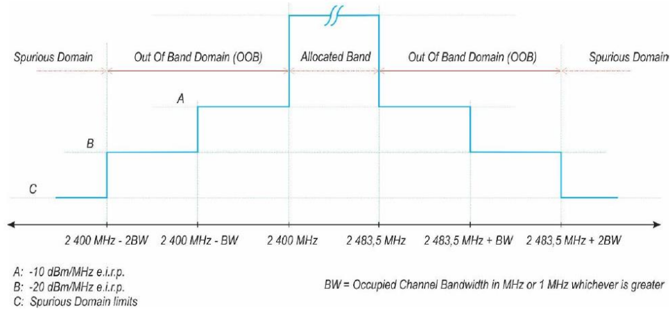
Figure 1: Transmit mask
