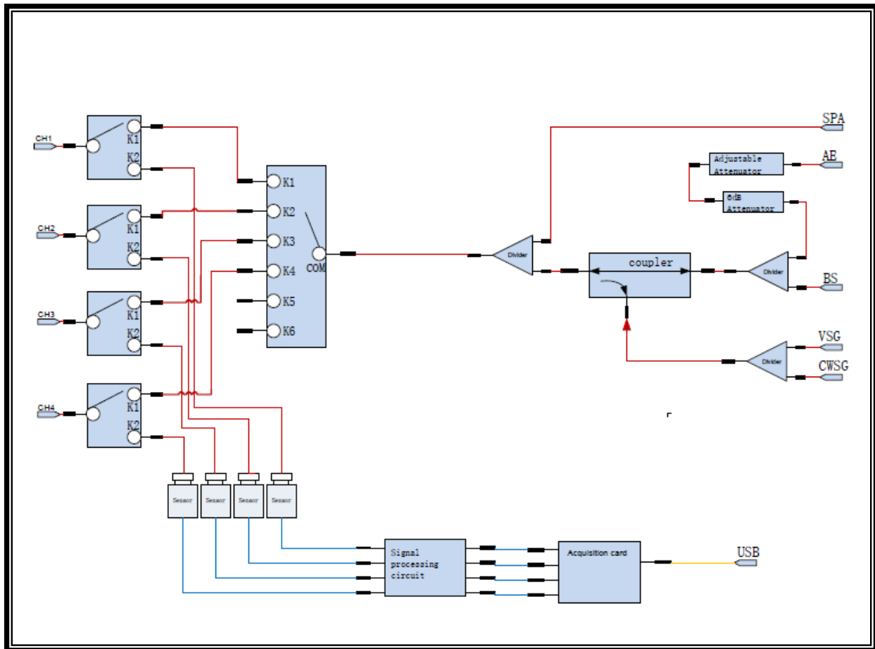
Tonsend SRD Test System
