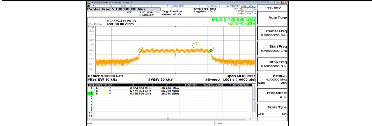
HTNV 11AC20SISO Ant1 5180
