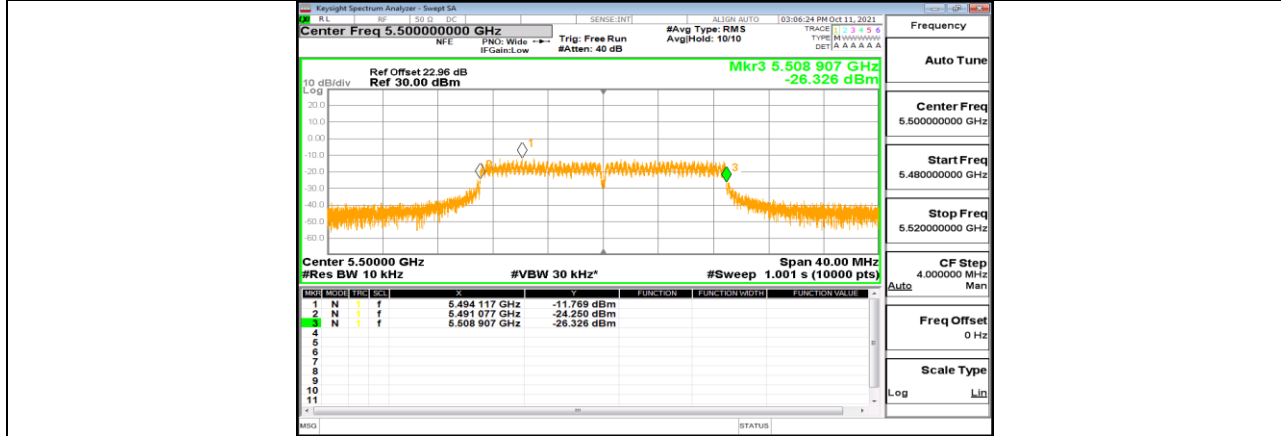
HTNV 11AC20SISO Ant1 5500
