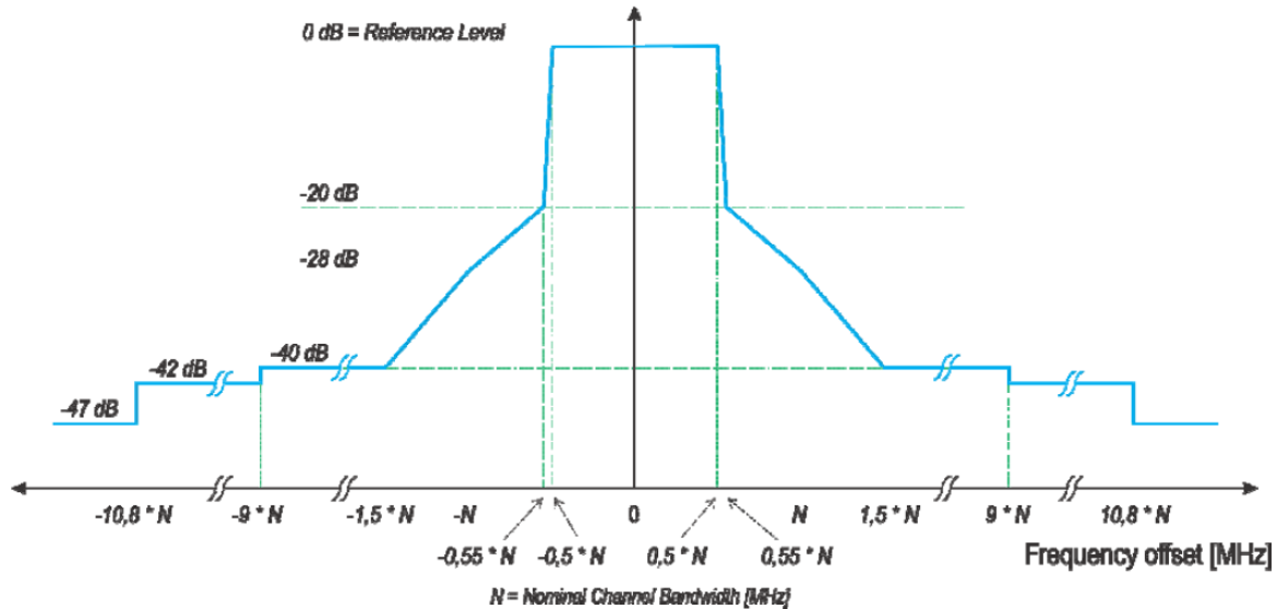
Figure 1: Transmit spectral power mask
