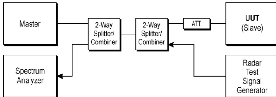
Figure 6: Set-up B
