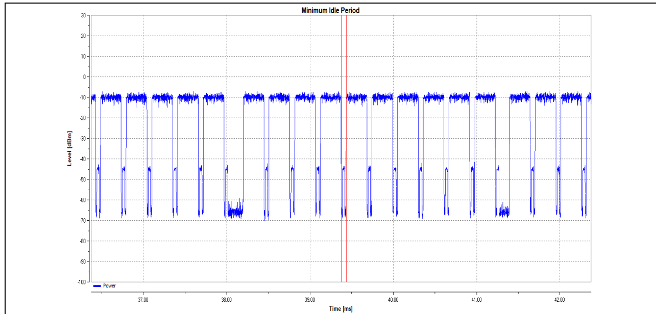
11N20MIMO Ant2 5180
