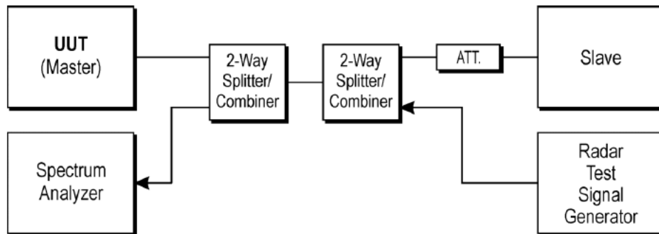
Figure 5: Set-up A
