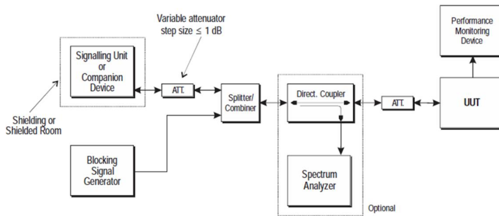
Figure 18: Test Set-up for receiver blocking
