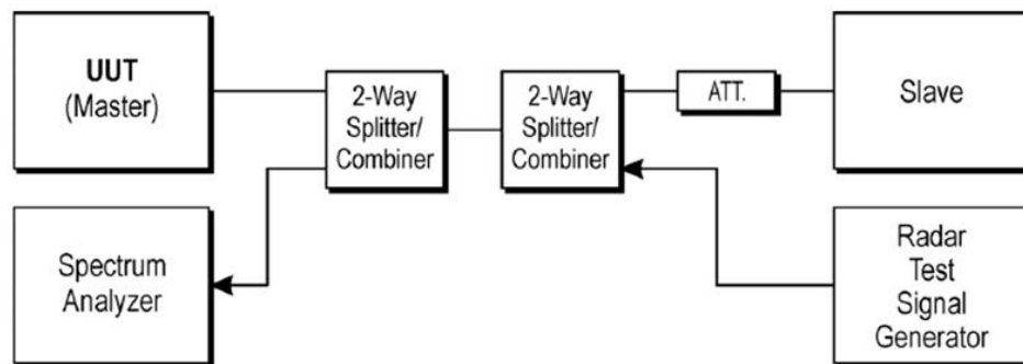
Figure 5: Set-up A
