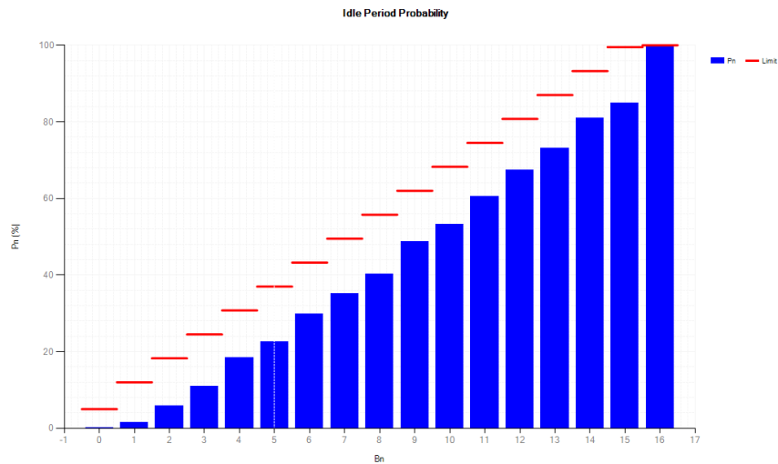
Idle Period Probability NVNT n40 5190MHz
