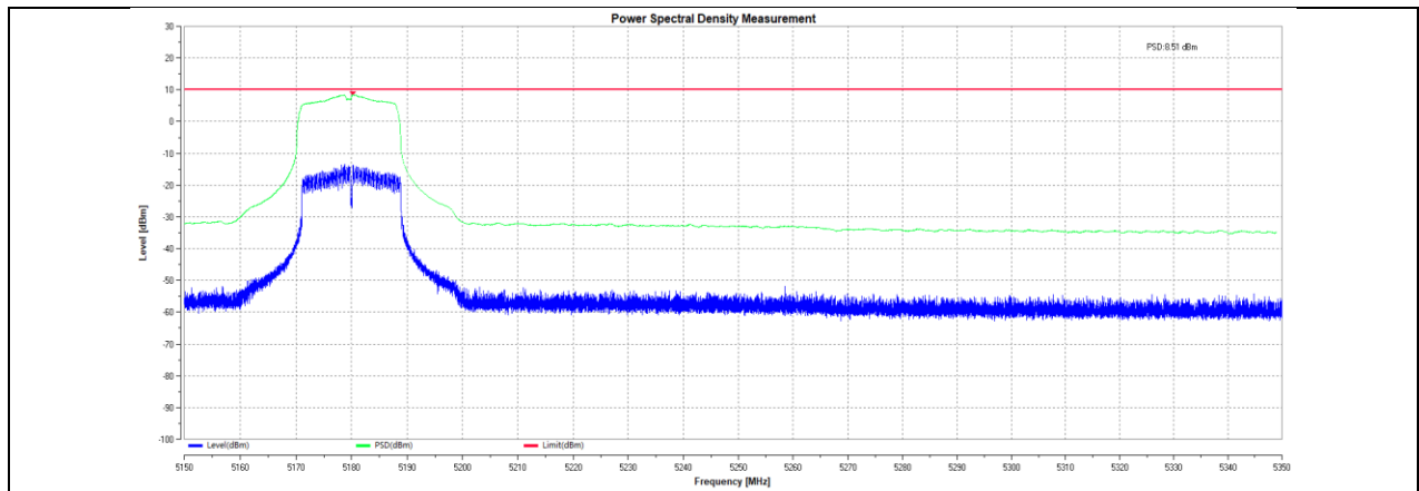
11N20MIMO total 5180
