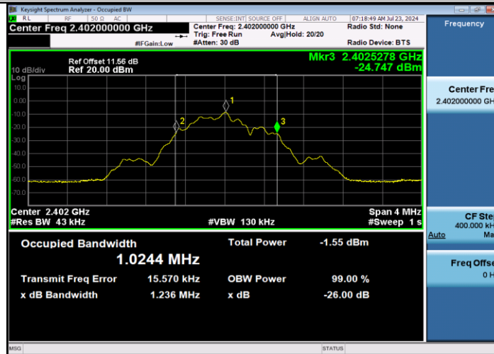
BLE_1M_Ant1_2440
