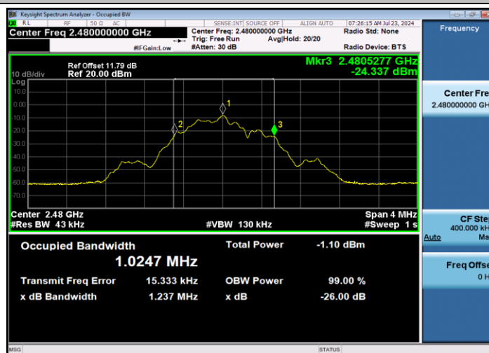
BLE_1M_Ant1_2480
