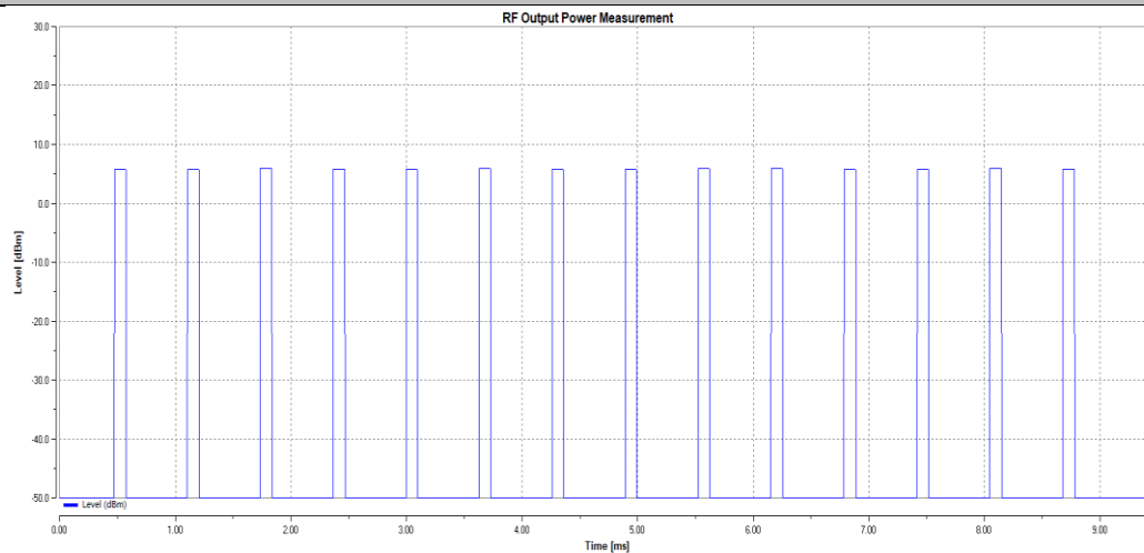
NTNV_BLE_1M_Ant1_2480
