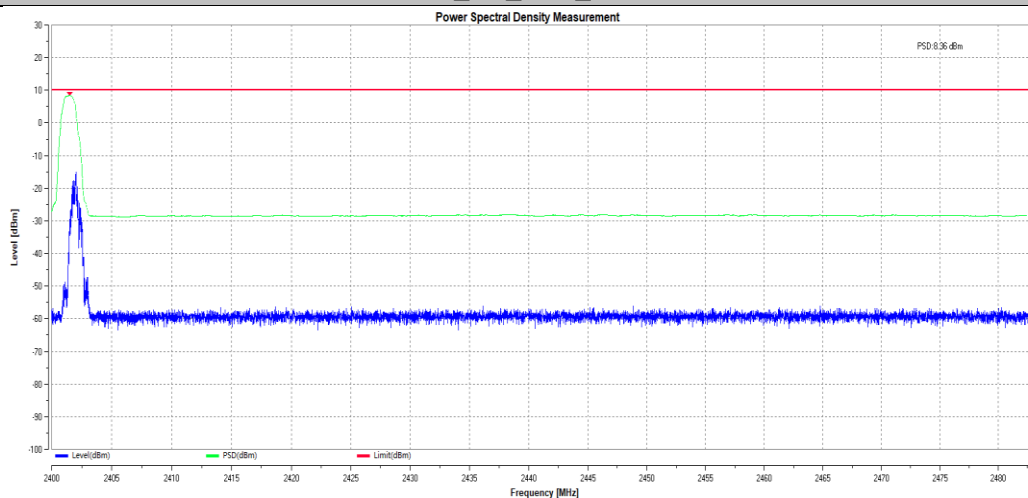
BLE_1M_Ant1_2440
