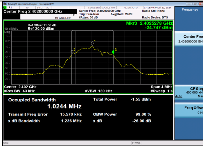
BLE_1M_Ant1_2440
