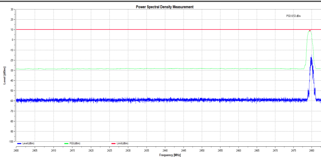
BLE_1M_Ant1_2480
