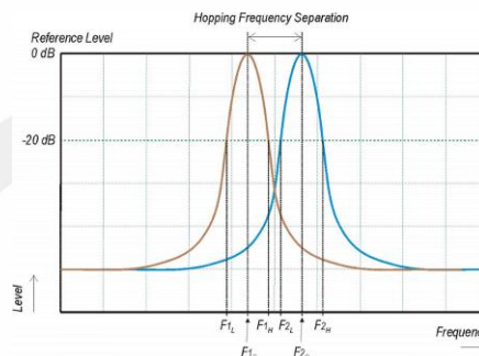
Figure 4: Hopping Frequency Separation
