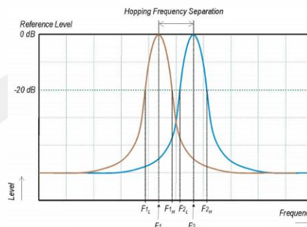
Figure 4: Hopping Frequency Separation
