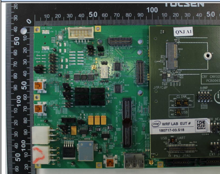
Extender board
